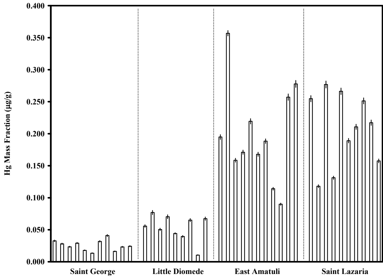
Figure 12. Mass fraction value ( \mu\text{g/g} ) and expanded uncertainty for each individual mercury wet mass fraction determination.
