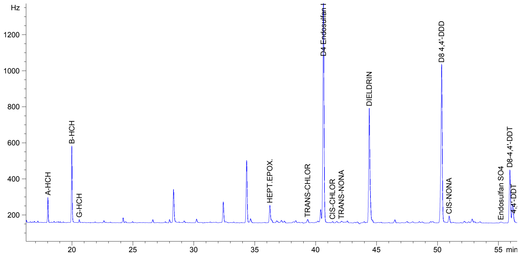
Figure 5. Representative F2 chromatogram of a murre egg from the DB-5 column.
