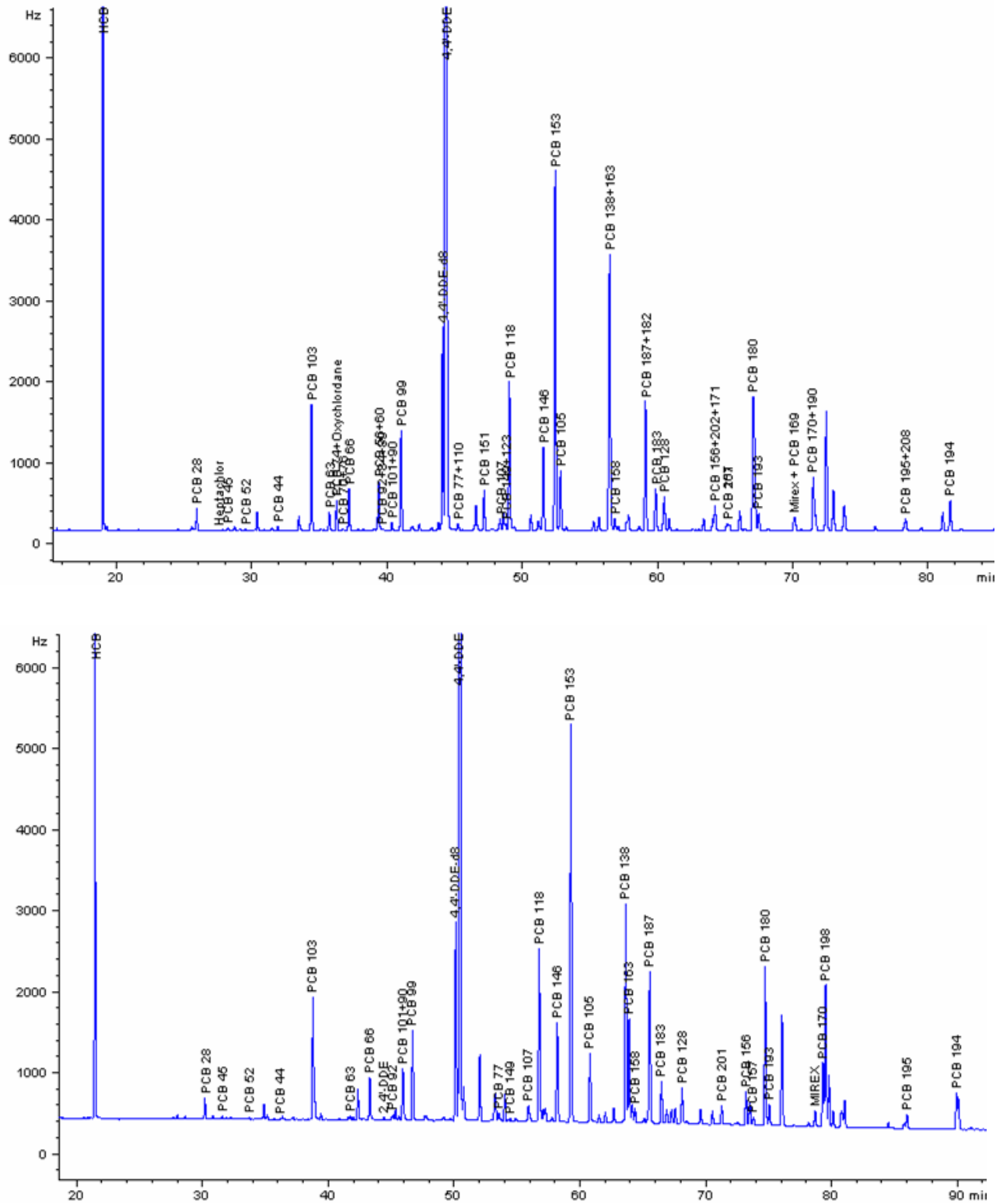
Figure 4. Representative F1 chromatograms of a murre egg. The top chromatogram is from the DB-5 column and the bottom chromatogram is the DB-XLB column. .
