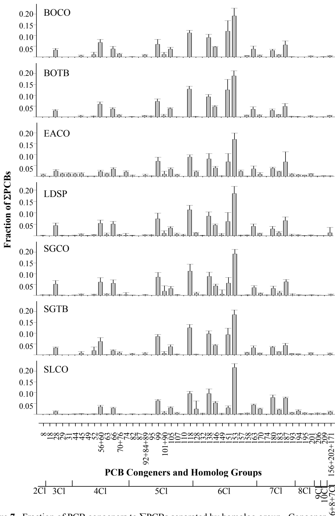
Figure 7. Fraction of PCB congeners to \Sigma PCBs separated by homolog group. Congener numbers based on IUPAC system. Abbreviations are the same as in Figure 6.
