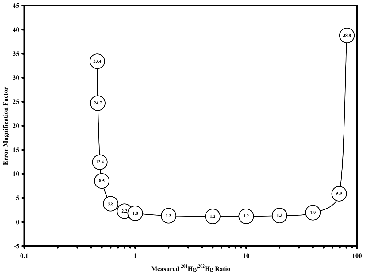
Figure 9. Error magnification factor as a function of measured ^{201}\text{Hg}/^{202}\text{Hg} ratio.
