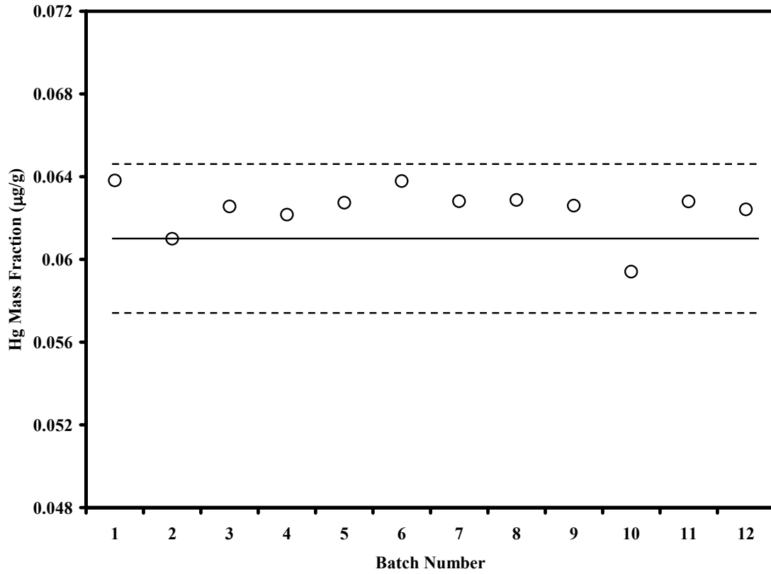
Figure 11. Control chart for mercury mass fraction ( \mu\text{g/g} ) in SRM 2976 Mussel Tissue (Trace Elements and Methylmercury), total mercury certified value = 0.0610 \mu\text{g/g} \pm 0.0036 \mu\text{g/g} .
