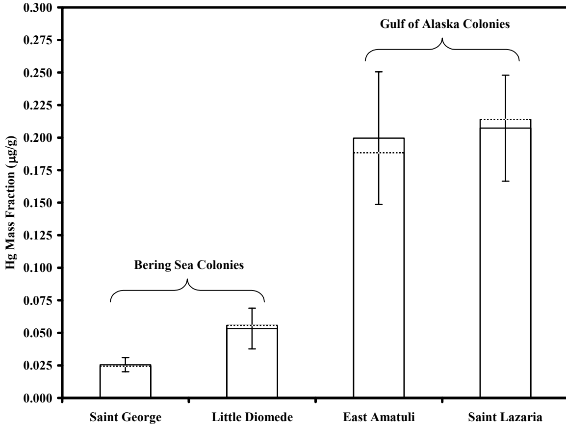
Figure 13. Mercury mass fraction data: mean \pm 95% confidence interval and median (dashed line) plotted as a function of island location.
