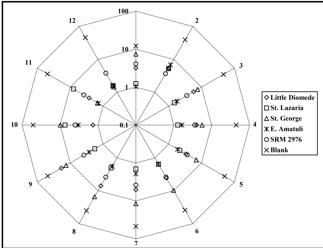
Figure 10. Radar plot showing all measured ^{201}\text{Hg}/^{202}\text{Hg} isotope dilution ratios (log axis) for each sample batch.
