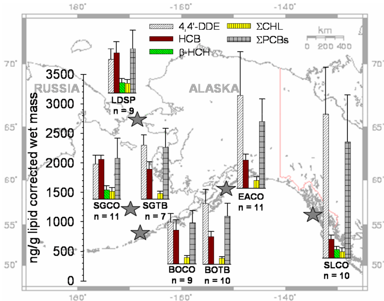
Figure 6. Concentrations (mean bars with 1 standard deviation error lines) of major persistent organic pollutants in eggs collected at murre ( Uria spp.) colonies in 1999 and 2000. BO = Bogoslof Island, EA = East Amatuli Island, LD = Little Diomedede Island, SG = St. George Island, and SL = St. Lazaria Island. CO = common murre eggs, TB = thick-billed murre eggs, and SP = murre species eggs.
