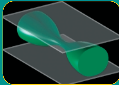
Lattice Boltzmann simulation of breakup of a fluid thread confined between parallel plates.
