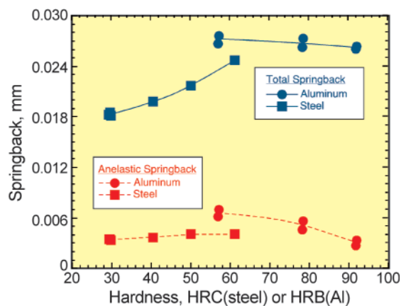
Figure 1: The total springback and anelastic (non-linear) contribution in Rockwell hardness tests.
