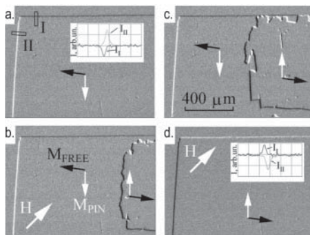
Figure 1: MOIF image of the remagnetization process of a Co/Ru/Co homogeneous structure containing pinholes in the Ru in a field oriented along the total magnetization vector. (a) H = 0 mT after magnetization in a field of +60 mT; (b) H = -9.4 mT; (c) H = -9.4 mT after a 5 sec. wait; (d) H = -13.0 mT. The inserts in (a) and (d) show the intensity change of the MO signal.
