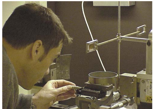
Figure 1: Residual stress measurement in Demeri cup at Advanced Photon Source.
