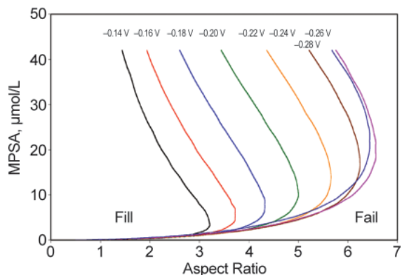
Figure 2: Feature fill/fail boundaries as a function of processing parameters: catalyst concentration, etc.
