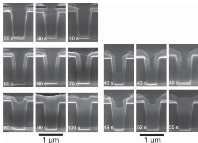
Figure 1: Superconformal filling of vias during silver (left) and copper (right) electrodeposition (NIST Metallurgy Division, using patterned wafers from International SeMaTech).
