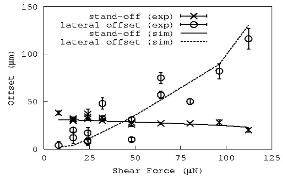
Figure 1. Measured lateral offset (misalignment) and normal offset (standoff height) for \approx 0.0023 \text{ mm}^3 \text{ Pb}_{63}\text{Sn}_{37} solder connecting 0.35 \text{ mm} diameter pads as functions of applied shear force. The curves are predictions of Surface Evolver.
