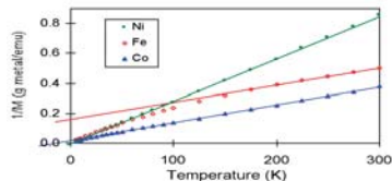
Figure 1. 1/M vs T for Ni, Fe-, and Co-containing dendrimers exhibiting straight line fits at high temperatures (Curie-Weiss behavior) with small deviations at low temperatures, particularly in the case of Fe.
