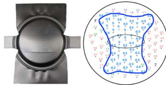
Figure 2. NIST plane-strain geometry and uniformity plot.
