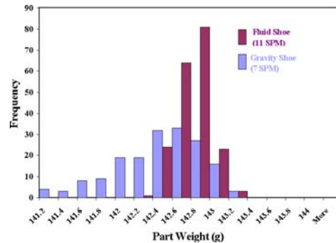
Figure 5. Weight distribution for gears made with and without the fluidized feedshoe technology.
