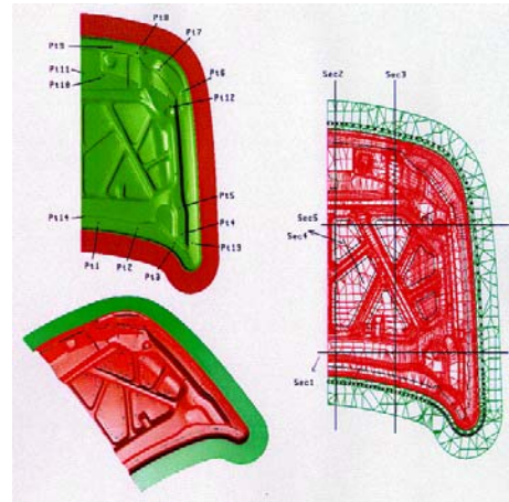
Figure 2. The inner panel of a car hood was one of the components targeted by industry for in-depth investigation of its springback behavior.
