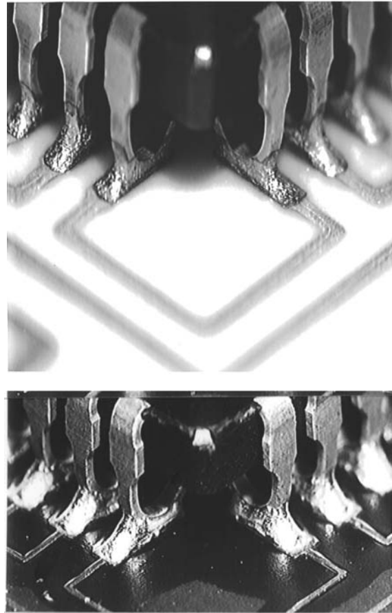
Figure 1. Plastic leaded chip carriers on ceramic (top) and polymeric (bottom) substrates assembled with Pb-free solders and surface finishes.
