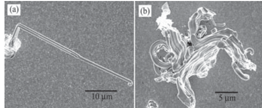
Figure 1. Defects include both (a) whiskers and (b) eruptions.
