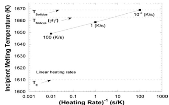
Figure 1. Calculated incipient melting temperature as a function of linear heating rates for Ni-0.045Ta-0.12Al mole fraction alloy solidified assuming a Scheil solidification. Local equilibrium distributions of \gamma' and \text{Ni}_3\text{Ta} are assumed.
