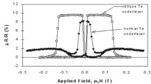
Figure 2. Magnetoresistance curves for two SAF-pinned spin valves deposited on oblique Ta and normally sputtered Ta underlayers. The obliquely deposited Ta underlayer stabilizes the SAF structure. The spin flop transition is visible as a bump in the normal Ta spin valve curve starting at 0.06 T.
