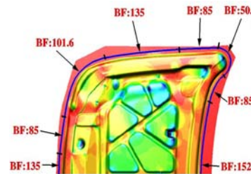
Figure 4. Inner panel of car hood.
