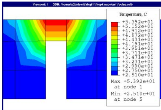
Figure 1. Temperature distribution due to heat pulse.
