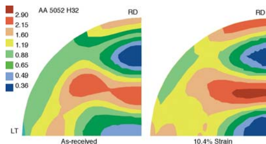
Figure 2. Influence of biaxial strain on (111) pole figure.
