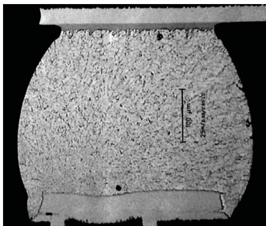
Figure 1. Metallographic cross-section of a lead-free SnAgCu solder selected under the NIST-led NEMI Pb-free Alloy Task Group. The chip-scale package shown here has been assembled with a SnPb component finish to determine how Pb contamination affects reliability.
