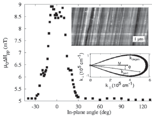
Figure 1. Ferromagnetic resonance linewidth in a 64 nm film of \text{Ni}_{80}\text{Fe}_{20} as a function of magnetization direction relative to parallel scratches in the substrate (top inset). M is perpendicular to the scratches at 0^\circ . The scratches contribute to linewidth only when perturbation wavevectors coincide with wavevectors of degenerate spinwave modes (bottom inset).
