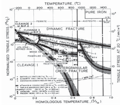
Figure 1. Fracture Mechanism Map for Pure Iron
