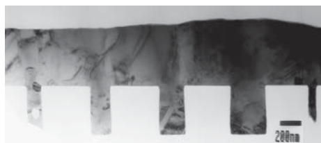
Figure 2. TEM image of copper electrodeposited nanoscale features in isuperfilled trenches. The electrodeposited copper contained microstructural defects such as voids, dislocations and twins that could not be revealed in the focused ion beam imaging.
