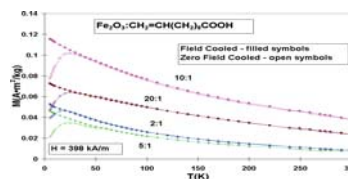
Figure 2. Magnetization behavior as a function of temperature for \gamma - Fe_2O_3 suspensions in carboxylic acid, with concentrations as labeled.
