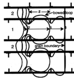
Figure 2. Schematic of model detailing progression of dislocation bows through the structure in TEM micrograph (from Peter Anderson, OSU).
