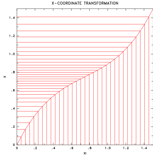
FIGURE 17: Polynomial Transformation.
