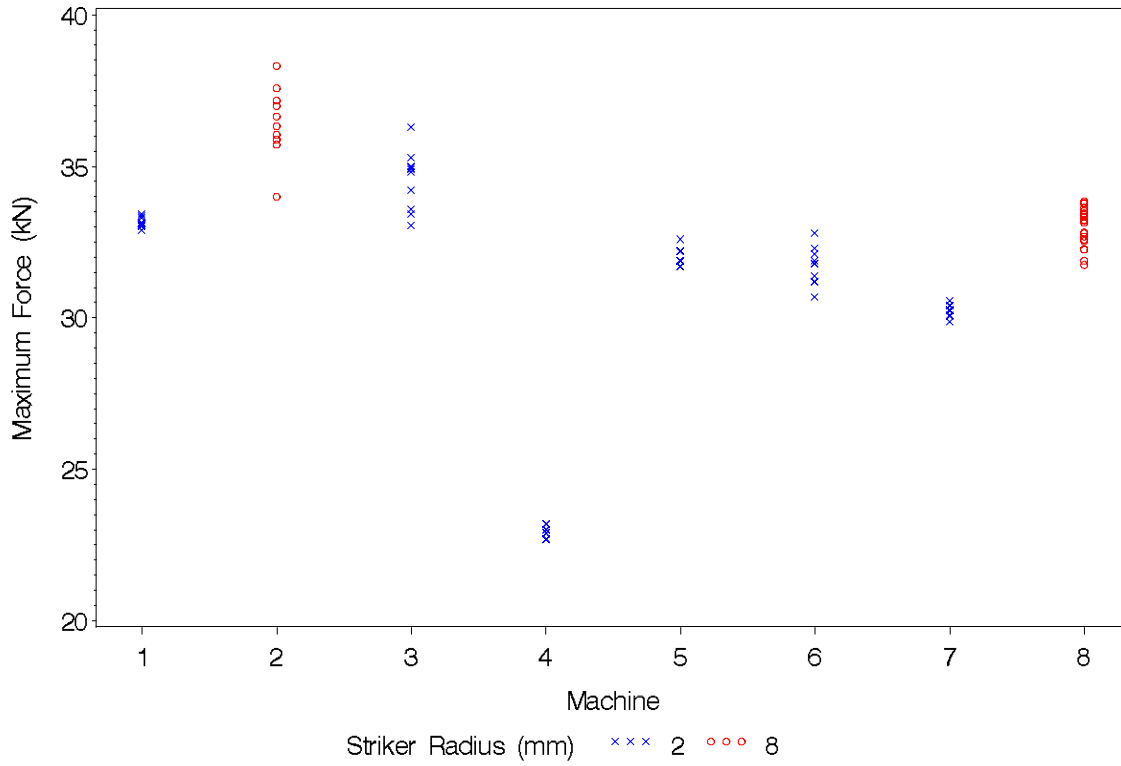
Figure 1. Low-energy maximum force for eight machines.
