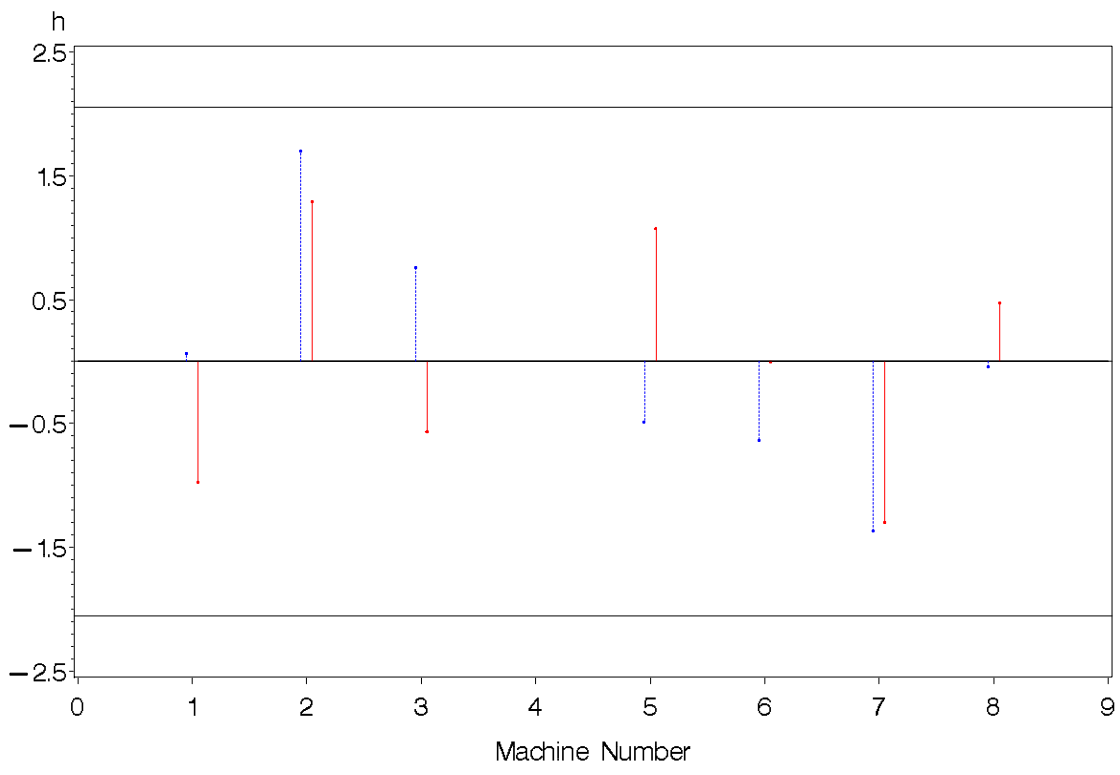
Figure 15. Between-laboratory consistency h statistics for seven Charpy machines. The dashed blue lines (left) correspond to the low energy data and the solid red lines (right) represent high energy data.
