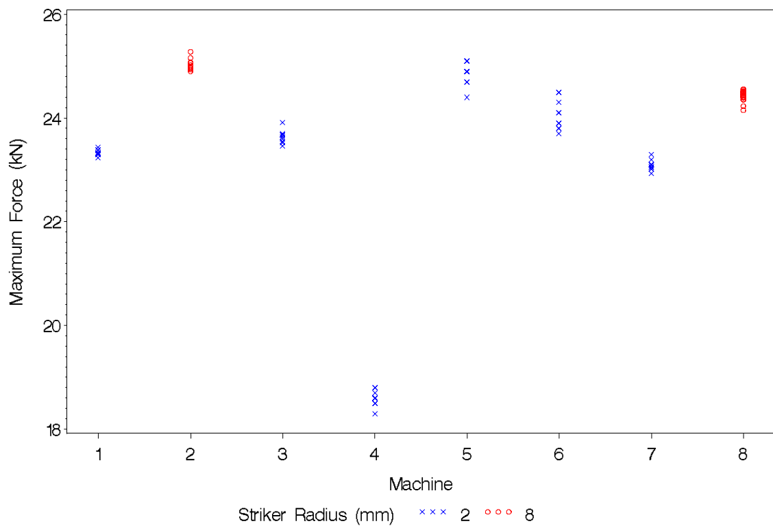
Figure 2. High-energy maximum force for eight machines.
