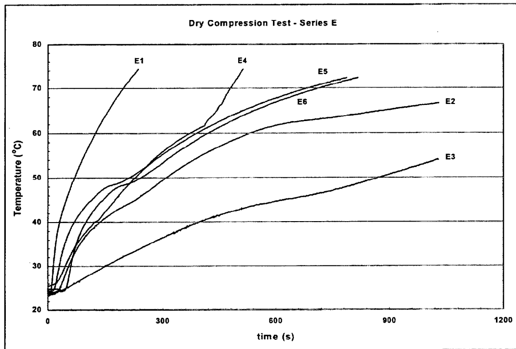
Figure 14 Dry compression test data for six different knee pad designs.
