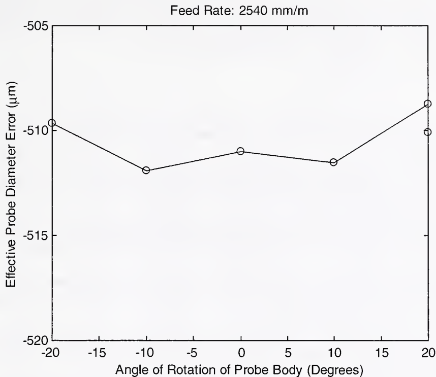
Figure 10. Display of Minimal Variation ( 2.5\mu\text{m} max error) Between Measurements at Various Angular Positions of Probe Body.
