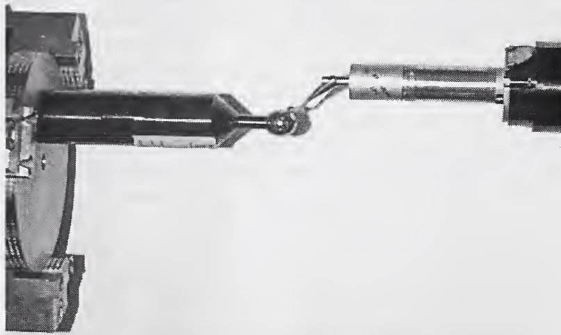
Figure 3. Fast probing of 0.75 in sphere.
