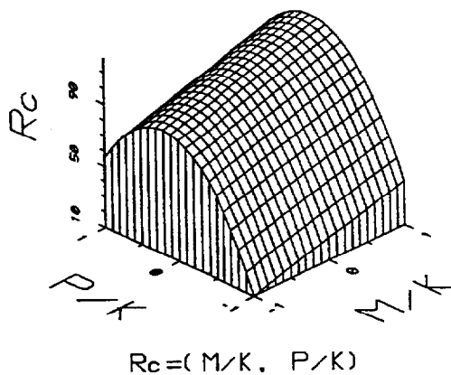
Figure 6.2: Epoxy concrete with the granite aggregate, showing the compressive strength ( R_c ) as a function of the material variables: K - aggregate, S - resin binder, M - microfiller, P - sand.
