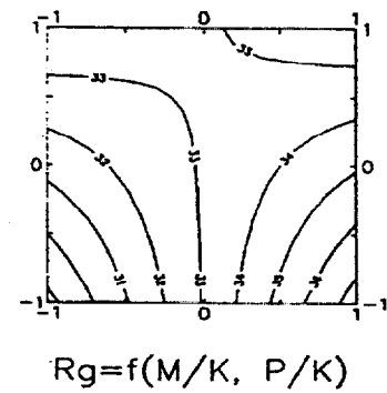
Figure 6.4: Epoxy concrete with the natural quartzite aggregate; flexural strength ( R_g ) as a function of the coded material variables; K - aggregate, S - resin binder, M - microfiller, P - sand
