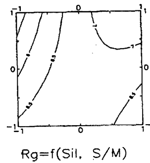
Figure 6.8: Highly-filled polyester concrete, showing the flexural strength ( R_g ) as a function of the material variables: K - aggregate, S - resin binder, M - microfiller, Sil - silane.
