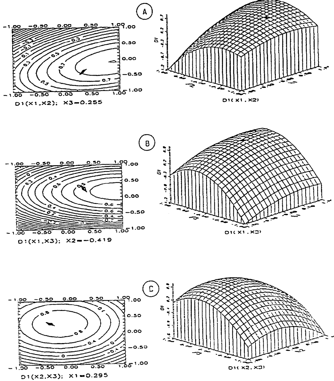
Figure 8.13: The overall desirability of the epoxy concrete in terms of low flammability and combustibility. Weight Set I. The top, middle, and bottom views are for cases where two different variables have been used for the coordinate axes.
