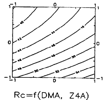
Figure 6.6: Polyester concrete, low temperature cure ( -10^{\circ}\text{C} ), showing the compressive strength ( R_c ) as a function of the material variables: NB - benzoyl peroxide, DMA - dimethylaniline, Z4A - aluminosilicate.
