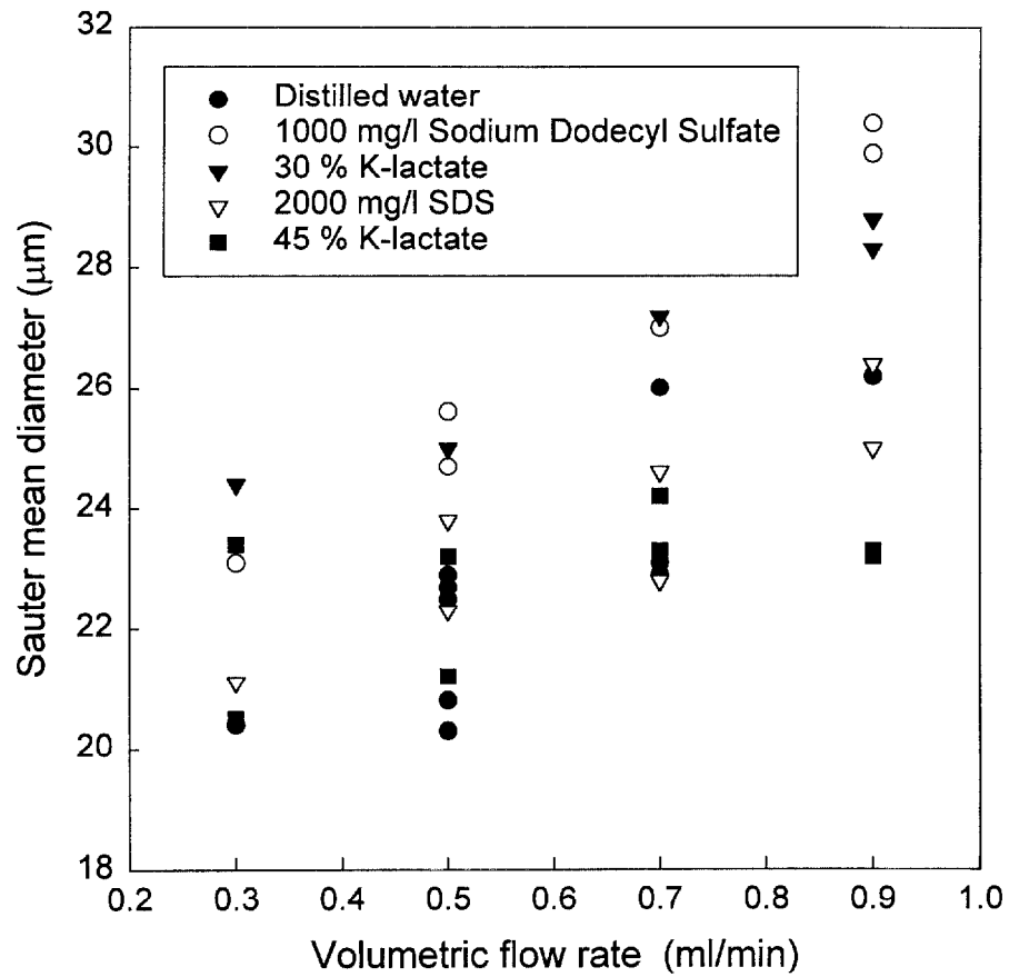
Figure 15. Droplet diameter measurements of various fluids using the PDPA at the centerline location, 2 cm downstream of the nebulizer exit.
