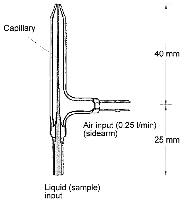
Figure 5. A schematic of the nebulizer.
