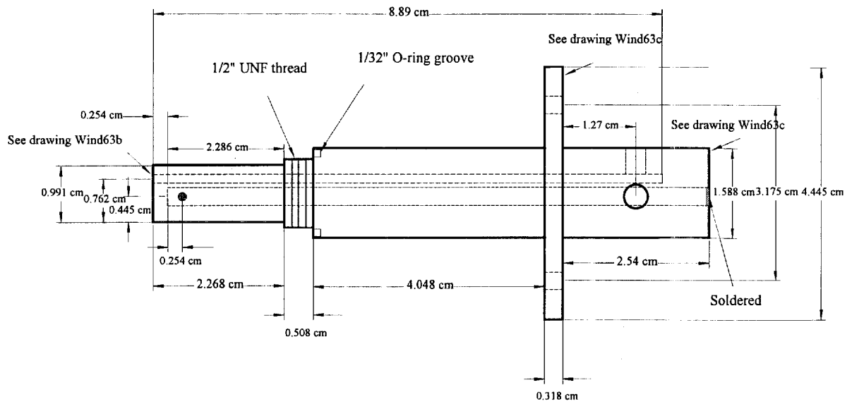
Burner insert (Brass)
