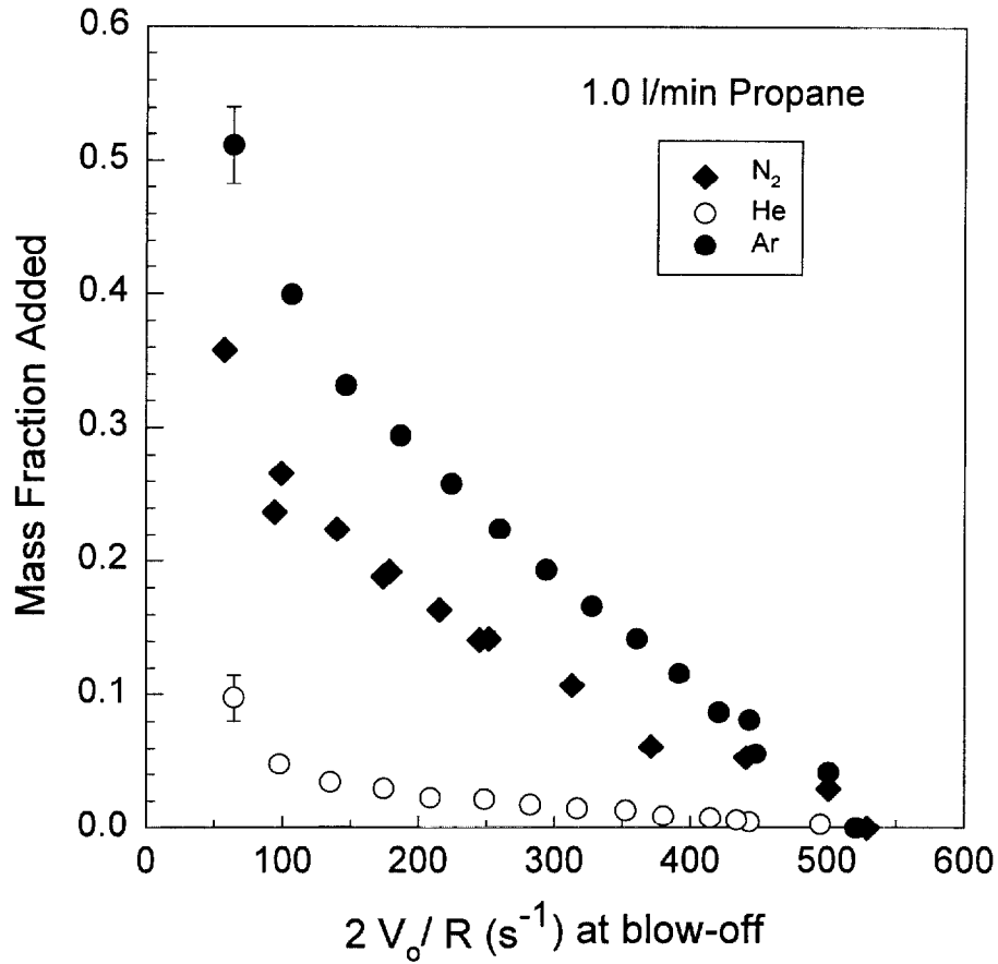
Figure 11. Mass fraction of inert gases added in air as a function of stagnation velocity gradient at blow-off.
