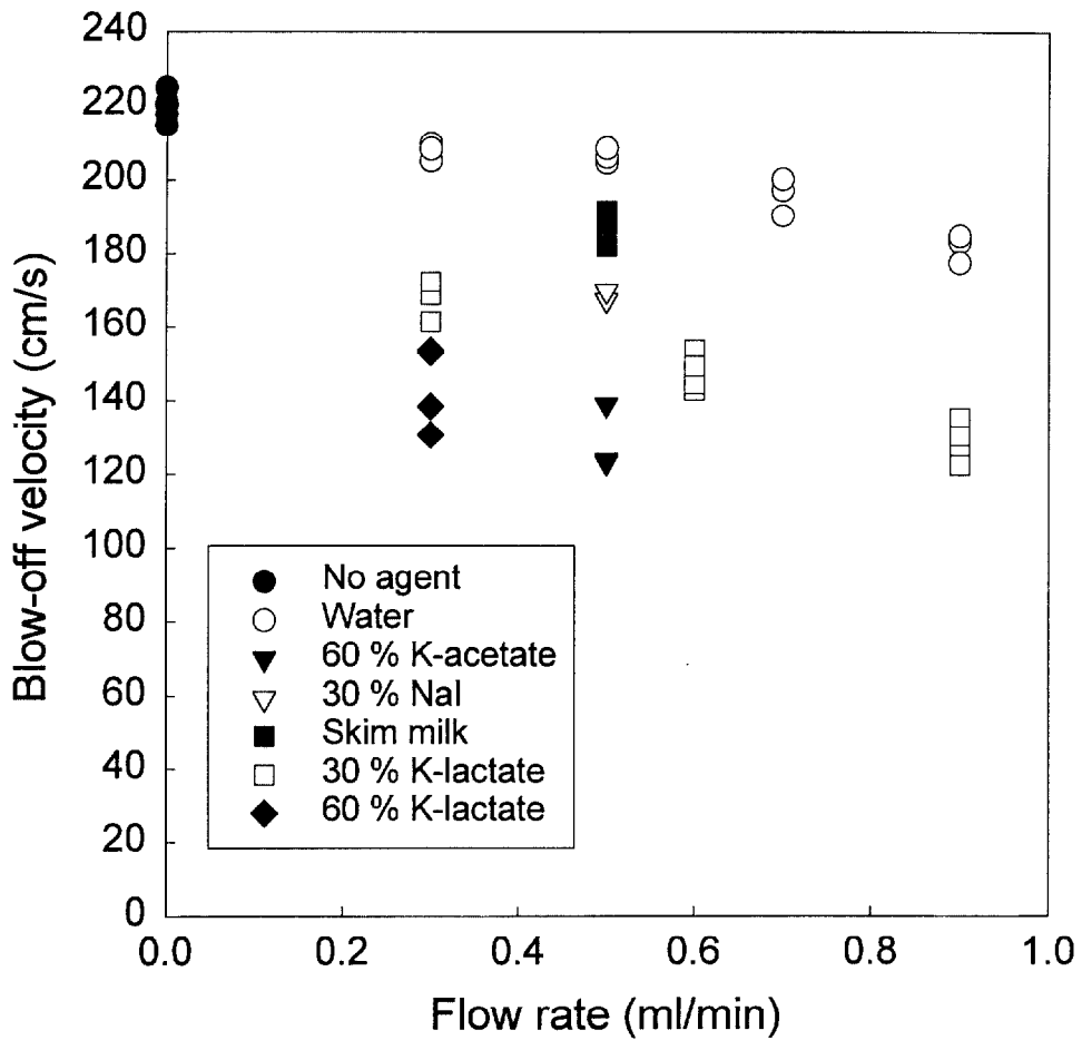
Figure 16. Screening results using different types of fluids.
