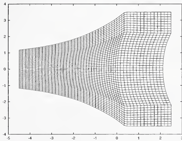
Figure 2: Contour mesh.
