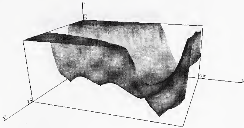
Figure 1: |\text{Bi}'(z)| , Modulus of the derivative of \text{Bi}(z) .
