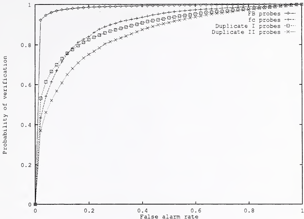
Fig. 6. Average performance of the algorithms on each probe category.
