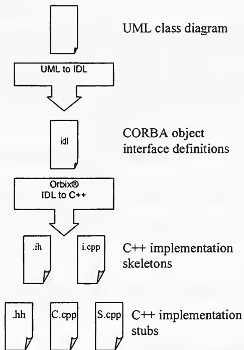
Figure 5: Files produced for wrapper development
