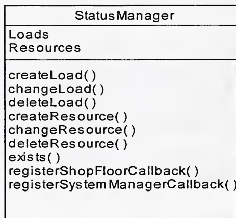
Figure 4: Richer Status Manager Class
