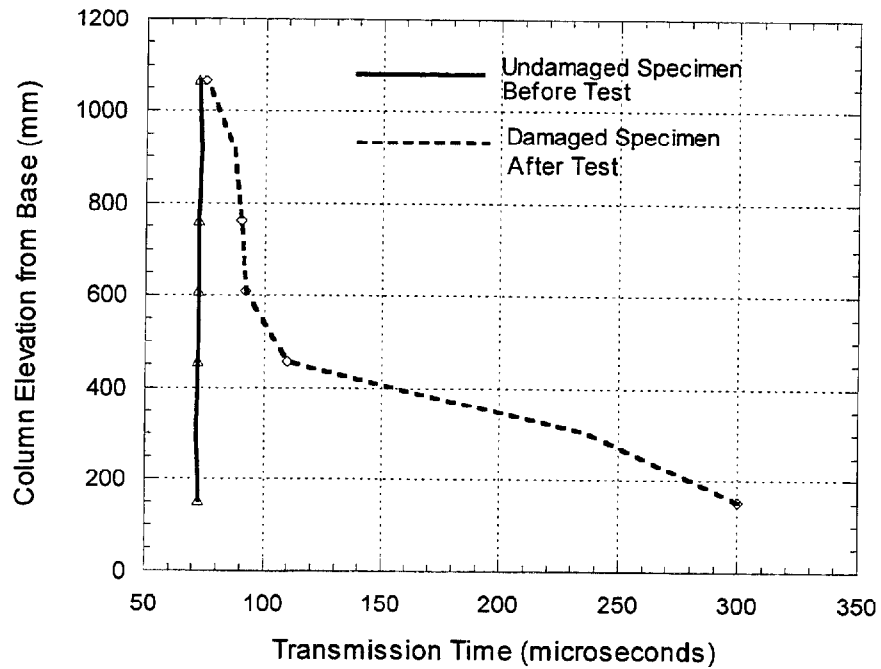
FIGURE A-3 Ultrasonic Readings Across Height of Specimen A6
