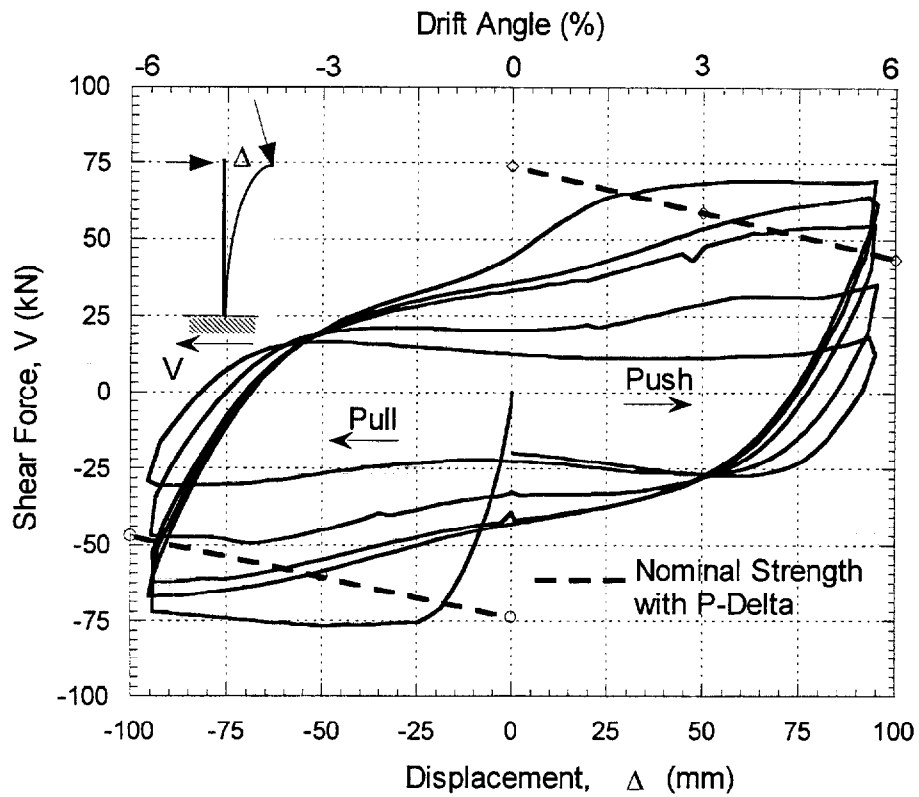
FIGURE 4-24 Shear vs. Displacement Response of Column A6
