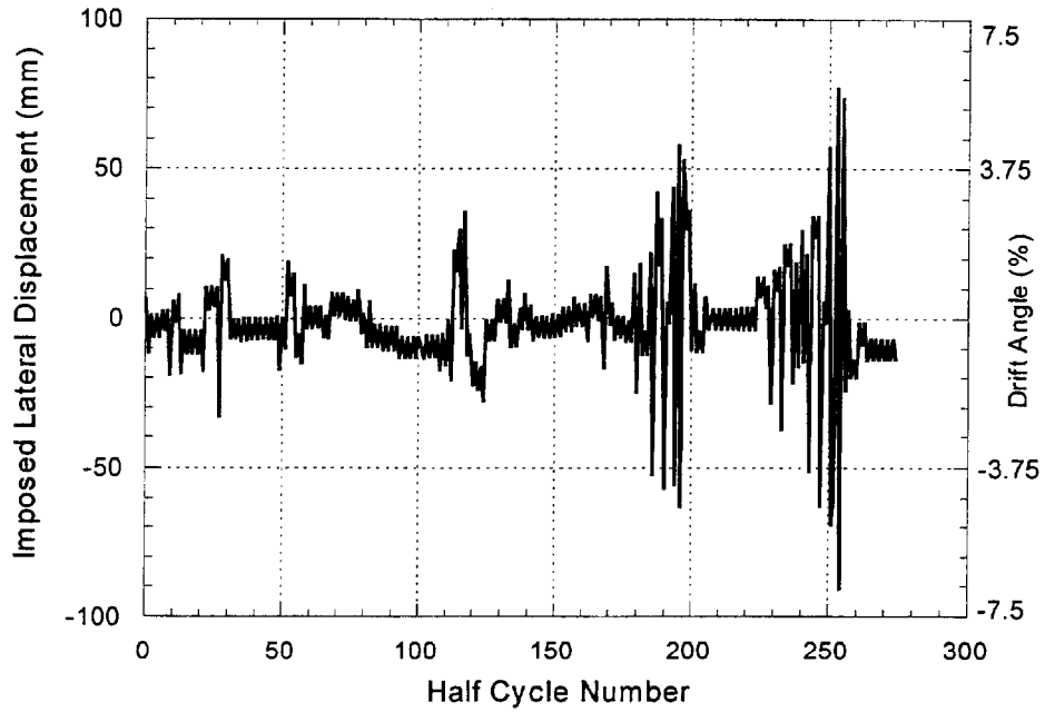
FIGURE 5-18 Displacement History Applied to Column A10
