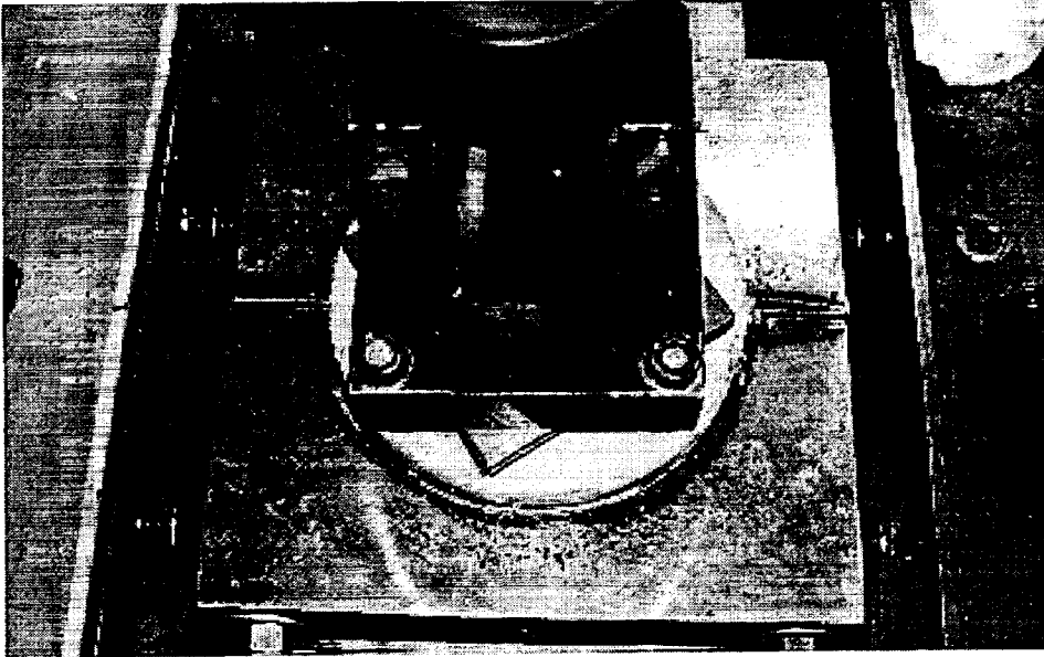
FIGURE 2-19 Overhead View of Out-of-Plane Support System
