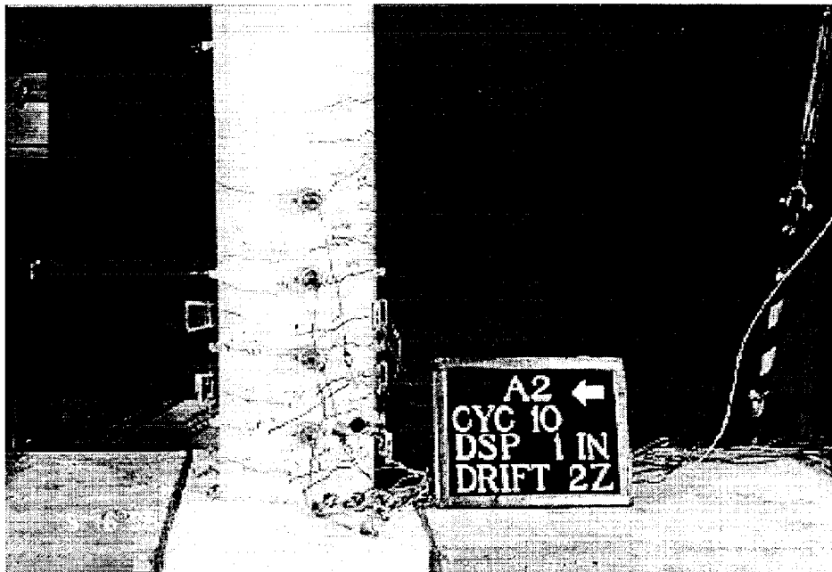
FIGURE 2-22 Electric Clinometers Used for Rotational Measurement
