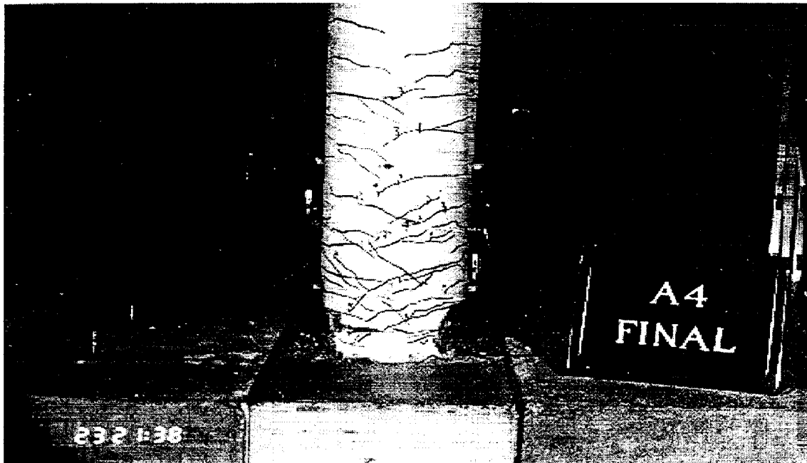
FIGURE 4-13 Condition of Specimen A4 at Cycle No. 18
