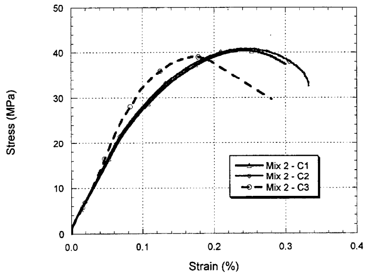
FIGURE 2-6 Stress vs. Strain for Concrete Mix 2 at 28 days
