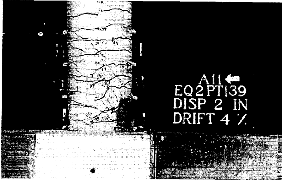
FIGURE 5-20 Specimen A11 at Half-Cycle # 139
