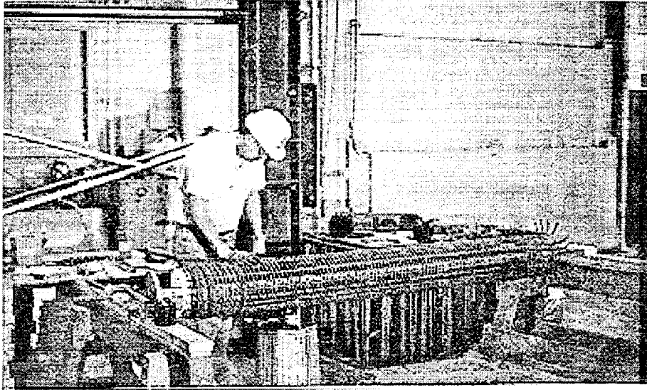
FIGURE 2-10 Cage Assembly for 1:4 Scale Model Piers
