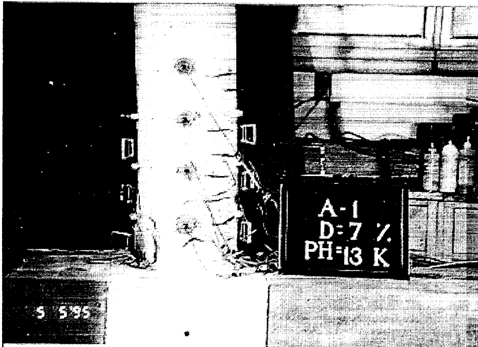
FIGURE 4-2 Damage to Specimen A1 at 3.5% Drift
