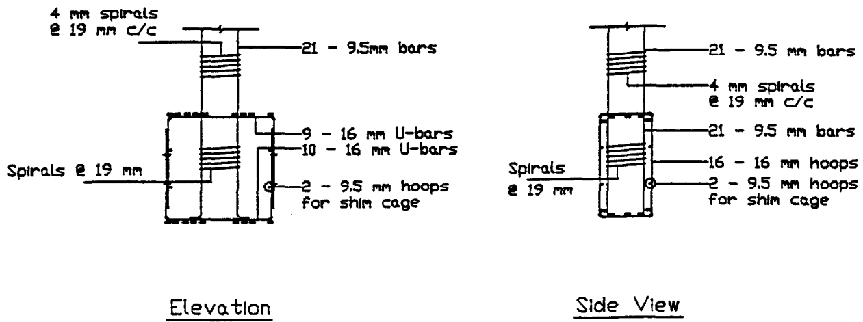
FIGURE 2-13 Reinforcement Arrangement for Specimen with Base Block
