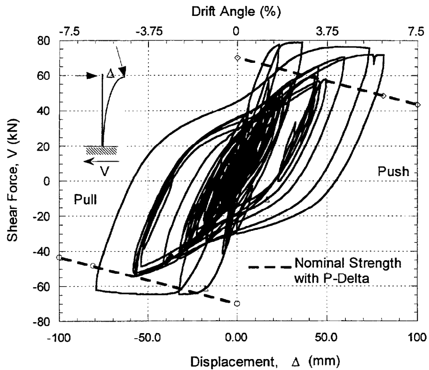
FIGURE 5-7 Force vs. Displacement Response of Column A7
