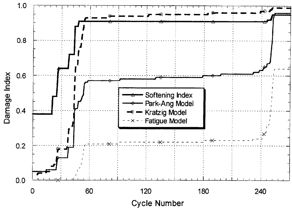
FIGURE 6-10 Comparative Evaluation of Progressive Damage for Specimen A8
