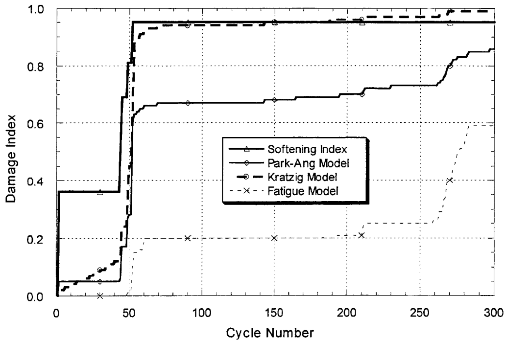
FIGURE 6-9 Comparative Evaluation of Progressive Damage for Specimen A7
