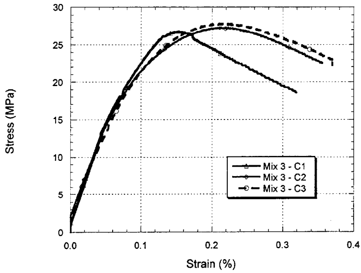
FIGURE 2-7 Stress vs. Strain for Concrete Mix 3 at 28 days
