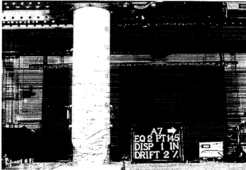
FIGURE 5-4 Damage to Specimen A7 at Half Cycle No. 145 During Earthquake #2
