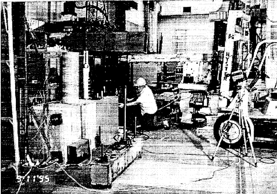
FIGURE 2-11 Post Tensioning of End Blocks to Footing
