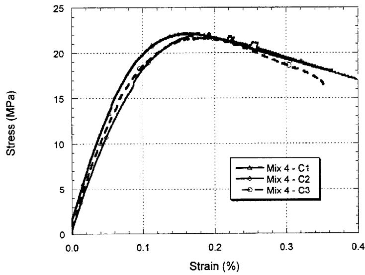
FIGURE 2-8 Stress vs. Strain for Concrete Mix 4 at 28 days
