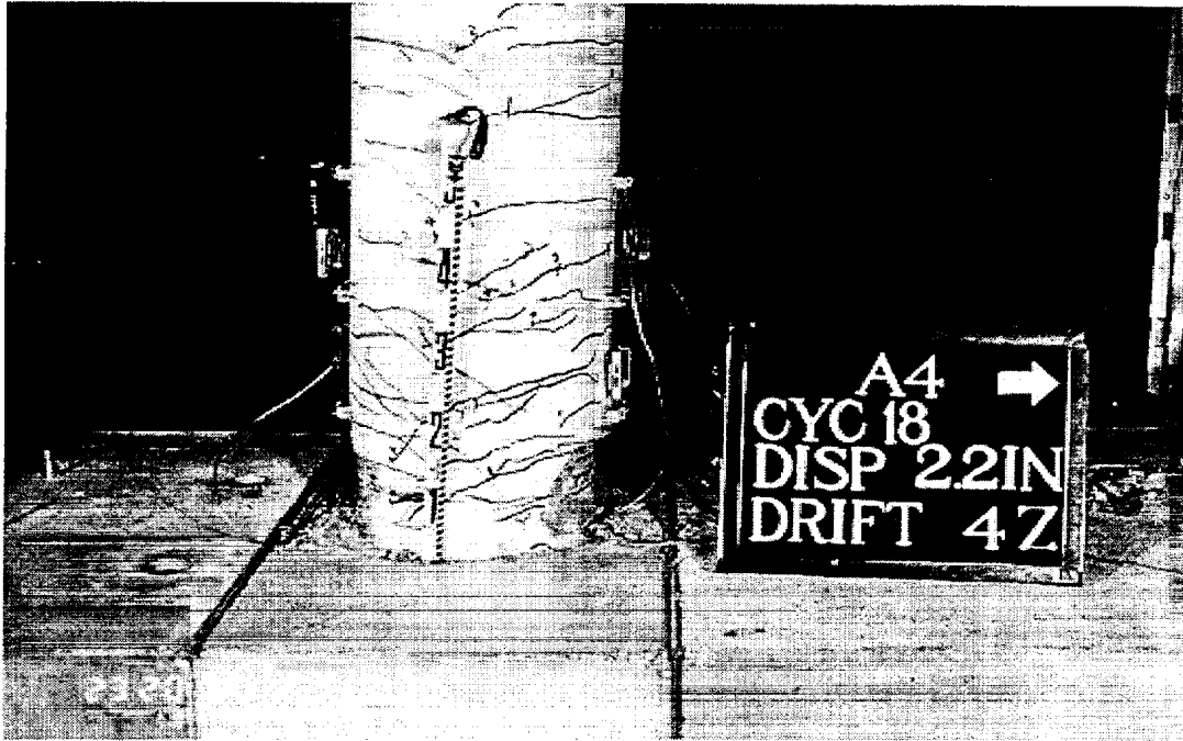
FIGURE 4-13 Condition of Specimen A4 at Cycle No. 18
