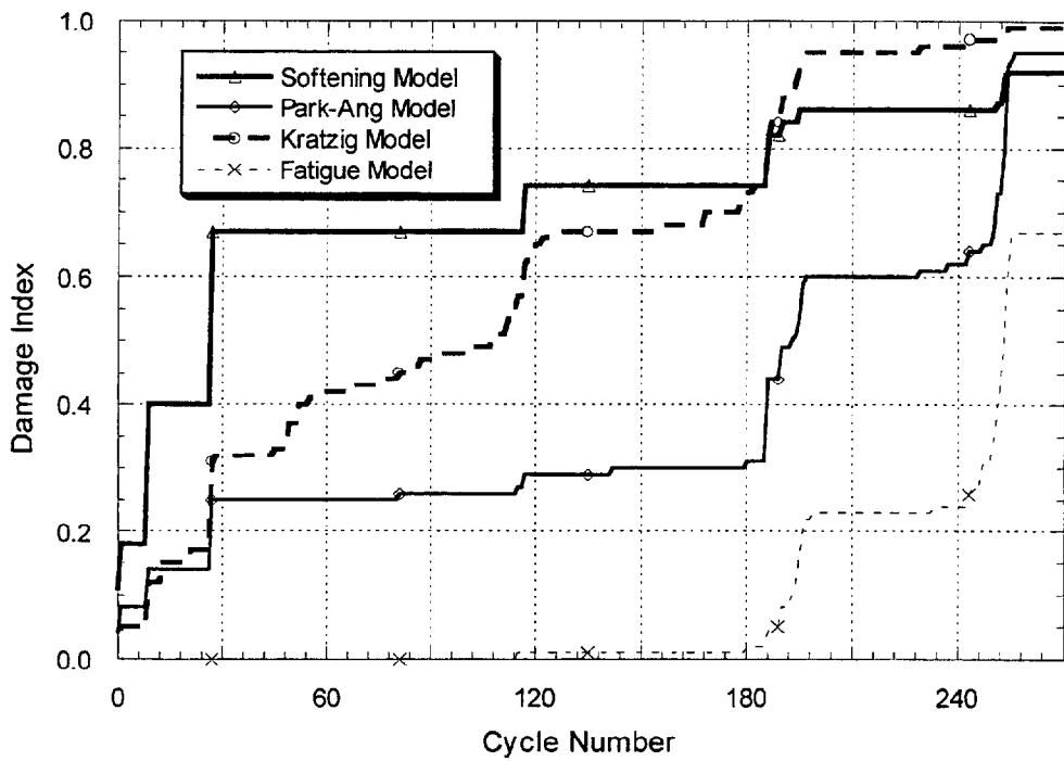
FIGURE 6-11 Comparative Evaluation of Progressive Damage for Specimen A9
