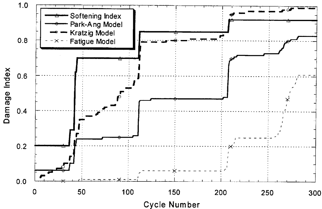
FIGURE 6-12 Comparative Evaluation of Progressive Damage for Specimen A10
