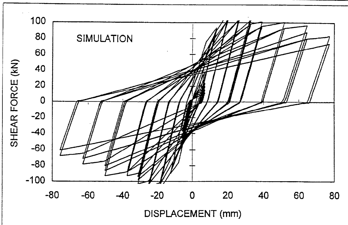
FIGURE 3-2 Calibration of Hysteresis Model
