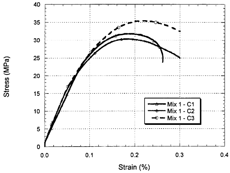
FIGURE 2-5 Stress vs. Strain for Concrete Mix 1 at 28 days
