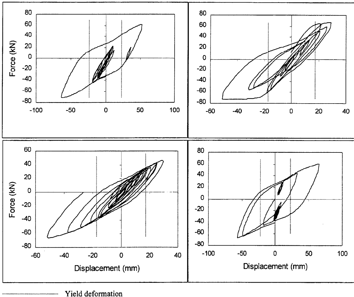
FIGURE 7-3 Local Loop Behavior Under Random Cyclic Response
