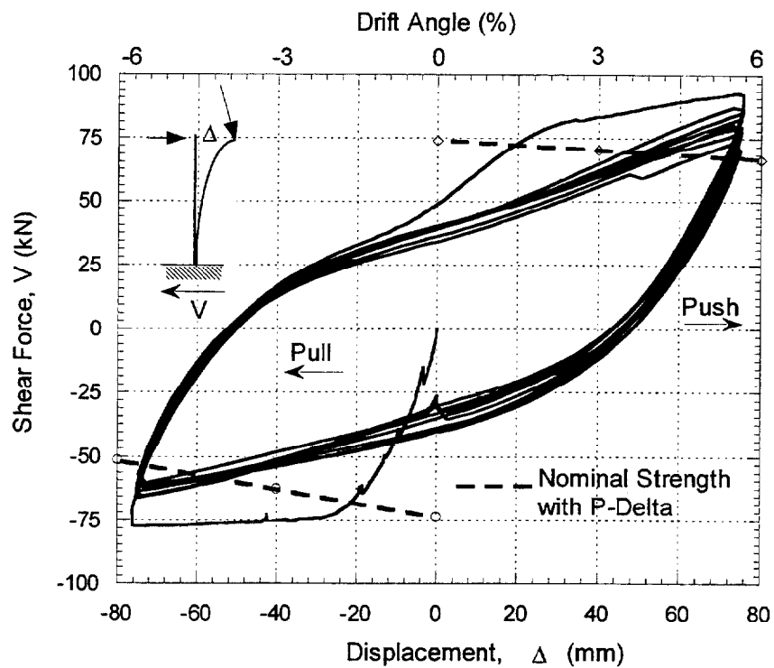
FIGURE 4-20 Shear vs. Displacement Response of Column A5
