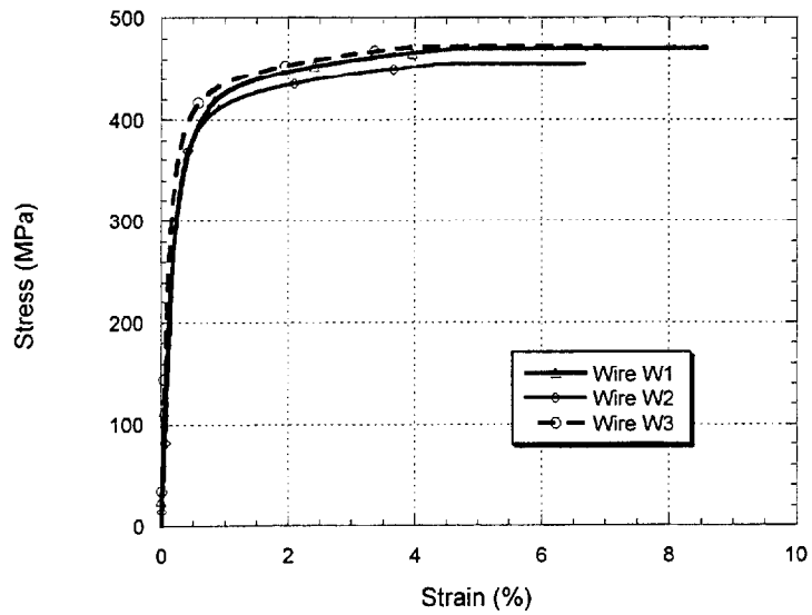
FIGURE 2-3 Stress vs. Strain Behavior of Annealed Wire Used for Spirals
