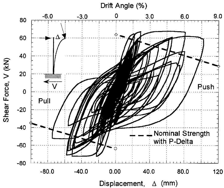
FIGURE 5-27 Base Shear vs. Lateral Displacement Response of Column A12
