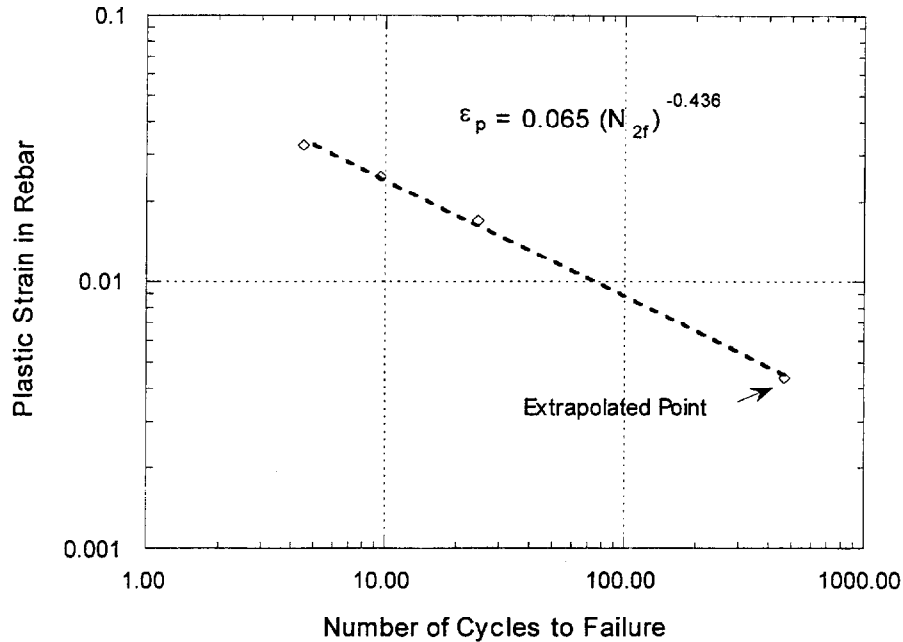
FIGURE 6-15 Coffin-Manson Fatigue Model for Plastic Strain
