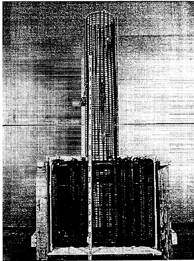
FIGURE 2-12 Cage Assembly for 1:4 Scale Model Column
