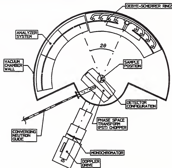
Figure 1. Schematic diagram of the CNRF backscattering spectrometer.
