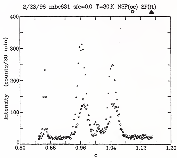
Figure 10. Polarized neutron scattering from the Cr antiferromagnetic structure at high angles, midway ( q = 1.0\text{\AA}^{-1} ) between the origin and the (002) Bragg peak in reciprocal space. (The sharp peak to the extreme left is not associated with the Cr magnetic structure.) The non-spin-flip scattering (open circles) is due to projections of the Cr moments parallel to the minimal magnetic field applied vertically and perpendicular to the scattering vector. The spin-flip scattering (filled triangles) arises from the horizontal projections of the Cr moments (but which are also perpendicular to the scattering vector). Two separate peaks appear, split about q = 1.0\text{\AA}^{-1} , due to the periodicity of the superlattice.
