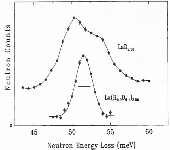
Figure 5. Comparison of the high-resolution \text{D}_o vibrational spectra for \text{LaD}_{2.50} and \text{La}(\text{H}_{0.9}\text{D}_{0.1})_{2.50} at 10 K.
