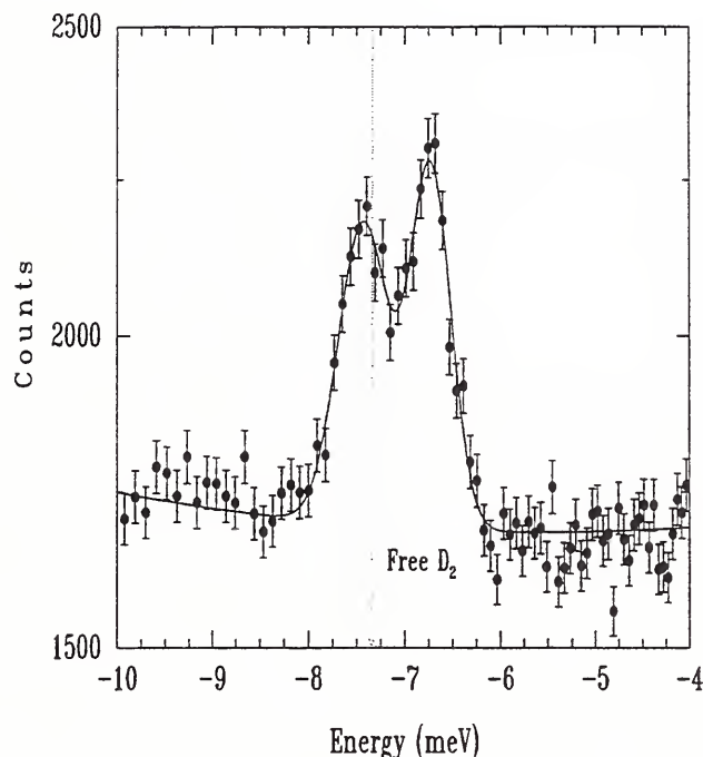
Figure 8. Time-of-flight energy gain spectrum of interstitial D_2 in C_{60} . The data are taken at 10K.
