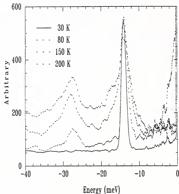
Figure 7. The temperature dependence of the energy gain spectrum for interstitial H_2 in C_{60} .
