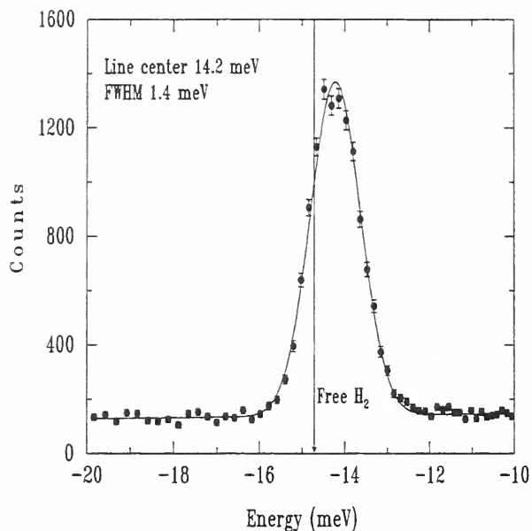
Figure 6. Time-of-flight energy gain spectrum of interstitial H_2 in C_{60} . The data are taken at 30 K.
