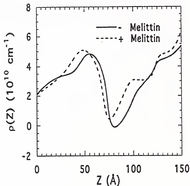
Figure 8. Representative neutron SLD profiles obtained from model-independent fits to the data in Fig. 7. The profiles for the sample with melittin consistently show a higher SLD in the acyl chain region of the d(54) -DMPC, indicating that melittin penetrates at least into this region. High resolution measurements are necessary to further pinpoint its location.
