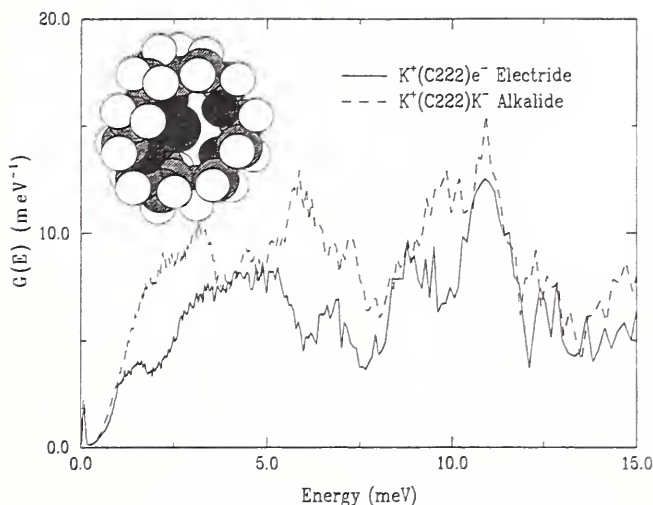
Figure 16. Low frequency vibrational density of states of the alkalide K^+(C222)K^- and electrider K^+(C222)e^- . Above \sim 15 meV, the vibrational spectra are virtually identical for both compounds. Inset: Structure of the K^+(C222) cryptand cation. The potassium ion is encapsulated within a cage formed by the three (CH_2)_2O(CH_2)_2O(CH_2)_2 legs of the cryptand which are joined at the poles by nitrogen atoms.
