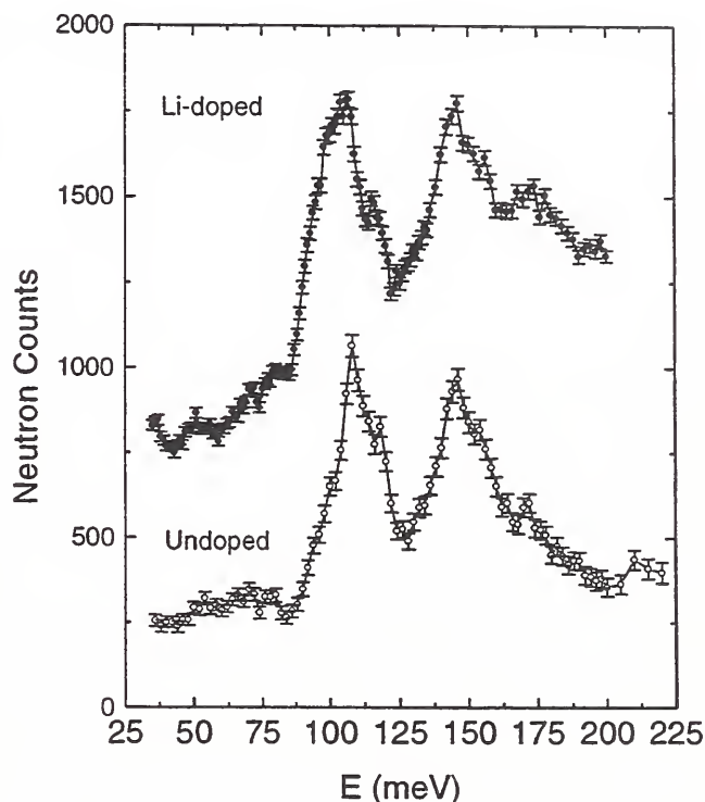
Figure 15. Inelastic neutron scattering spectra of DC650 before and after lithium doping, measured at 16K using the Be filter. The latter is shifted vertically for clarity.
