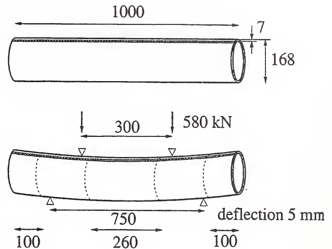
Figure 4. Schematic of the bent tube before bending and cutting. The weld parallels the cylinder axis. The central 260 mm and the outer 100 mm portions are cut out and used for the neutron measurements.
