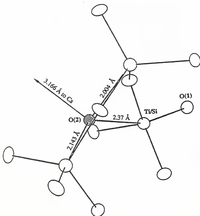
Figure 6. Environment of one of the extra oxygen atoms (shaded circle), showing its relationship to the neighboring \text{TO}_4 tetrahedra.
