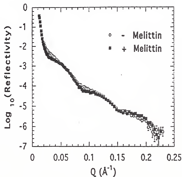
Figure 7. \text{Log}_{10}(\text{reflectivity}) vs Q from a \text{C}_{18}\text{SH}/\text{d}(54)\text{-DMPC} HBM in \text{D}_2\text{O} in the presence (+) and absence (-) of melittin, a pore-forming toxin which is active in HBMs. The data show qualitatively that melittin serves to change the contrast of the HBM relative to the \text{D}_2\text{O} but has relatively little influence on its total thickness. This suggests that melittin penetrates at least partially into the HBM.
