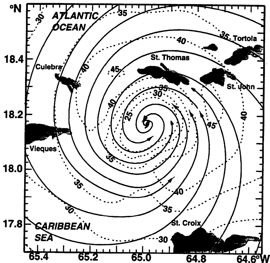
Figure 4. Typical plot of HRD surface wind analysis for Hurricane Marilyn valid at 0330 UTC 16 September 1995. Isotachs (m/s) and streamlines (solid) are shown for maximum 1-minute wind speeds at 10 m over water (Powell and Houston 1997).
