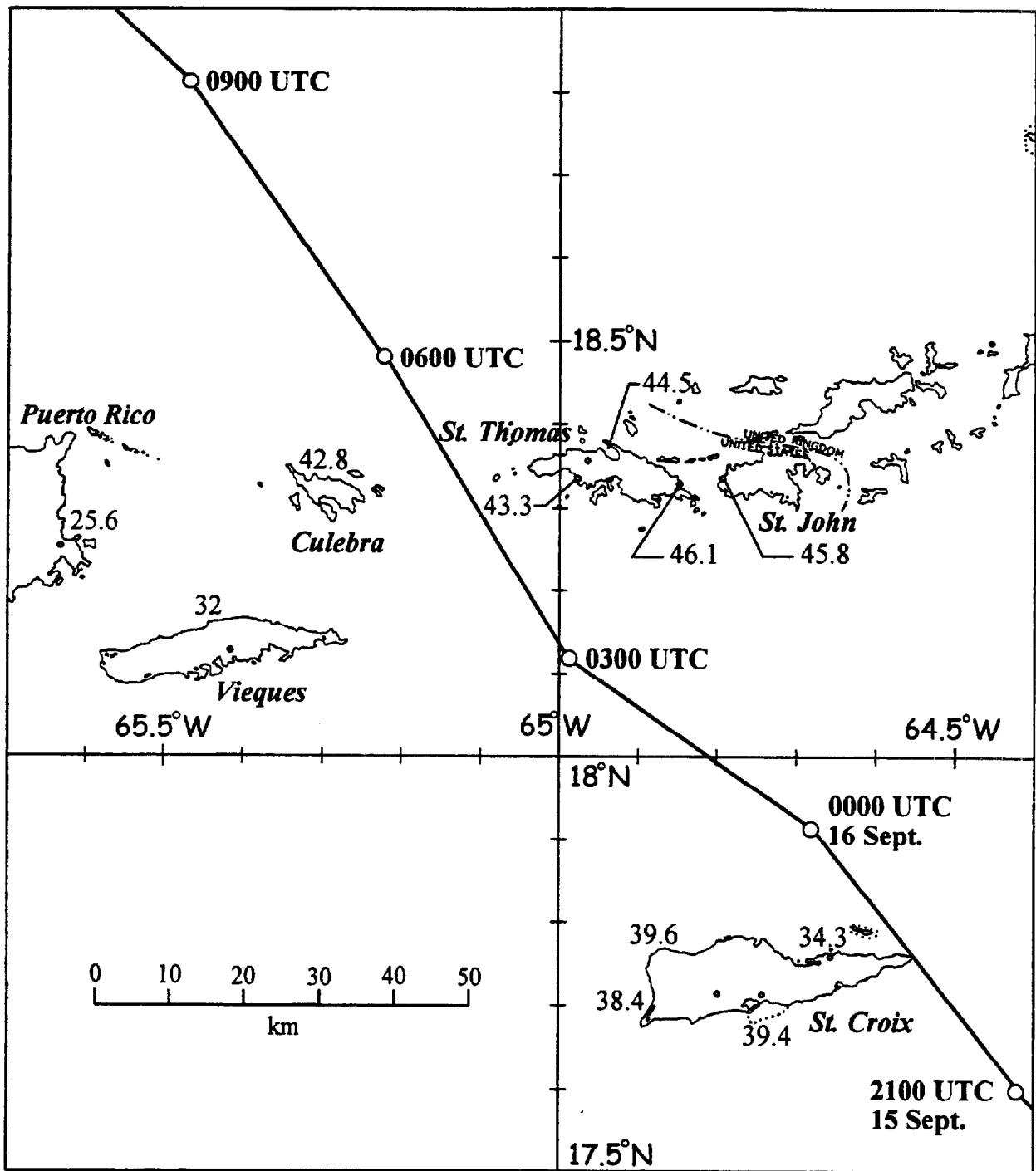
Figure 5. Probable maximum over-water sustained speeds (m/s) in Hurricane Marilyn based on HRD analysis.
