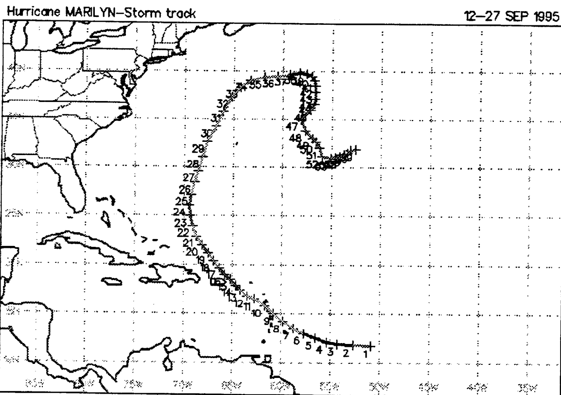
Figure 1. Hurricane Marilyn's complete storm track. Source: Department of Earth and Atmospheric Sciences, Purdue University.
