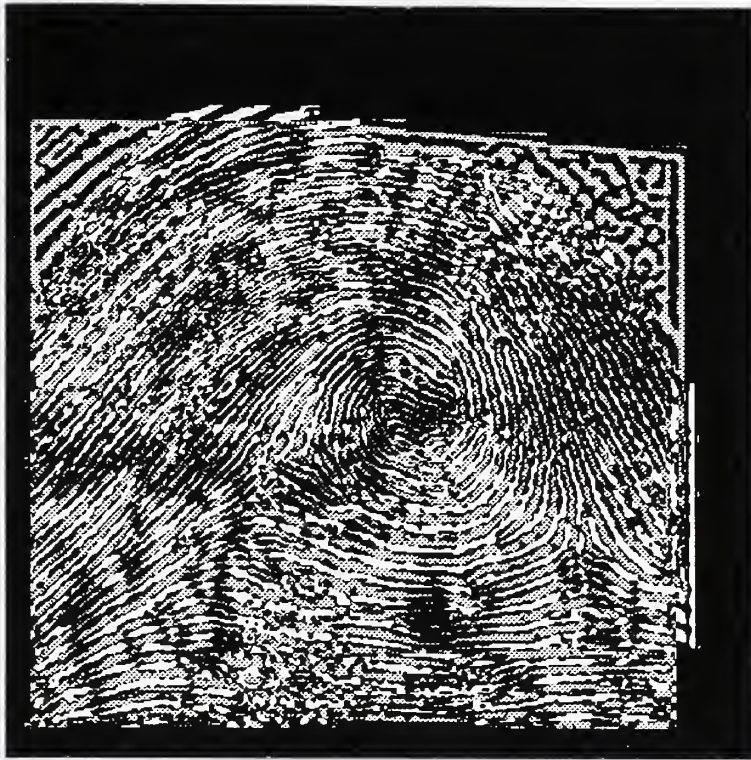
Figure 3: Correlation of two rollings of the same print. (Dark gray indicates correlated ridges, white and light gray indicate uncorrelated ridges.)
