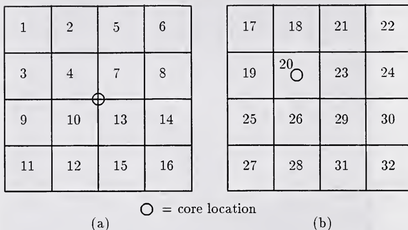
Figure 4: Shows image partitioning and the corresponding feature number.
