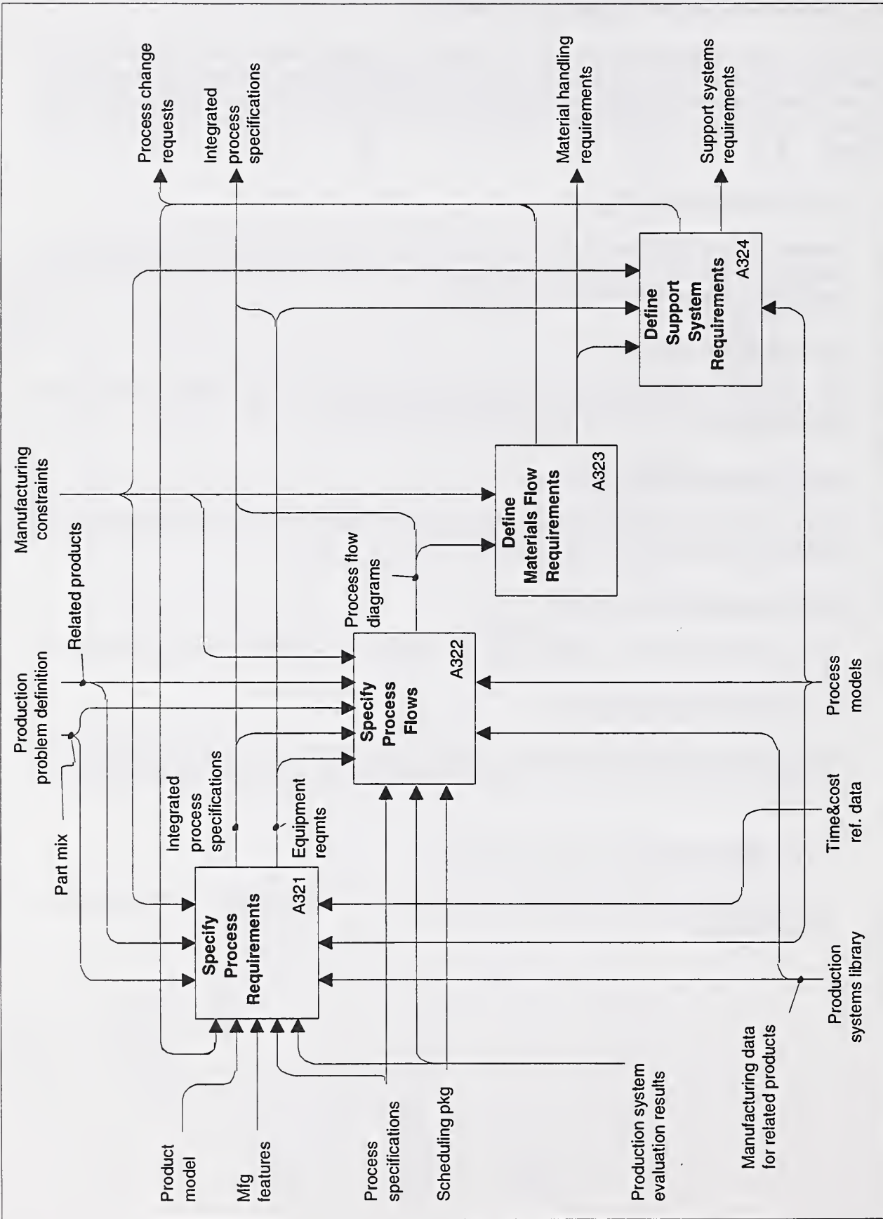
SIMA Manufacturing Activity Model Node: A32 Specify Production & Support Processes
