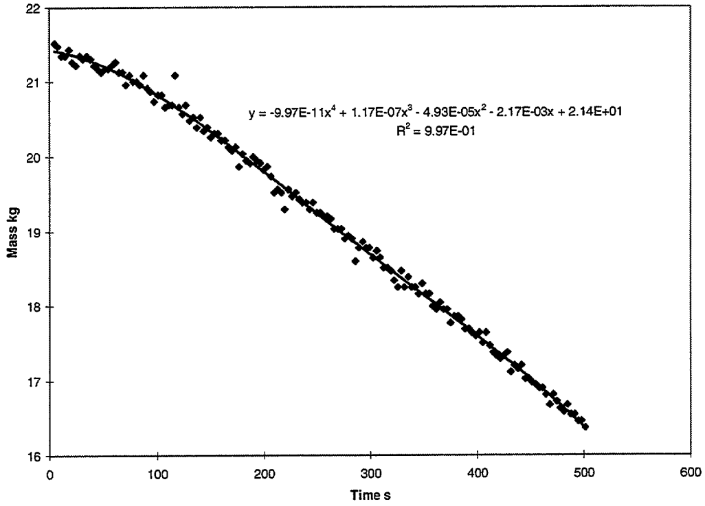
Figure 3 Load Cell Polynomial Fit for 500 kW Fire
