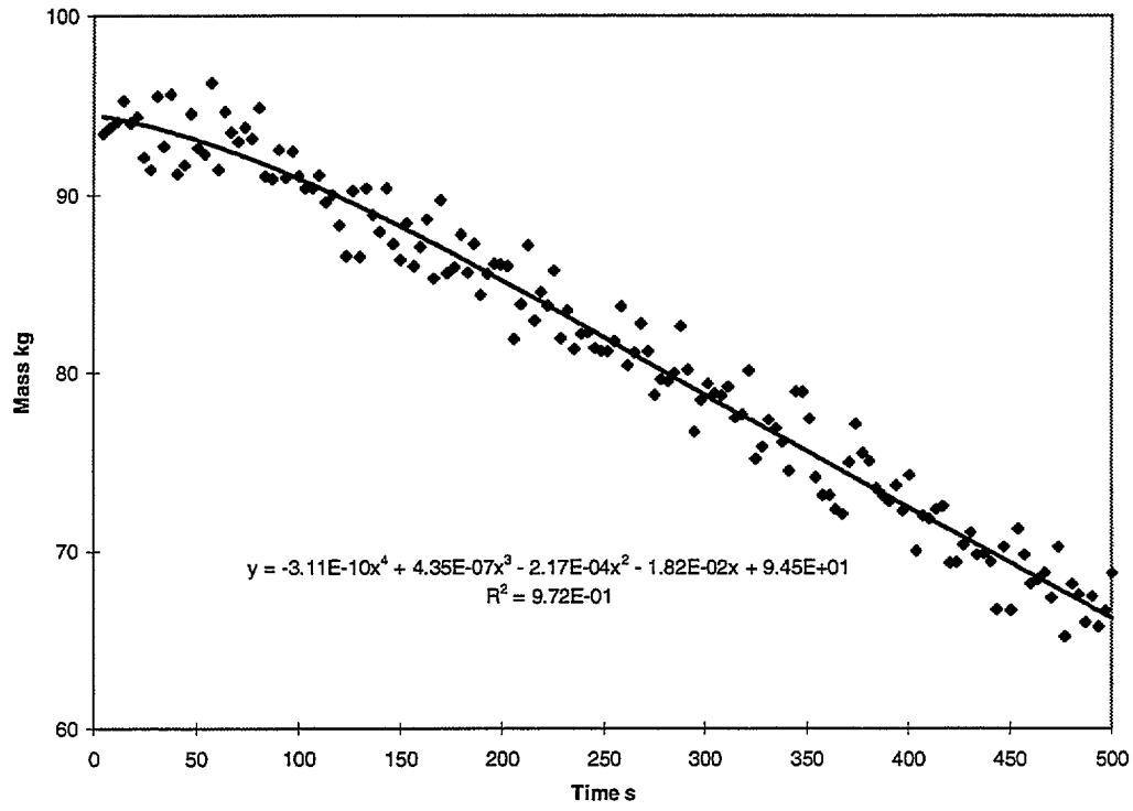
Figure 4 Load Cell Polynomial Fit for 2.7 MW Fire
