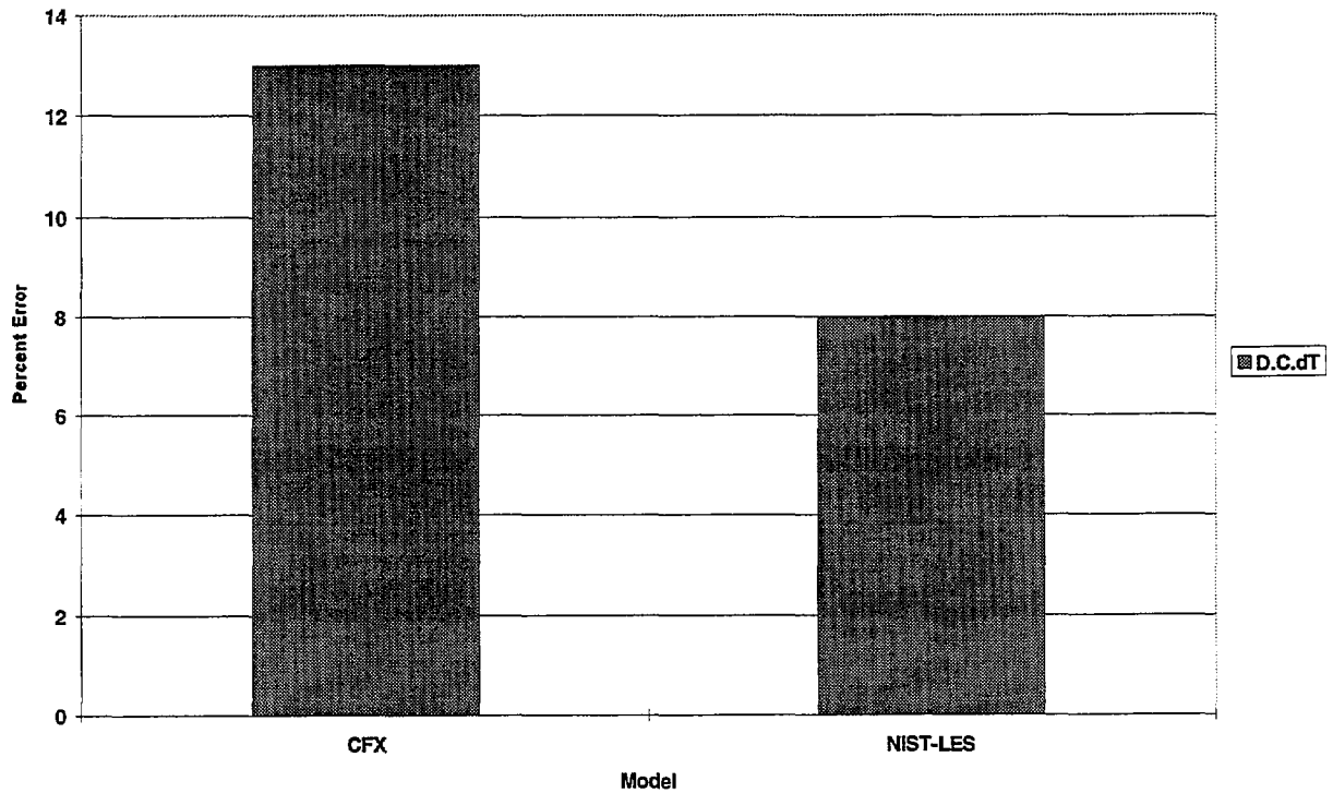
Figure 20 Deviations between Model Predictions and Measured temperature Jump Across the Draft Curtain
