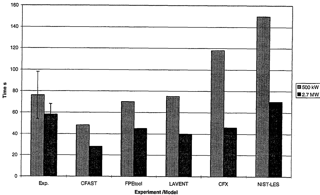
Figure 12 Draft Curtain Spilling Time
