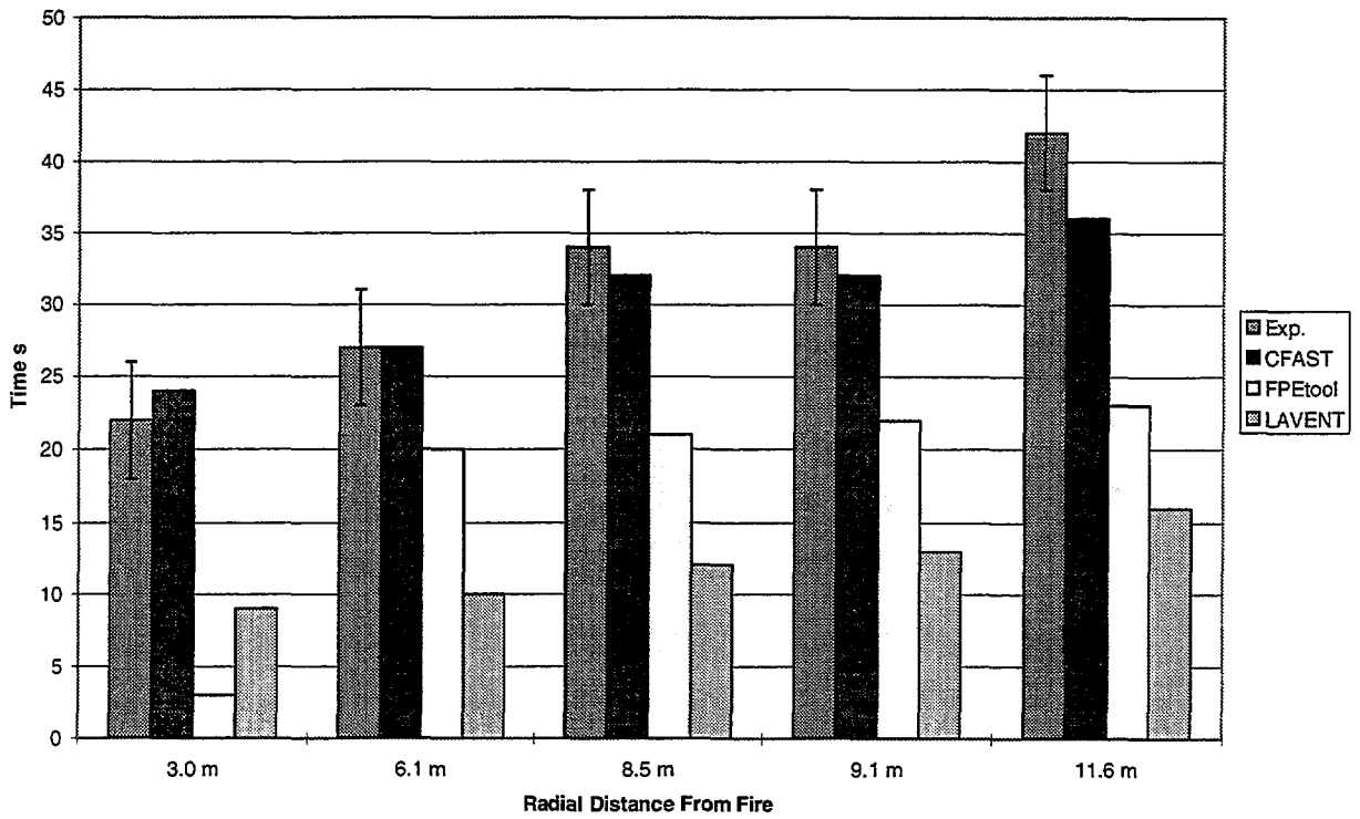
Figure 16 Smoke Detector Activation with Zone Model Predictions for the 2.7 MW Fire
