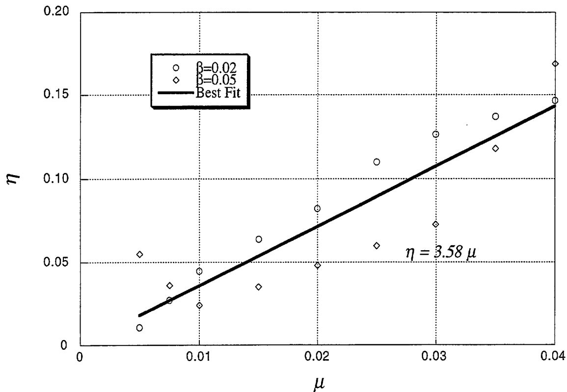
Figure 3.5 Relationship between the constant \eta and the mass ratio \mu
