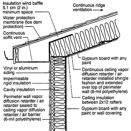
b. Roof 2 - Heating Climate (Vented Cathedral Ceiling)
