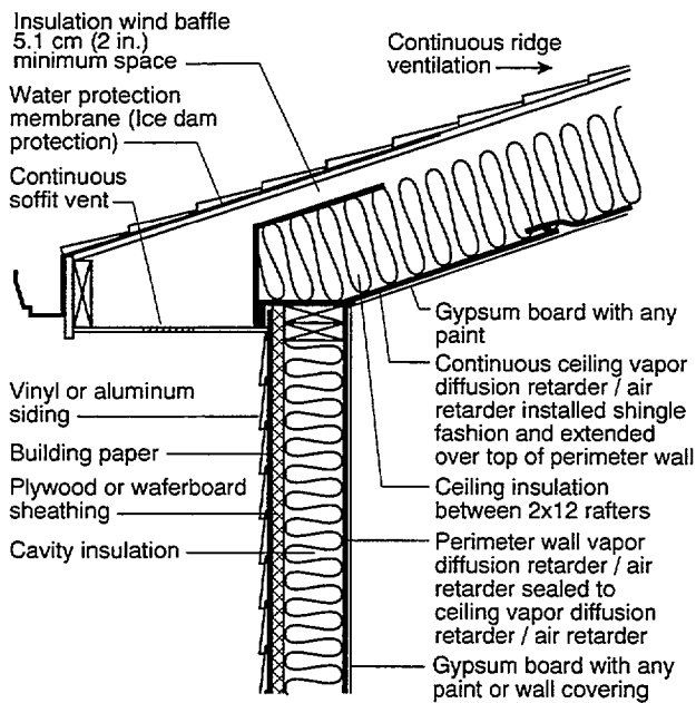
c. Roof 3 - Mixed Climate (Vented Cathedral Ceiling)
