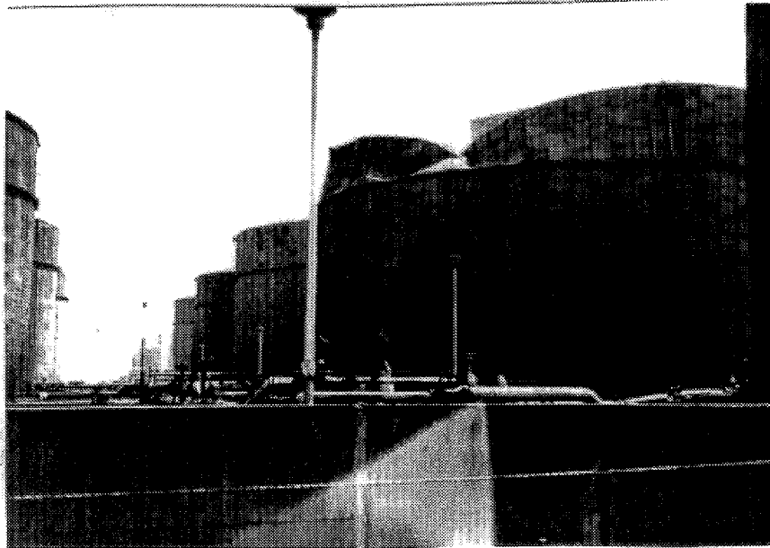
Figure 3. Imploded tanks in Sendai, Japan, from 1978 earthquake.
