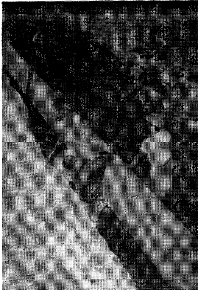
Figure 1. Typical pipeline earthquake failure repair.
