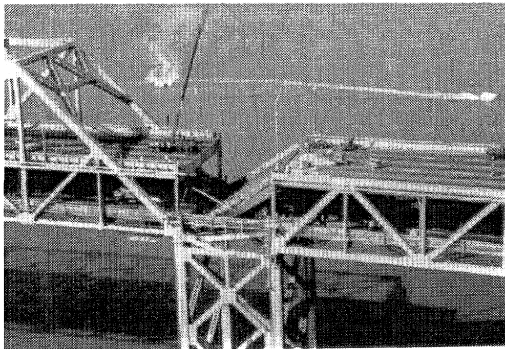
Figure 12a. Aerial photo looking north at pier E-9 on October 19, 1989, showing the collapsed upper and lower 15.1 m deck spans.
