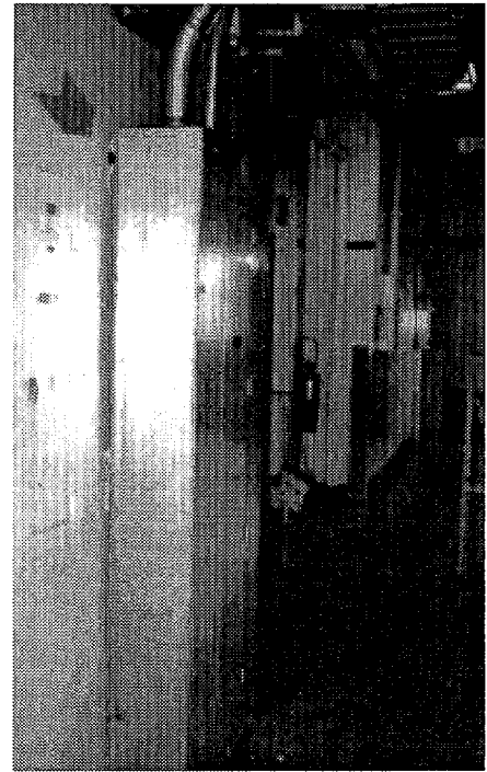
Photo 5. Loma Prieta earthquake 1989. An AC panel in a central office pulled away from the wall. Close up view on the left.
