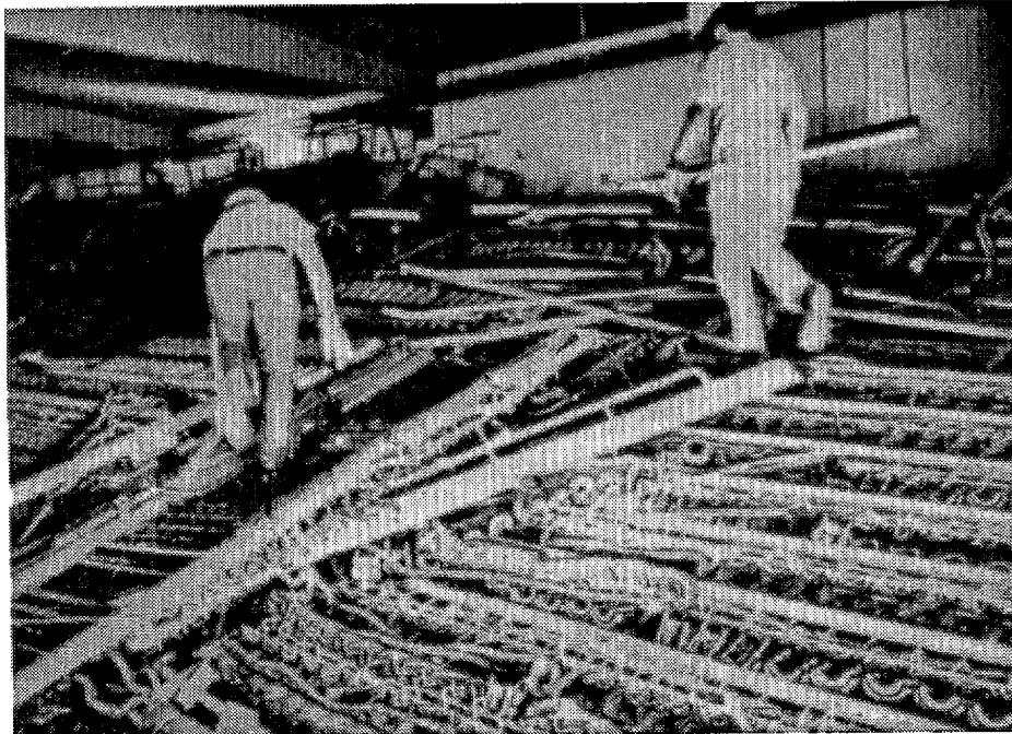
Photo 1. Sylmer CO after San Fernando earthquake 1971. Overhead bracing failure resulted in switching equipment collapse. Cost $4.5 million to restore.
