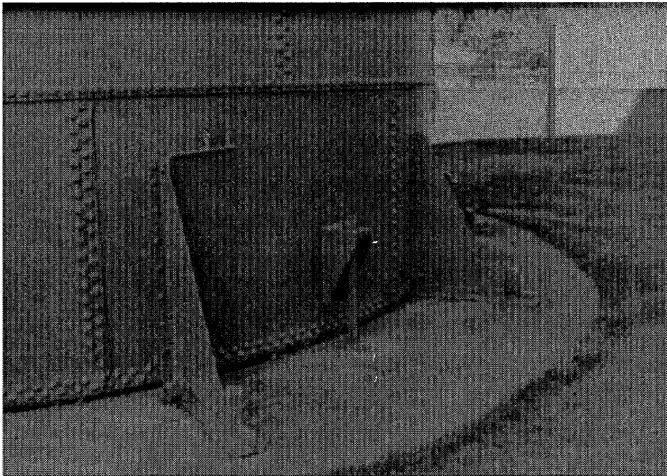
Figure 10. Seismic upgrade to a standpipe.
