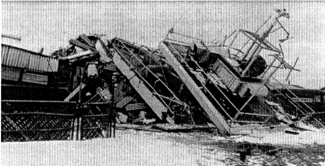
Figure 3. Collapsed control tower at Anchorage International Airport. Prince William Sound earthquake, March 27, 1964.
