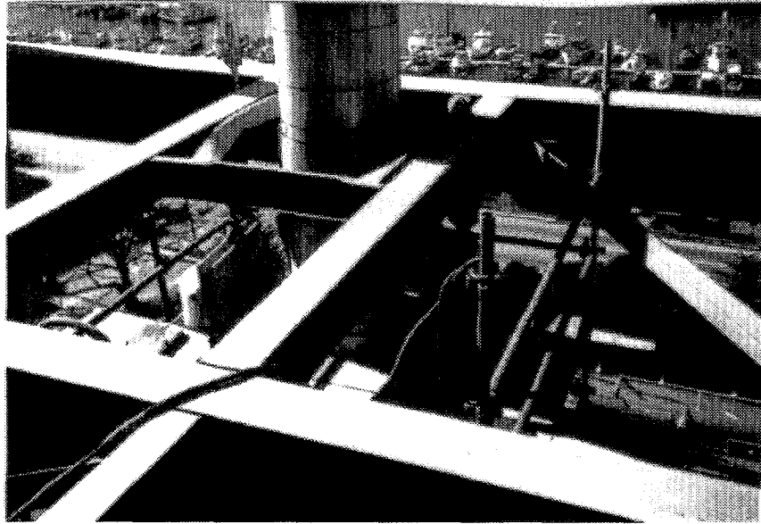
Figure 5. Damaged steam pipe restraint.
