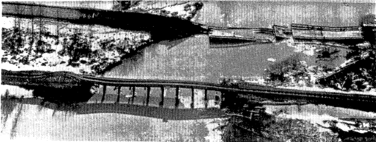
Figure 1. Collapsed bridge on the Seward Highway. Also track damage on approaches to adjacent railroad bridge. Prince William Sound earthquake, March 27, 1964.
