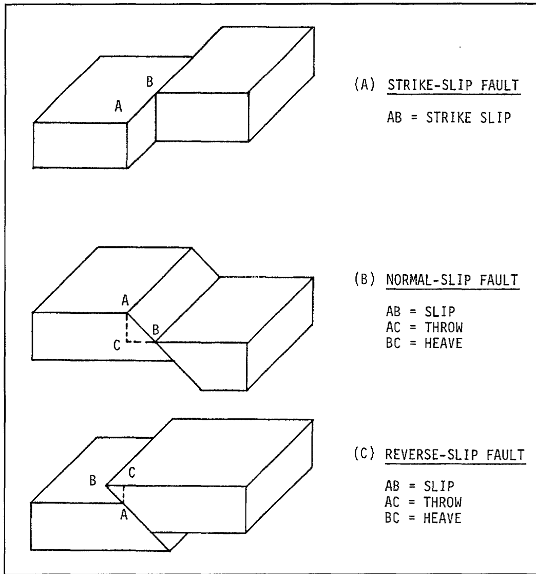
Figure 4. Types of fault movement (after Krinitsky, 1974).
