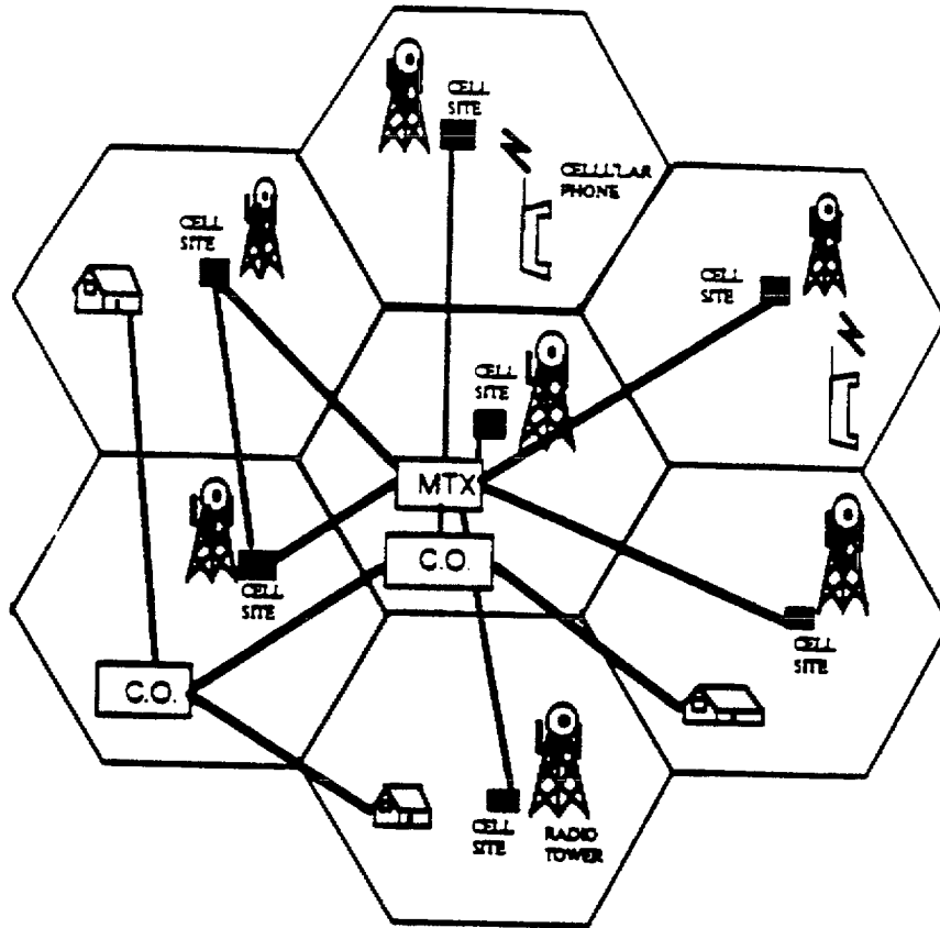
Figure 2. Cellular radio concept.
