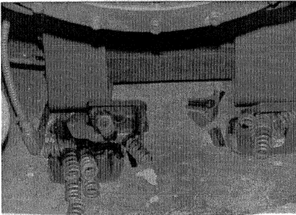
Figure 4. Spring vibration isolator on an engine-generator set, damaged in an earthquake.
