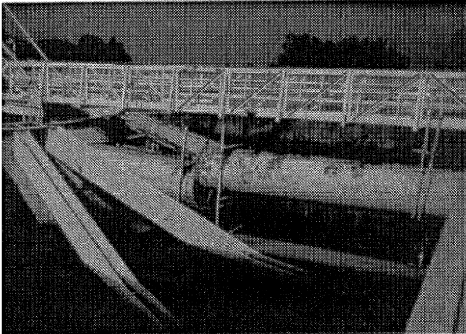
Figure 6. Sloshing damage to a clarifier at the Rinconada Water Treatment Plant resulting from the Loma Prieta Earthquake.
