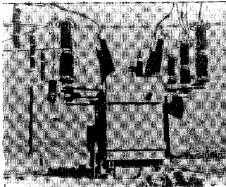
Figure 8. Unanchored transformer slides and damages lightning arrester.
