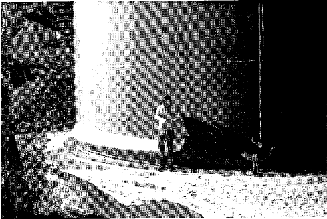
Figure 8. Circumferential buckle in water tank, Olive View Hospital, 1971 San Fernando Earthquake.
