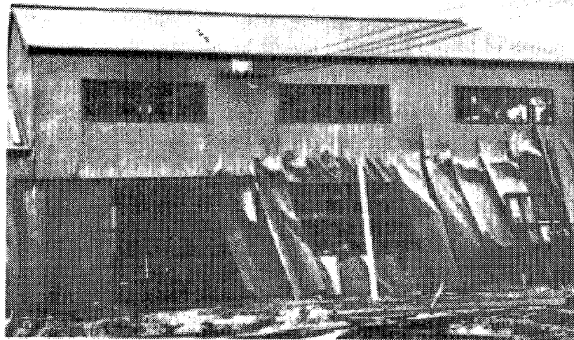
Figure 4b. Building pulled apart by lateral spreading during the 1964 Niigata earthquake. Source: Kawasumi (1968).
