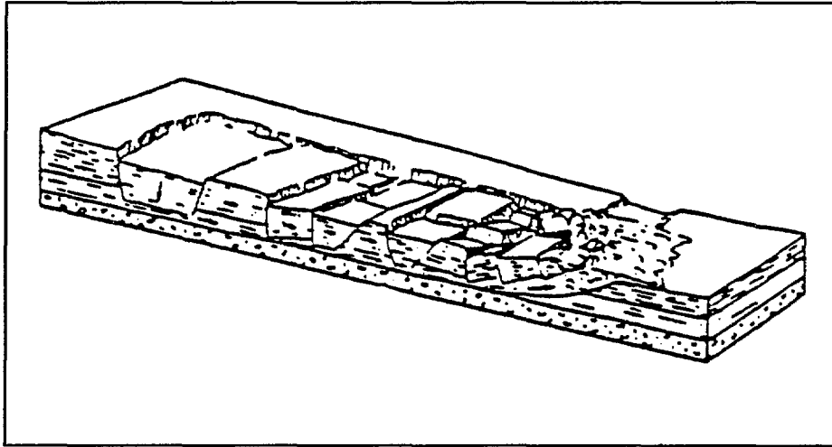
Figure 6. Lateral spread ground displacement (after Schuster and Fleming, 1982).
