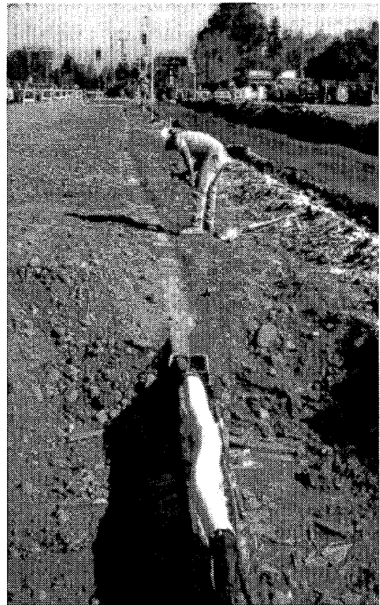
Photo 10. Burying fibre optic cable in process.
