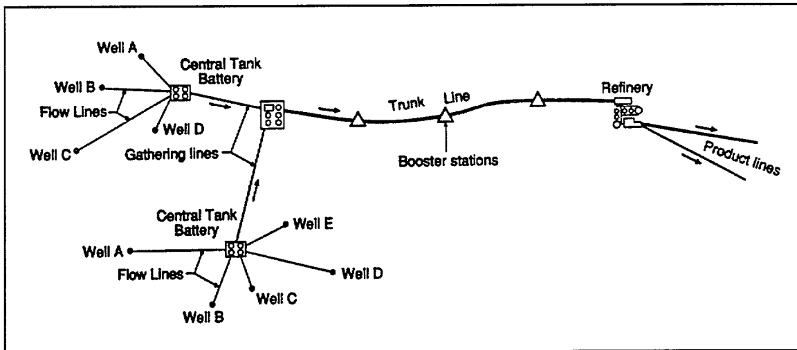
Figure 2. Schematic of liquid fuel pipeline system (after Yokel and Mathey, Giuliano, 1981).
