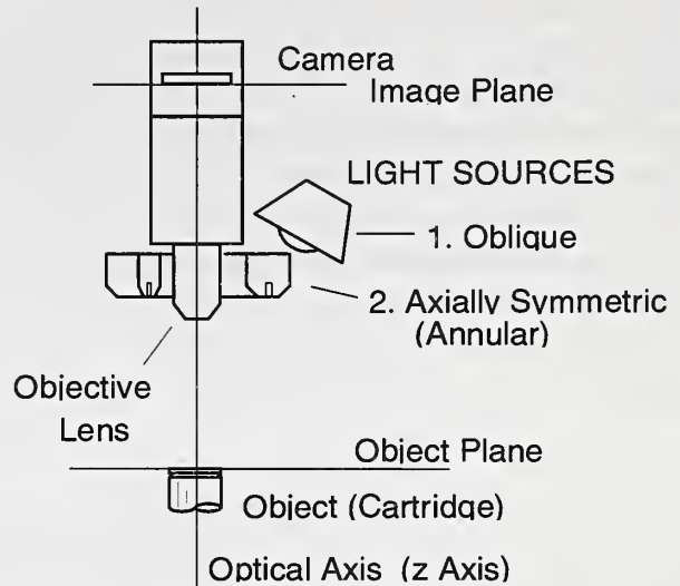
Figure 1. Optical configuration for ballistic cartridge imagery used in this document. (Axially symmetric light source shown in partial cross-section.)
