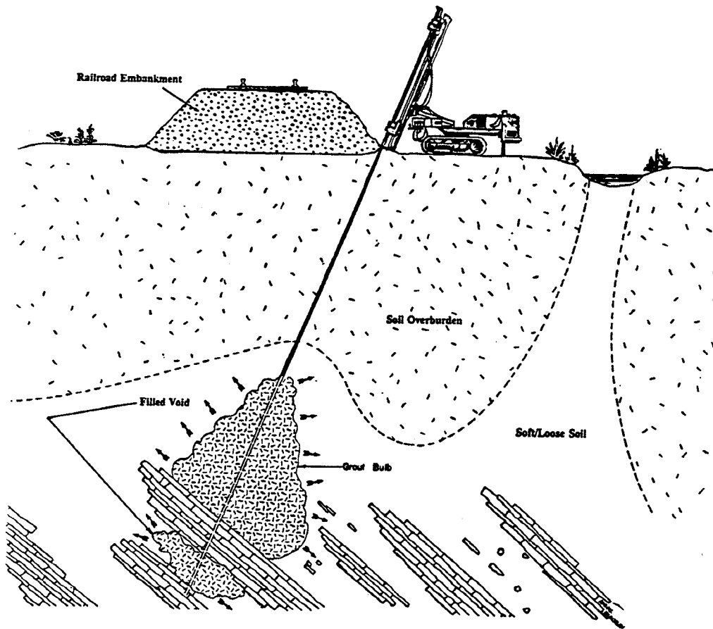
Fig. 3.6 - Remediation of Settled Rail Line in Sinkhole Area by Compaction Grouting (Brill and Hussin, 1992).
