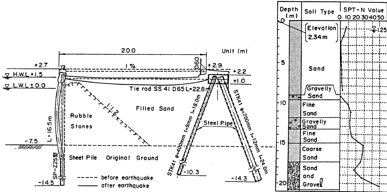
Fig. 2.34 - Cross Section of a Damaged Steel Sheet Pile Quay Wall at Kushiro Port, Japan, Showing Ground Conditions and Wall Deformations Caused by Liquefaction-induced Horizontal Ground Movement (Iai et al., 1994).
