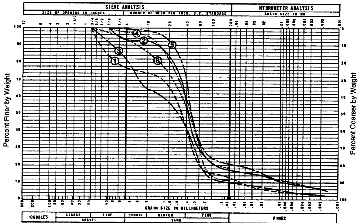
Fig. 2.3 - Grain-size Distribution Curves of Split-Barrel Samples Taken from the Loose Sand at the Pinopolis West Dam (Salley et al., 1987).
