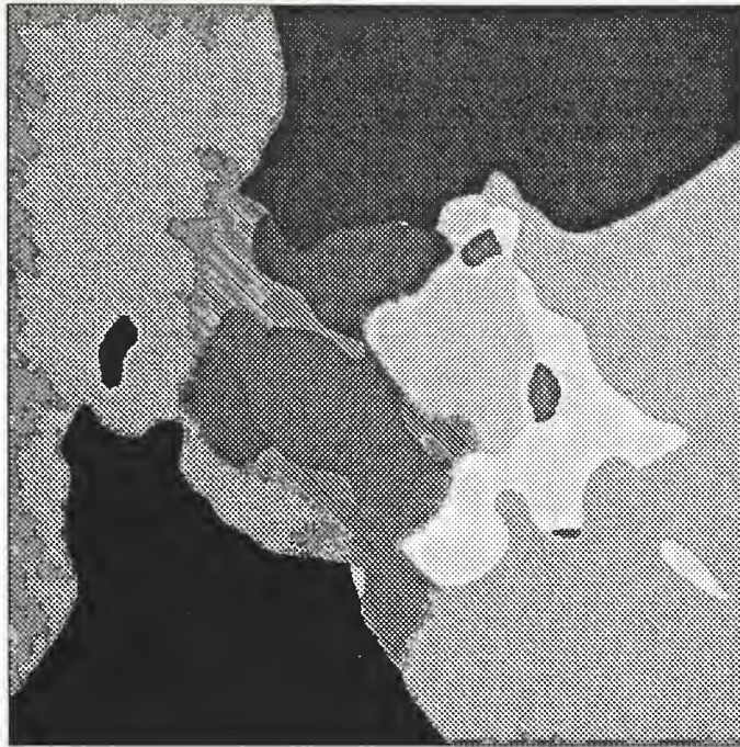
Figure 1: The diagram shows digit classifications generated by a PNN classifier using the first two K-L components in a region centered on (0, 0) with an extent large enough to contain the feature vectors.
