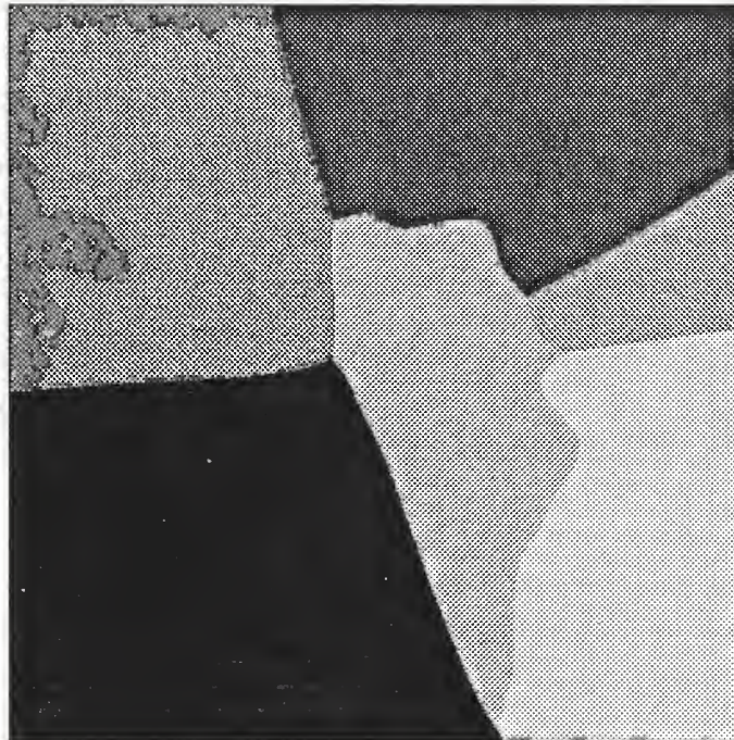
Figure 2: The diagram shows digit classifications generated by a MLP classifier using the first two K-L components in a region centered on (0, 0) with an extent large enough to contain the feature vectors.
