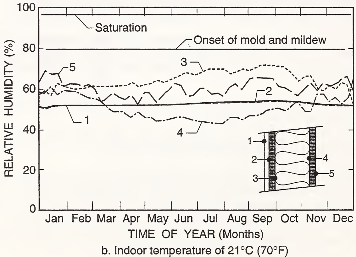
Fig. 7. Surface relative humidity of layers plotted versus time of year for variable-permeance-claddings wall exposed to Miami, FL weather.
