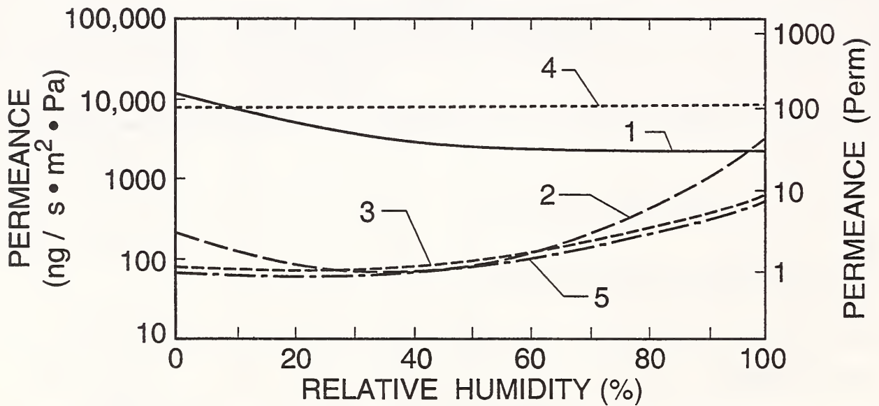
b. Permeances
