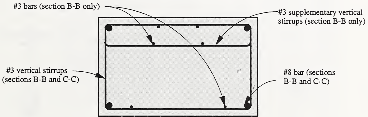
b) Sections B-B and C-C
