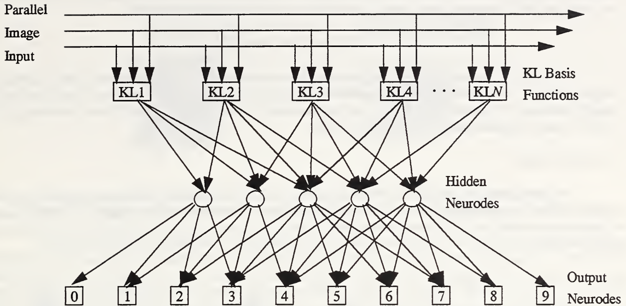
Figure D.11. KL feature-based MLP network model.
