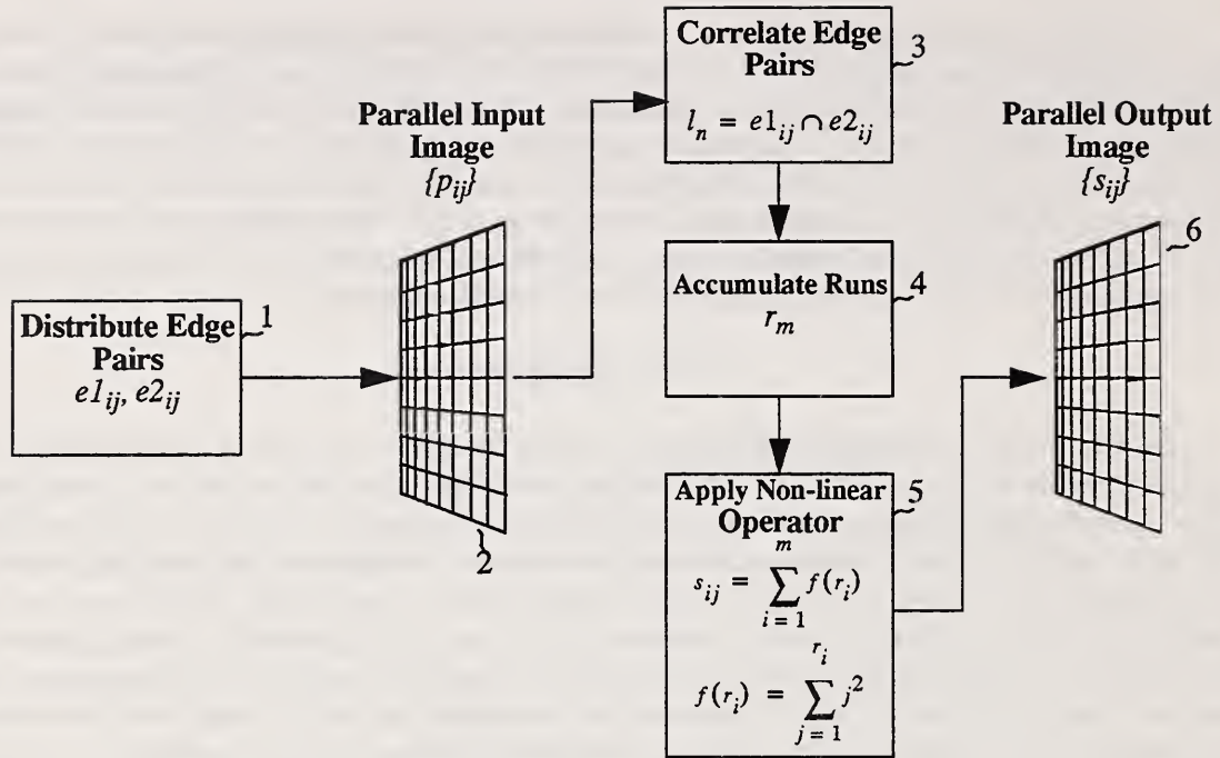
Figure D.1. Flow diagram describing the CURL algorithm.
