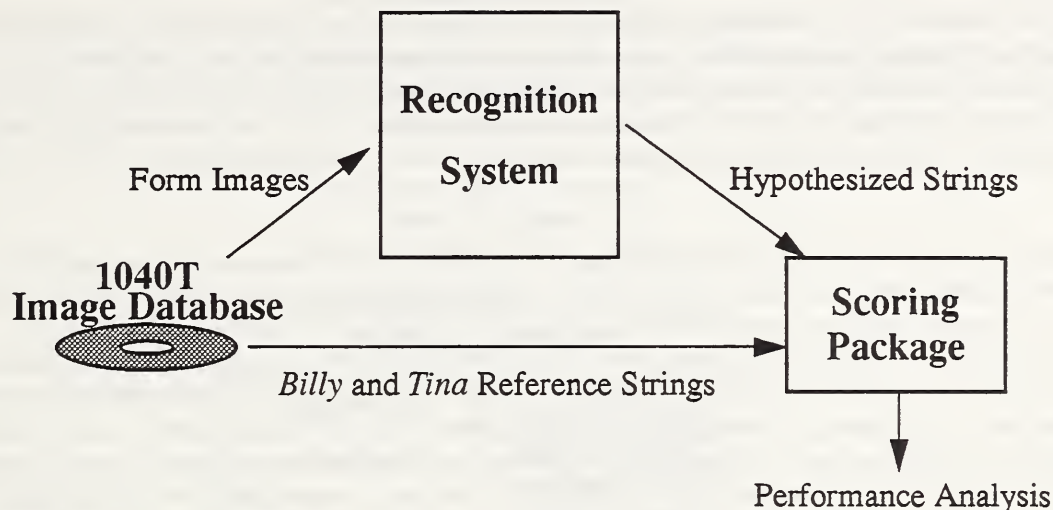
Figure 3. Testing paradigm for recognition systems using the 1040T database and the Scoring Package.
