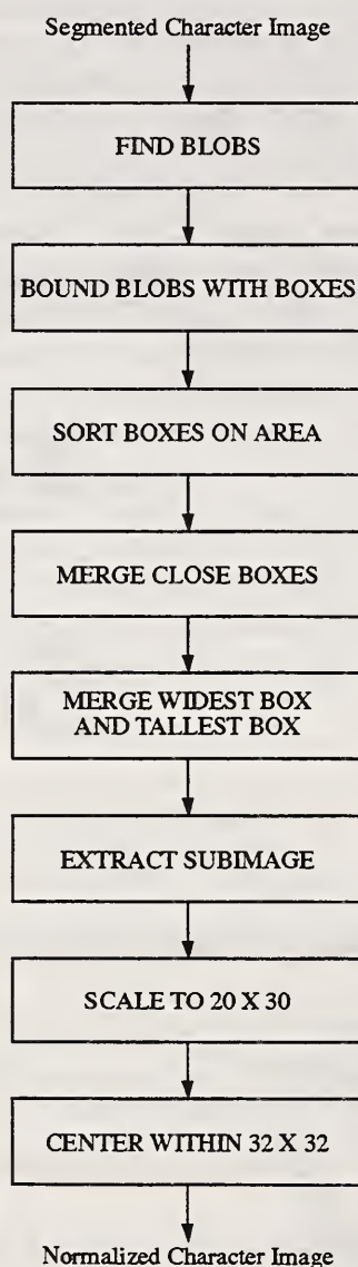
Figure D.9. Third generation normalization process flow.
