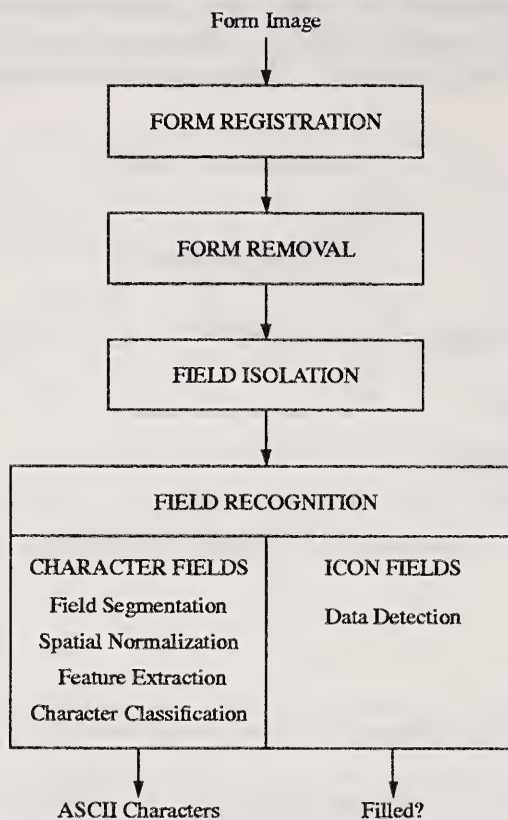
Figure 4. Functional components of the Model Recognition System.
