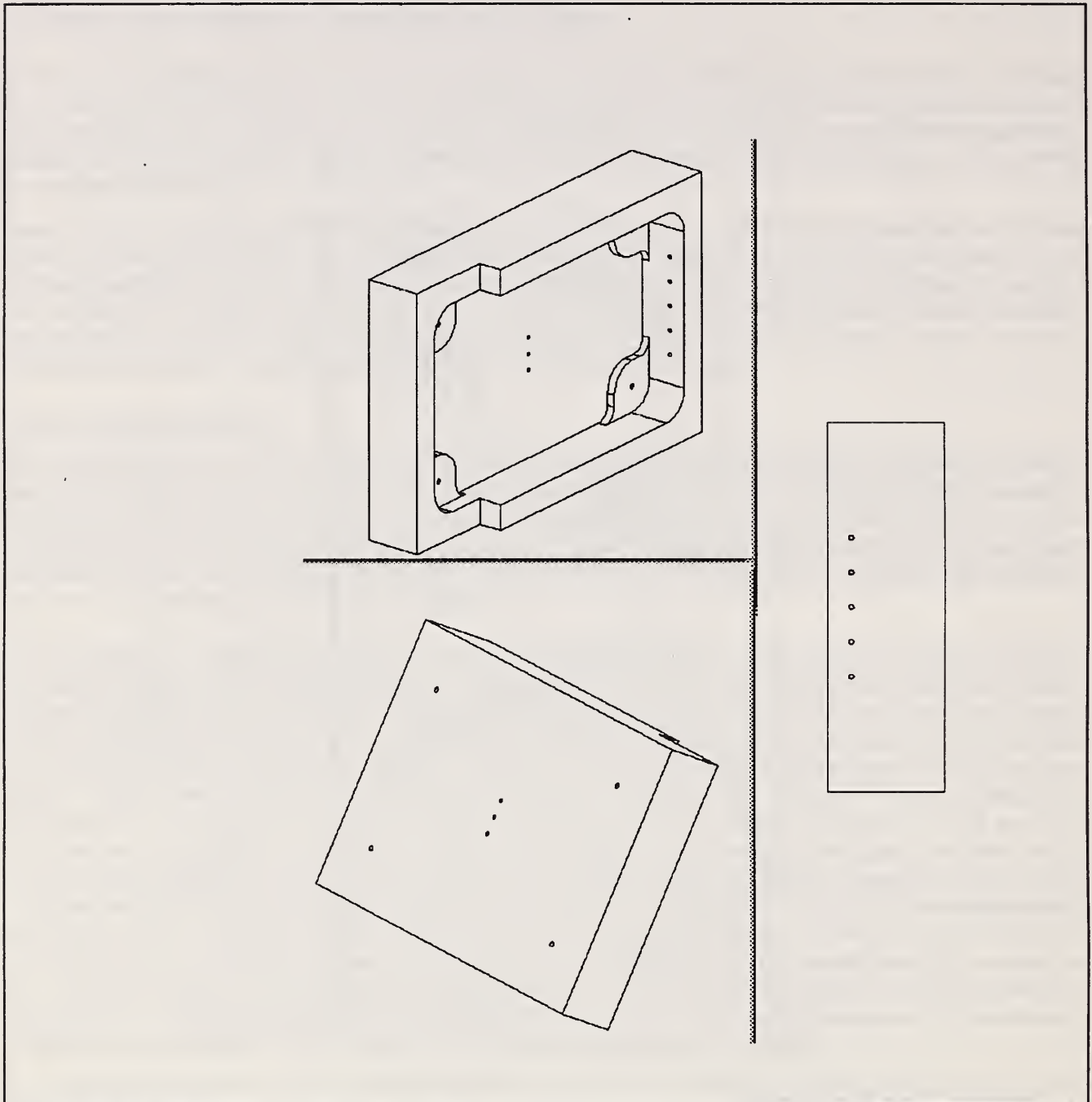
FIGURE 2. Indirectly Modified Blind Holes
