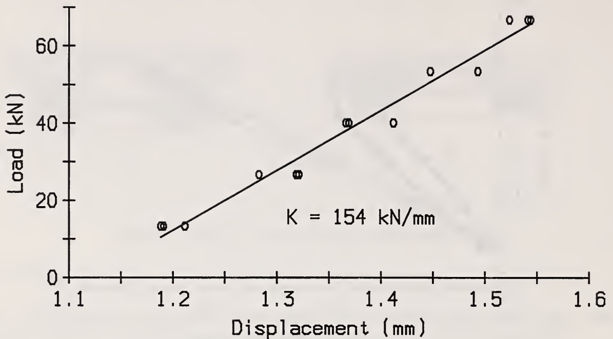
Figure 21. Stiffness measurement of prototype device dual-spring assembly.
