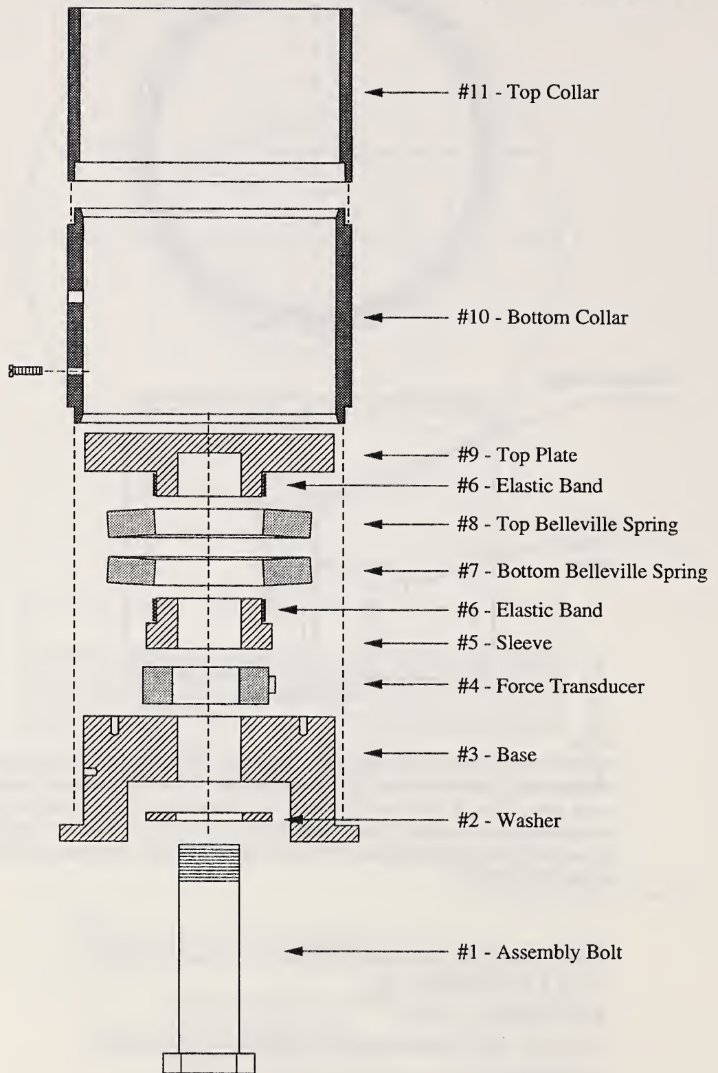
Figure 38. Assembly drawing.
