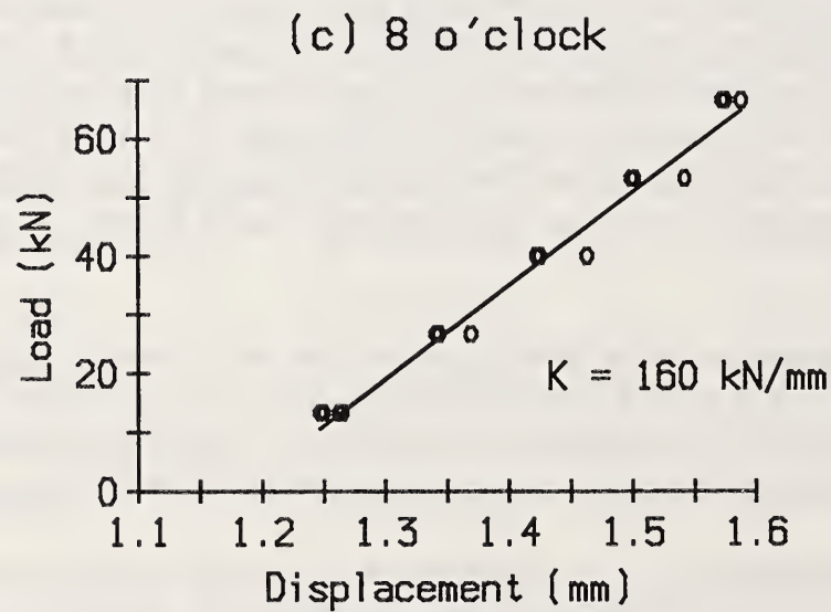
Figure 31. Stiffness of device measured in different orientations.
