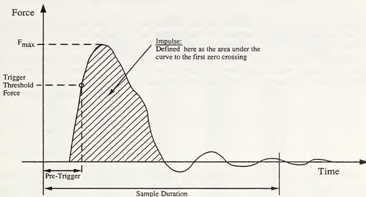
Figure 27. Typical force-time history.
