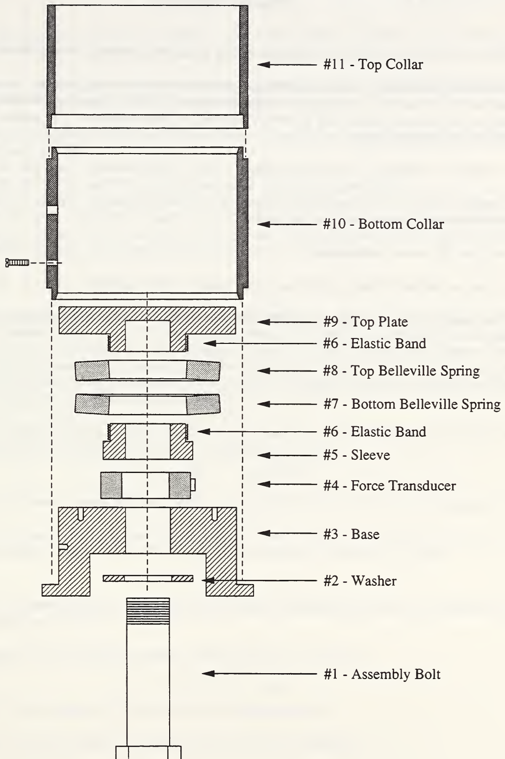
Figure A1.6: Assembly Drawing
