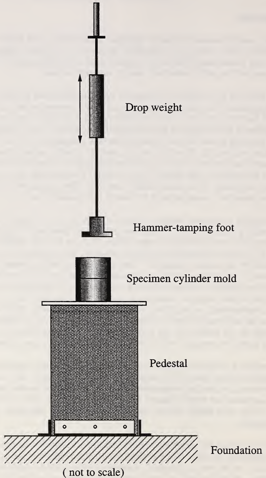
Figure 1. Marshall compaction hammer.
