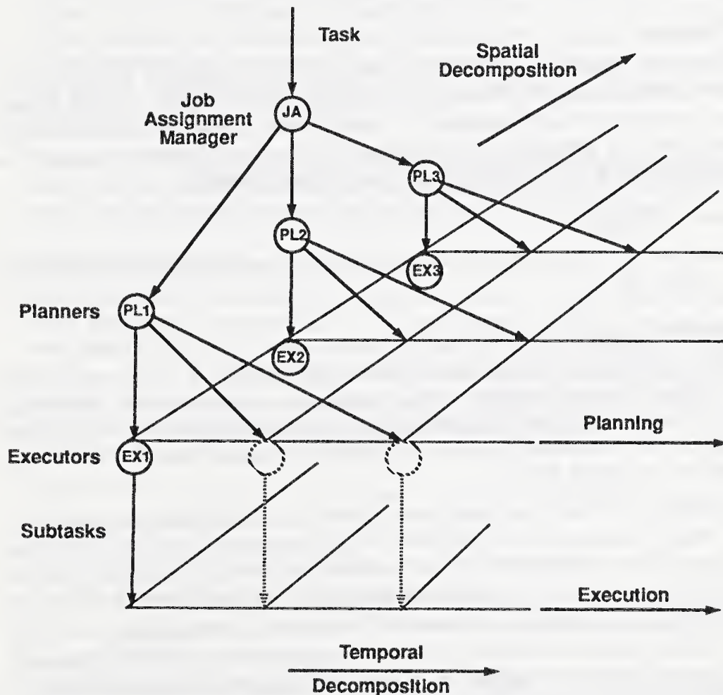
Figure 5. RCS Task Decomposition
