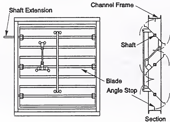
Figure 1. Multi-Blade Construction Used For Balancing, Control, Fire, and Smoke Dampers [adapted from SMACNA (1981)].
