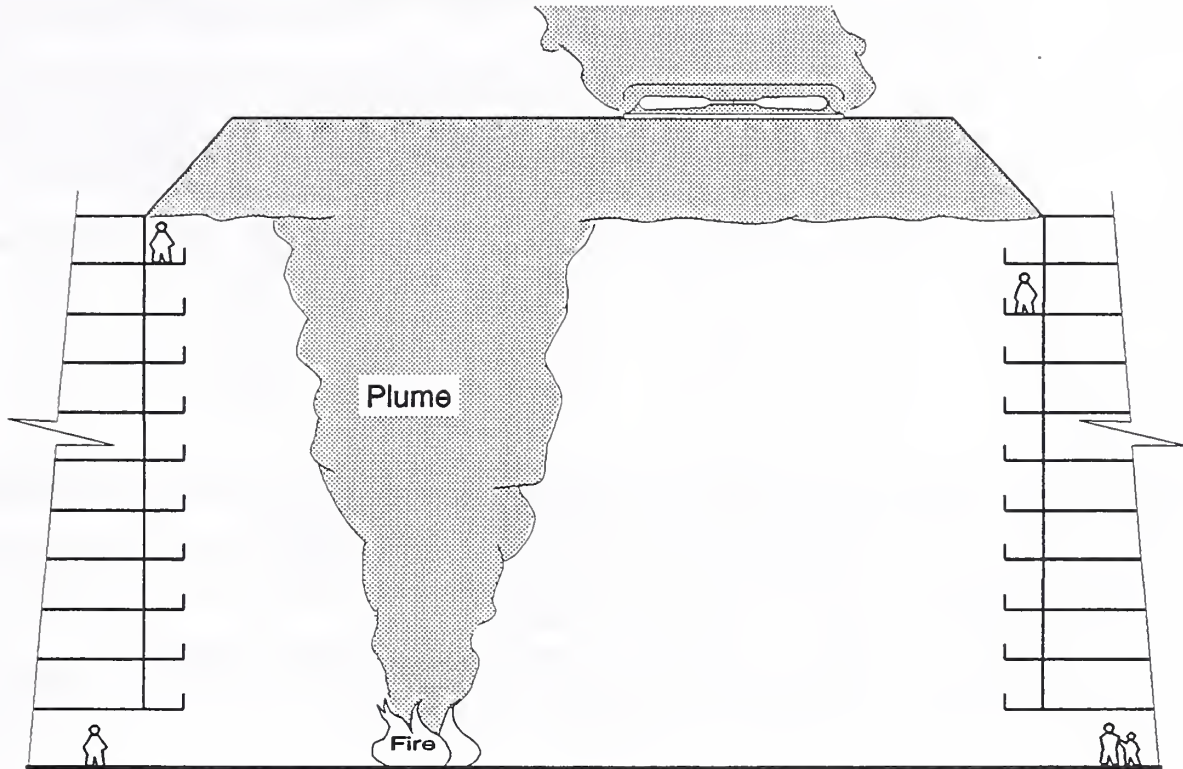
Figure 8. Atrium Smoke Exhaust System.
