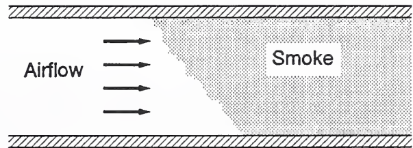
Figure 7. Critical Velocity to Prevent Smoke Backflow in a Corridor.
