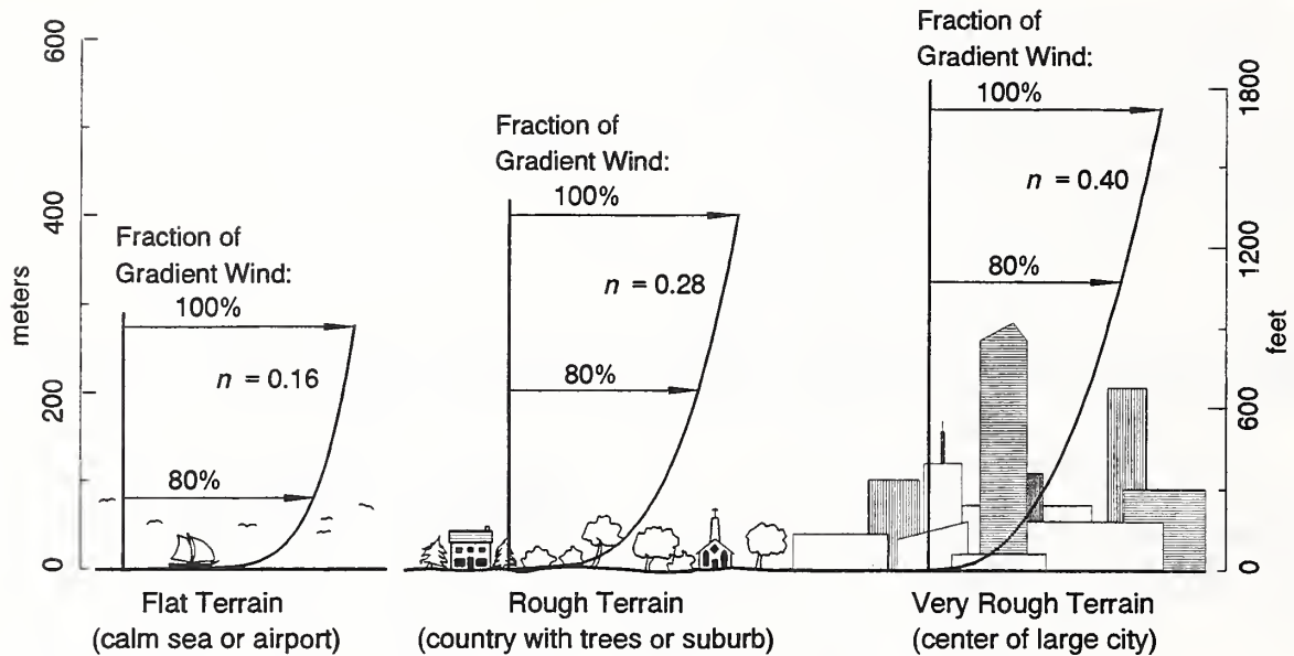
Figure 3. Wind velocity profiles for different terrain
