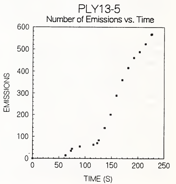
Figure 5. A comparison of AE events from duplicate samples of 13 mm thick plywood under identical operating conditions.
