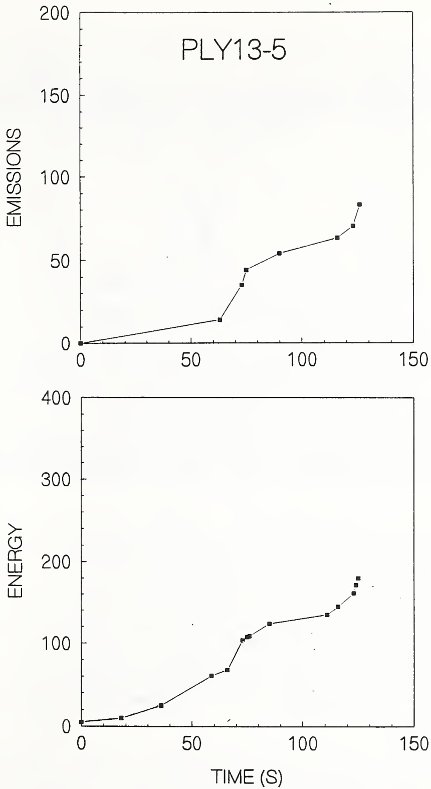
Figure 4. Number of emissions and cumulative energy from 13 mm thick plywood sample heated with 1.1 kW flame.
