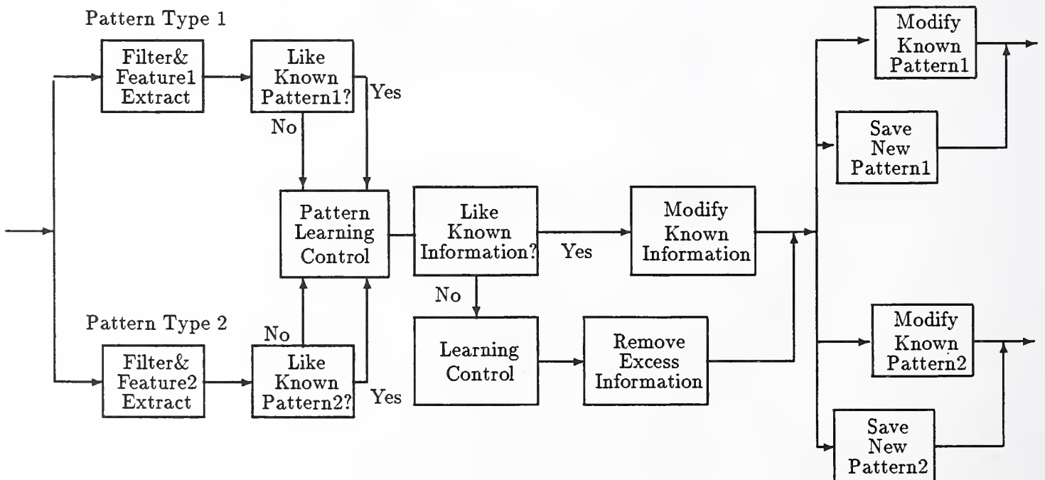
Figure 7: Data flow for size optimization in a multi-map network.
