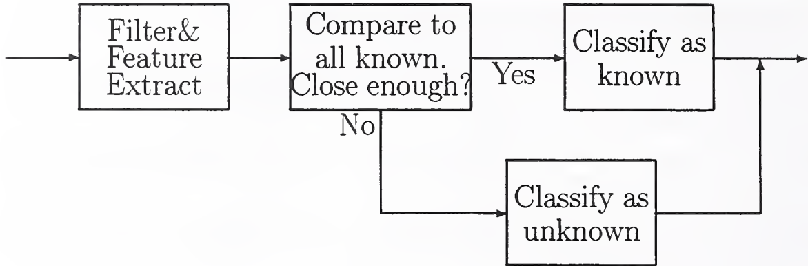
Figure 1: Data flow in a simple classification system.
