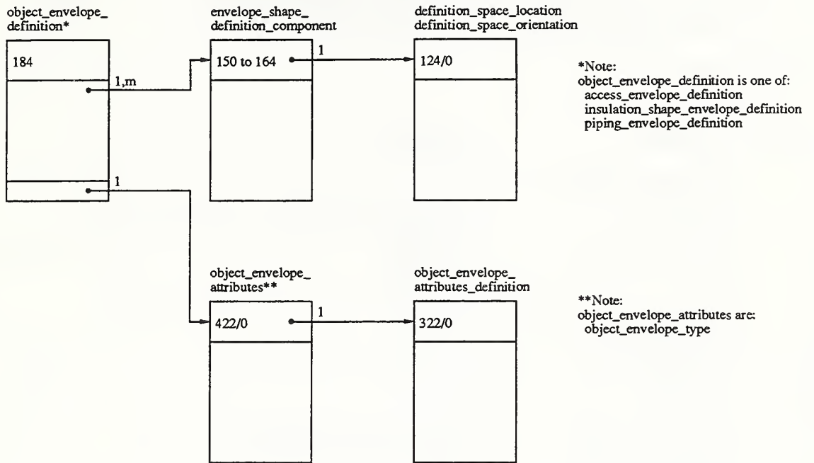
Figure 4-6. Object envelope definition and installed access envelope
