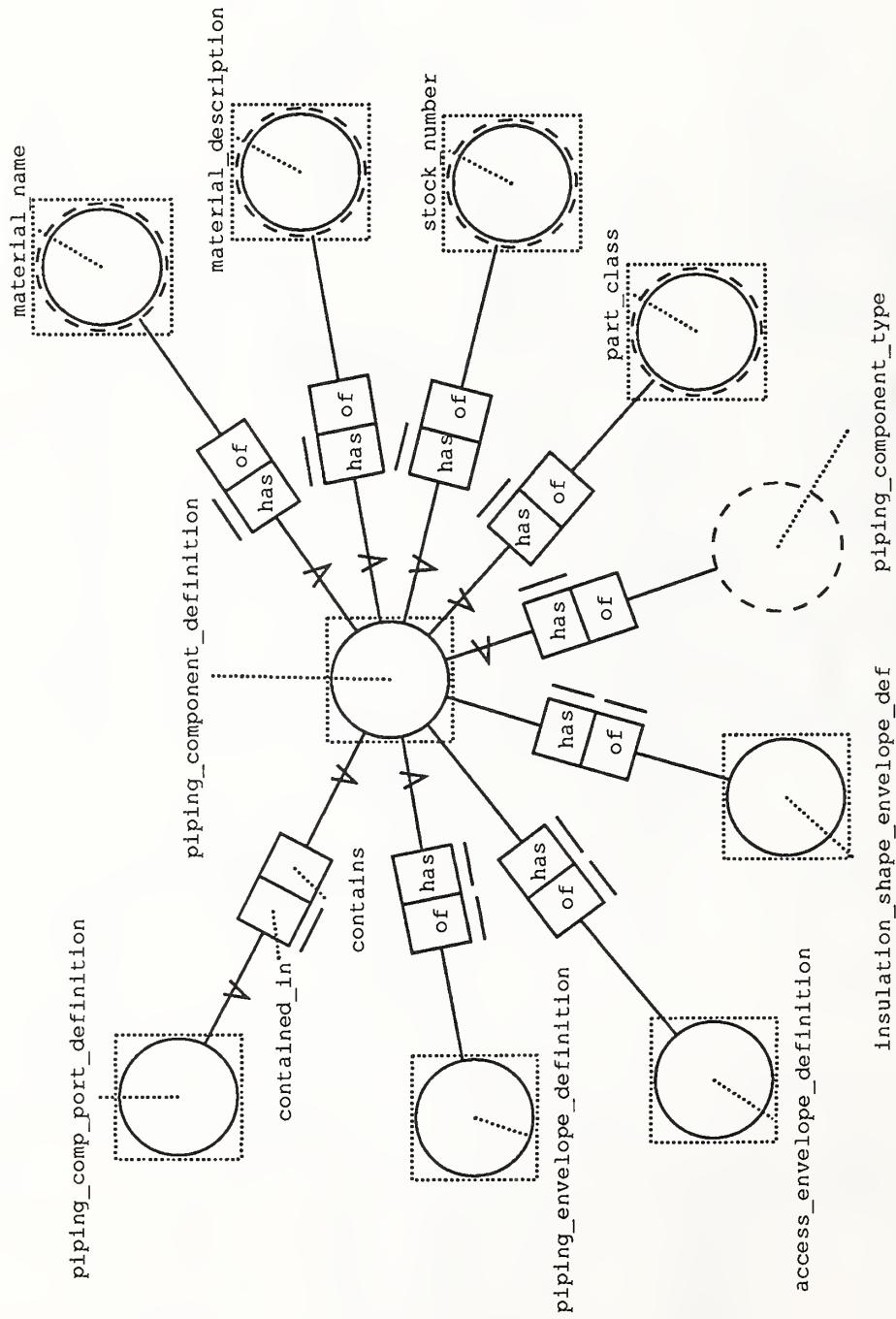
Figure 3-18. Piping component definition
