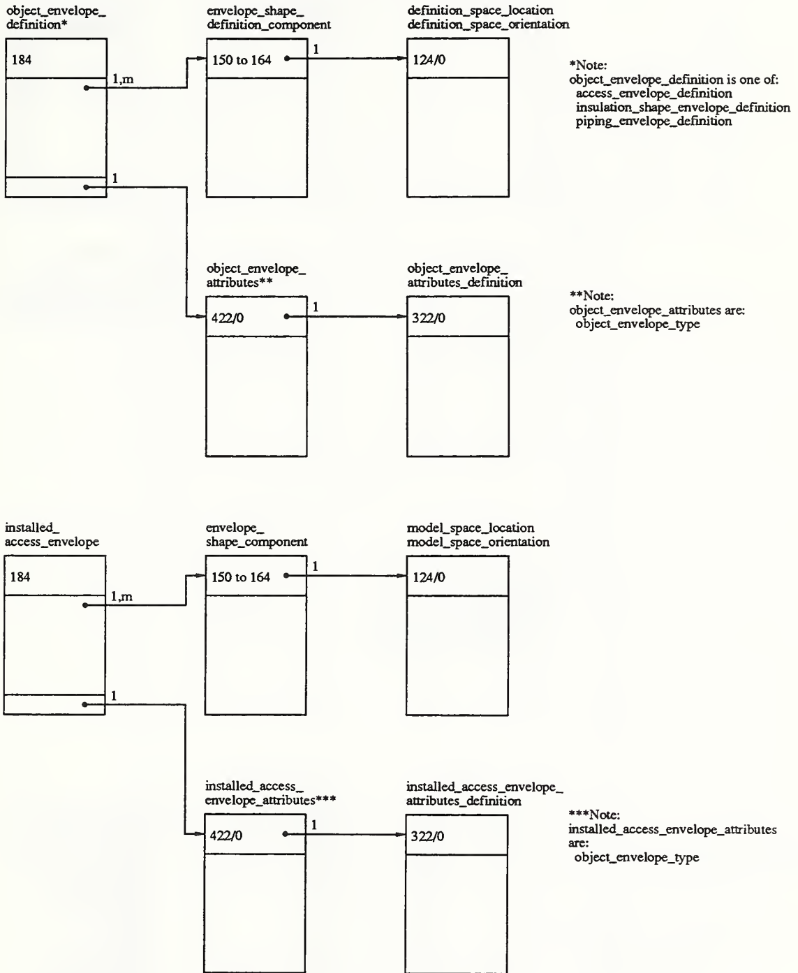
Figure E-6. Object envelope definition and installed access envelope
