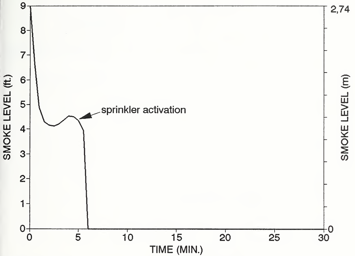
Figure 35. Smoke level in an individual room in Whipple Building
