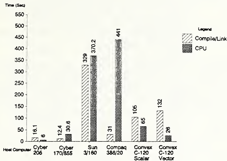
Figure 7. Timing benchmarks for CMMML computers.
