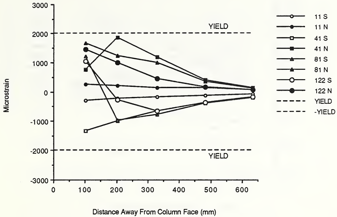
Fig. 3.43 Bottom northeast reinforcing bar strains - E-P-Z4.
