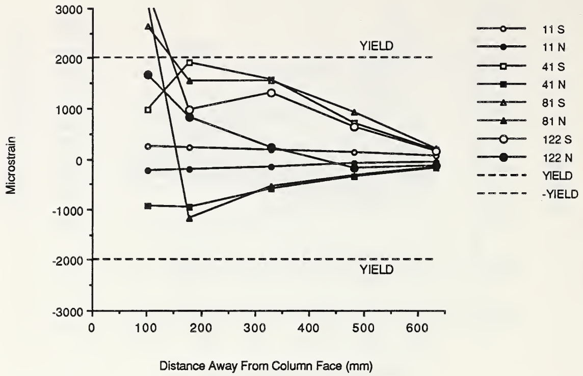
Fig. 3.49 Bottom southwest reinforcing bar strains - E-P-Z4.
