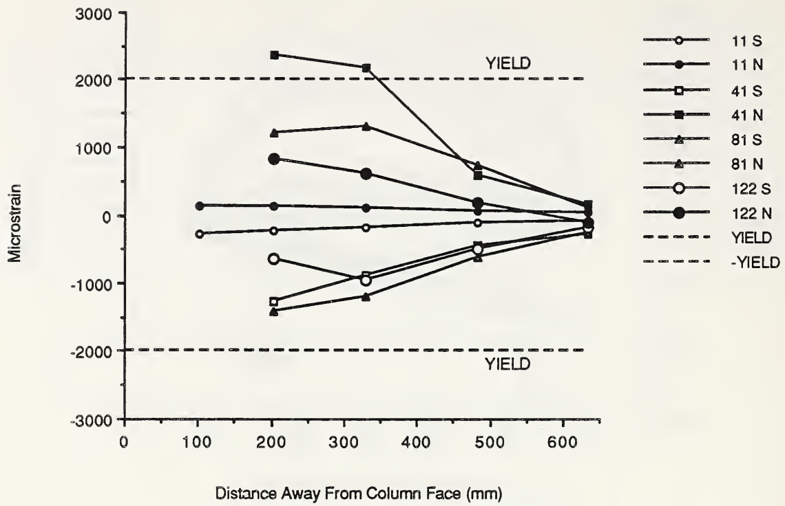
Fig. 3.27 Top southeast reinforcing bar strains - D-P-Z4.
