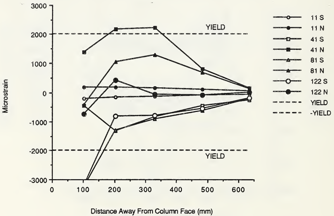
Fig. 3.24 Bottom northeast reinforcing bar strains - D-P-Z4.
