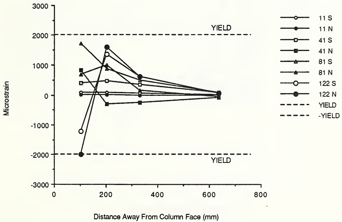
Fig. 3.52 Top northwest reinforcing bar strains - F-P-Z4.
