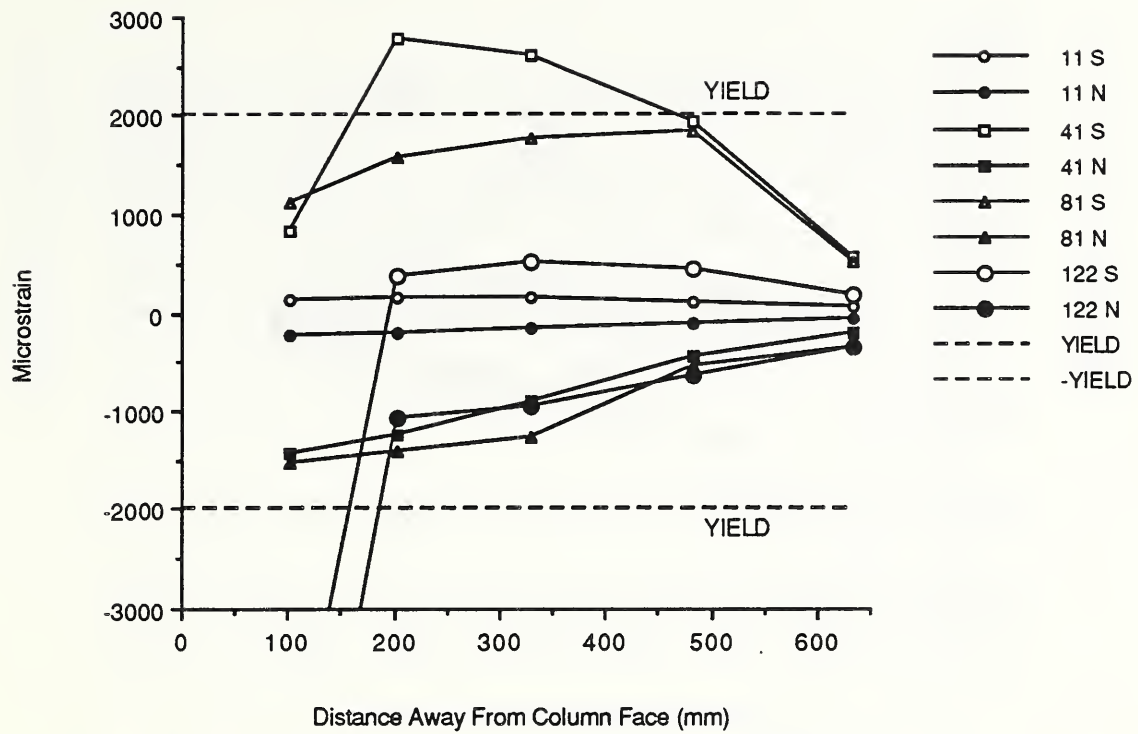
Fig. 3.25 Top northwest reinforcing bar strains - D-P-Z4.
