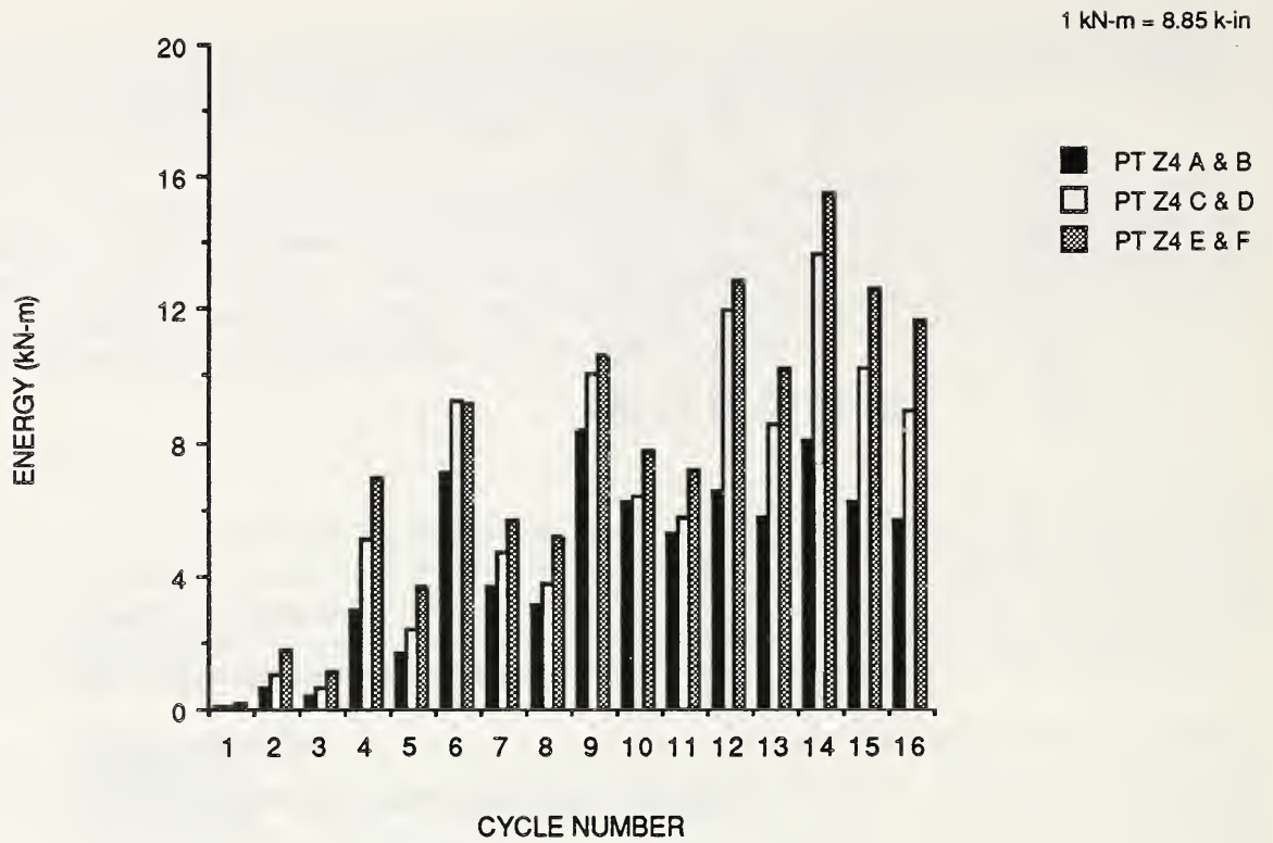
Fig. 4.2 Cyclic energy absorbed by precast Zone 4 specimens.
