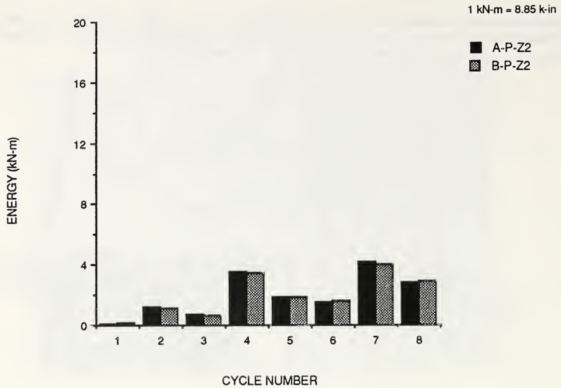
Fig. 3.66 Energy absorbed by specimens A-P-Z2 and B-P-Z2.
