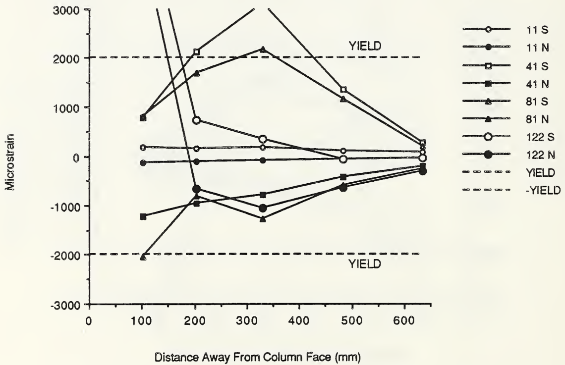
Fig. 3.28 Bottom southeast reinforcing bar strains - D-P-Z4.
