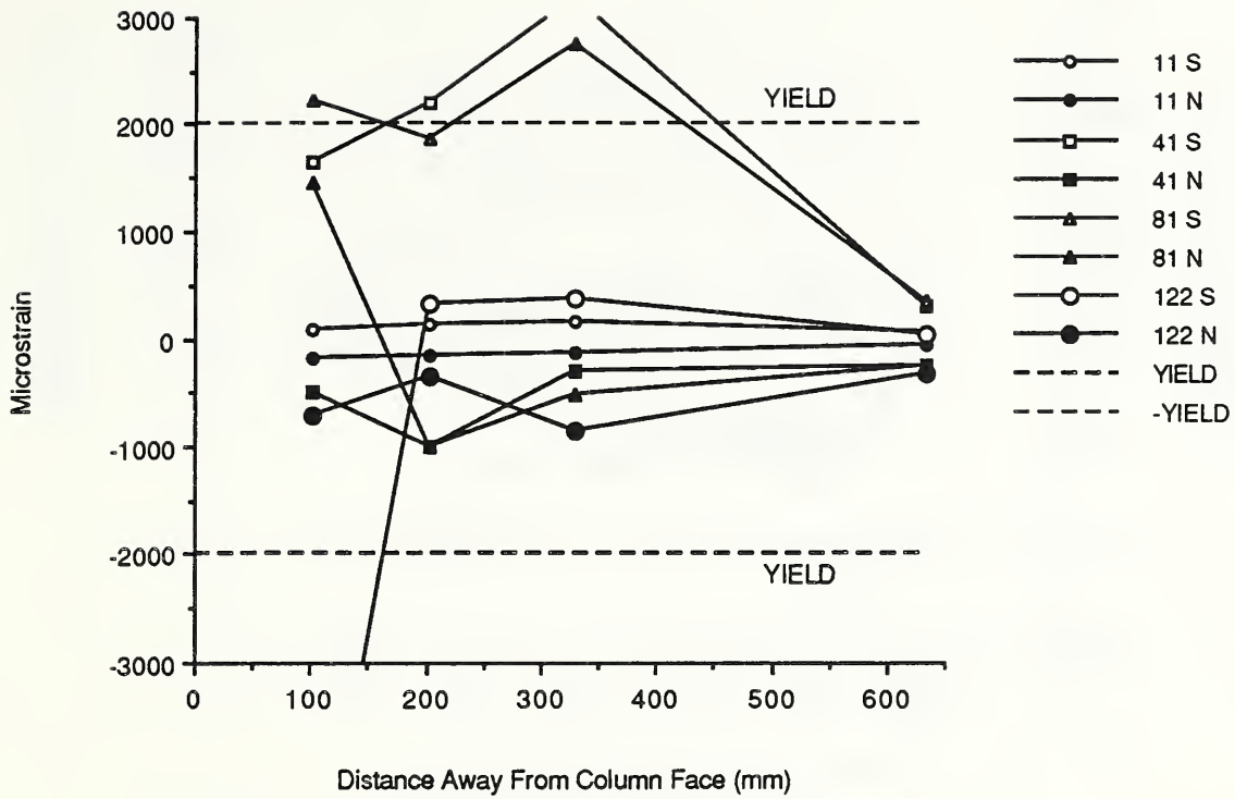
Fig. 3.17 Top northwest reinforcing bar strains - C-P-Z4.
