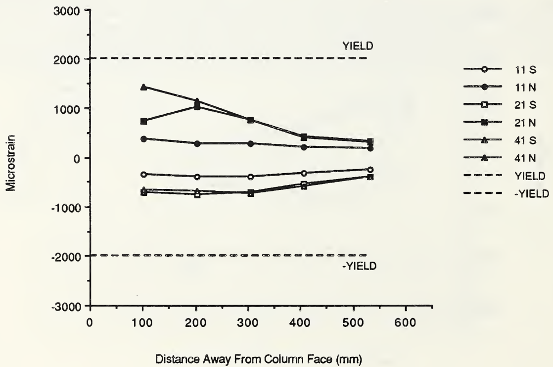
Fig. 3.70 Bottom northwest reinforcing bars strains - A-P-Z2.
