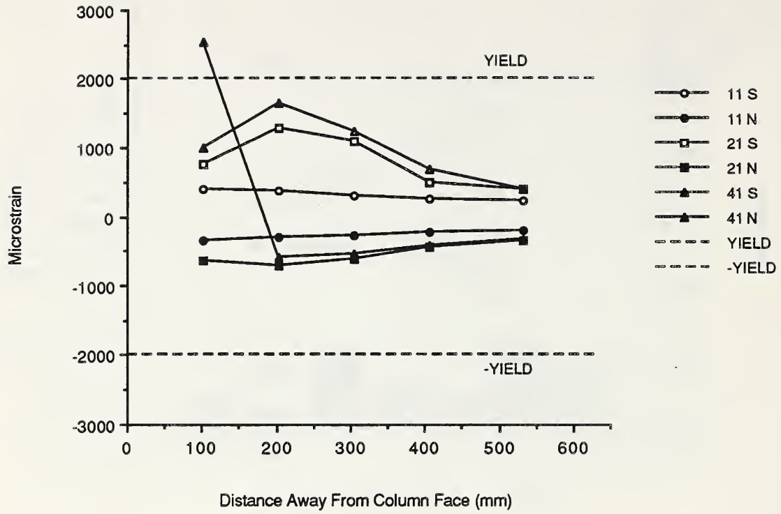
Fig. 3.69 Top northwest reinforcing bar strains - A-P-Z2.
