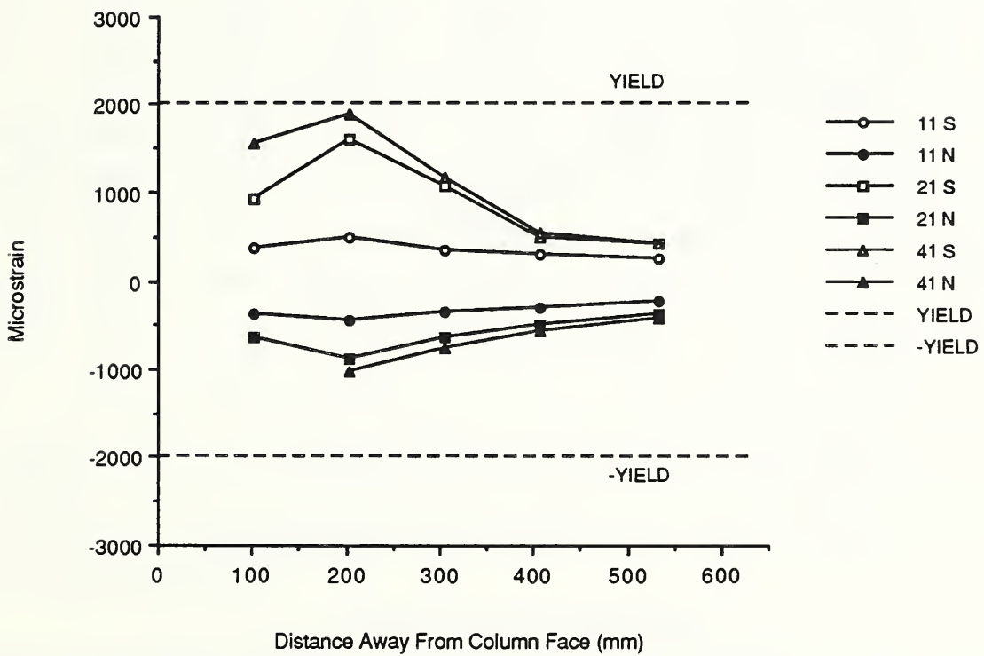
Fig. 3.80 Bottom southeast reinforcing bar strains - B-P-Z2.
