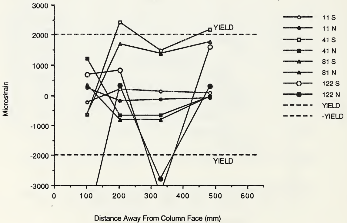
Fig. 3.20 Bottom southeast reinforcing bar strains - C-P-Z4.
