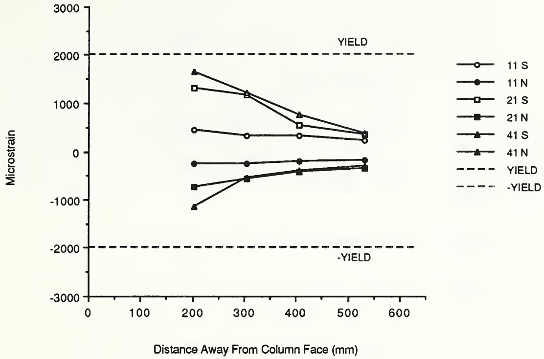
Fig. 3.67 Top northeast reinforcing bar strains - A-P-Z2.
