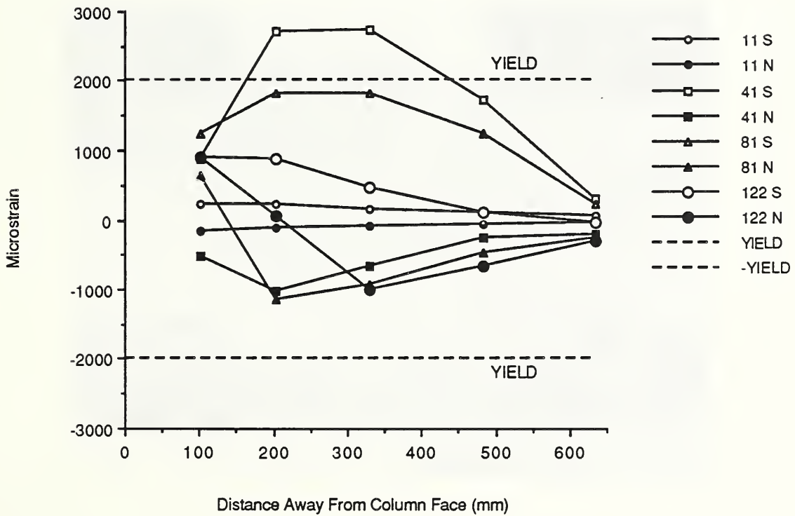
Fig. 3.30 Bottom southwest reinforcing bar strains - D-P-Z4.
