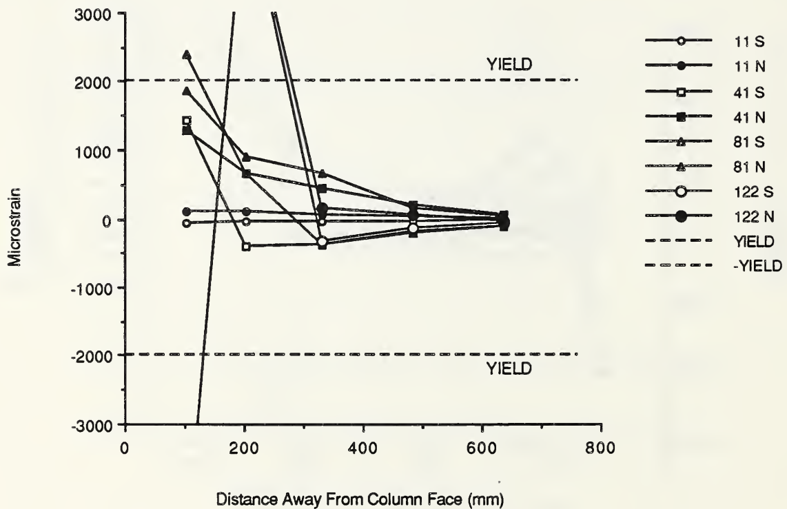
Fig. 3.54 Top southeast reinforcing bar strains - F-P-Z4.
