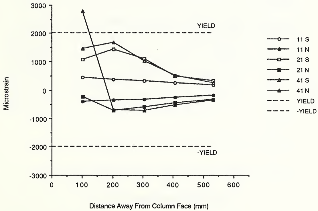
Fig. 3.72 Bottom southeast reinforcing bar strains - A-P-Z2.
