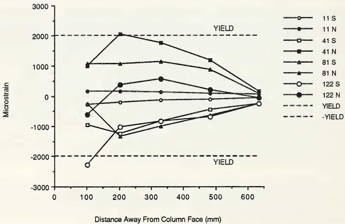
Fig. 3.16 Bottom northeast reinforcing bar strains - C-P-Z4.
