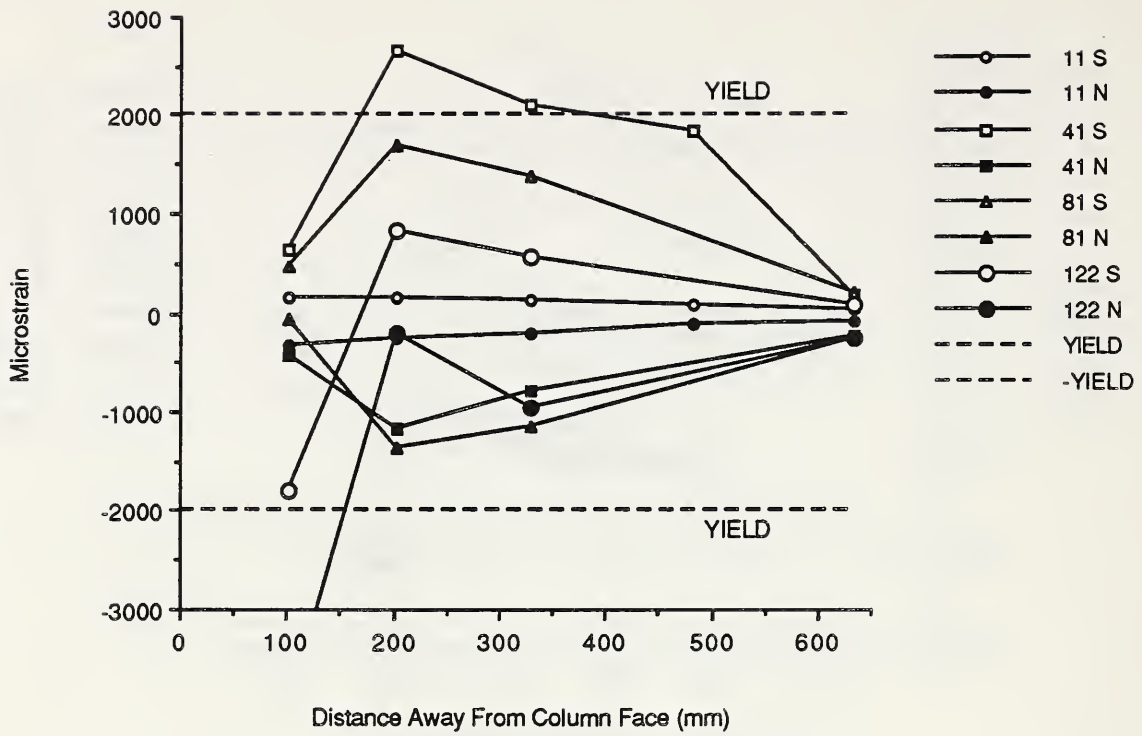
Fig. 3.23 Top northeast reinforcing bar strain - D-P-Z4.
