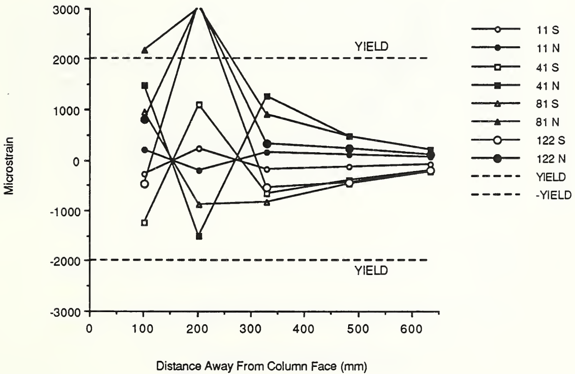
Fig. 3.48 Top southwest reinforcing bar strains - E-P-Z4.
