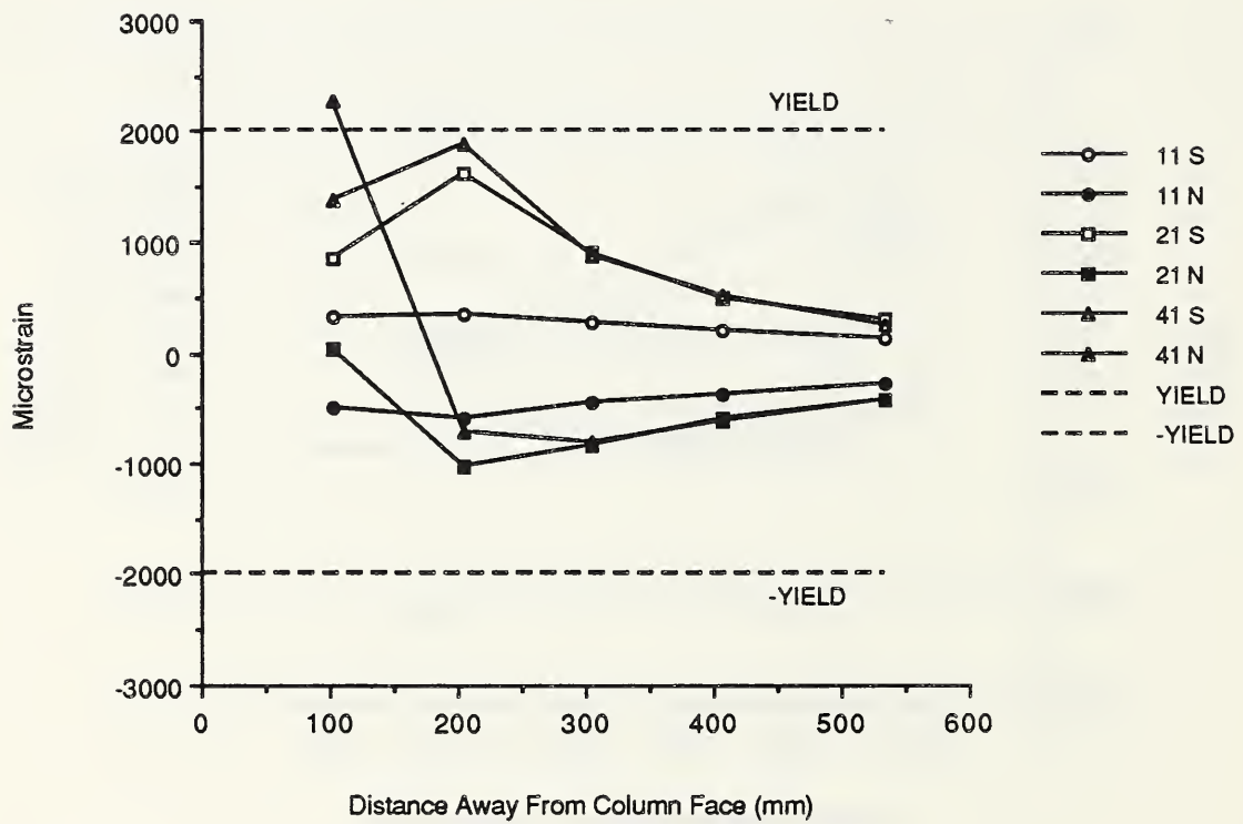
Fig. 3.74 Bottom southwest reinforcing bars strains - A-P-Z2.
