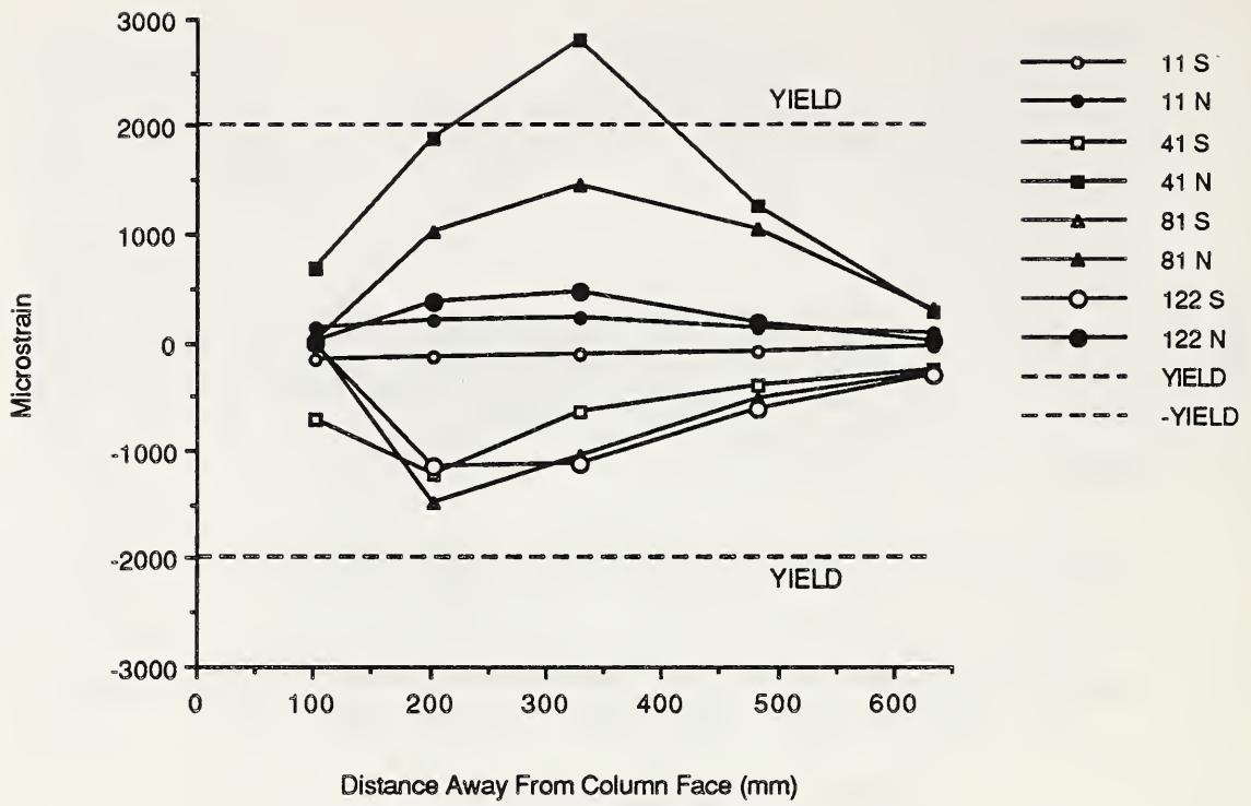
Fig. 3.19 Top southeast reinforcing bar strains - C-P-Z4.
