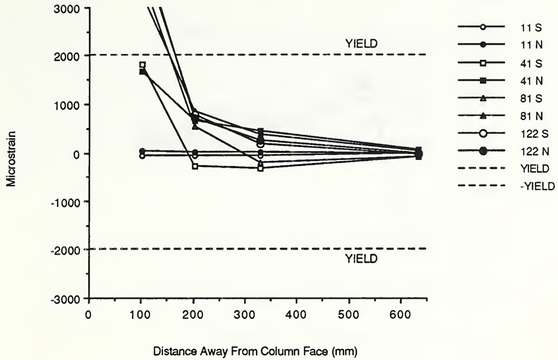
Fig. 3.51 Bottom northeast reinforcing bar strains - F-P-Z4.
