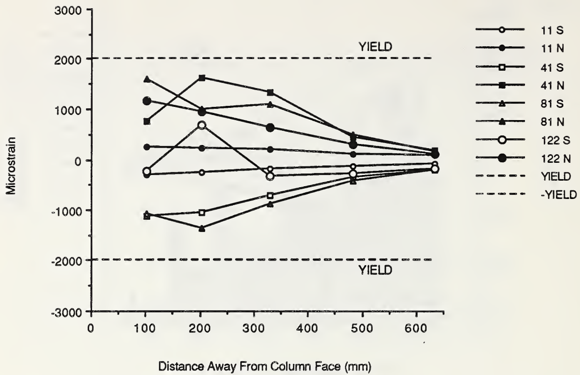
Fig. 3.45 Bottom northwest reinforcing bar strains - E-P-Z4.
