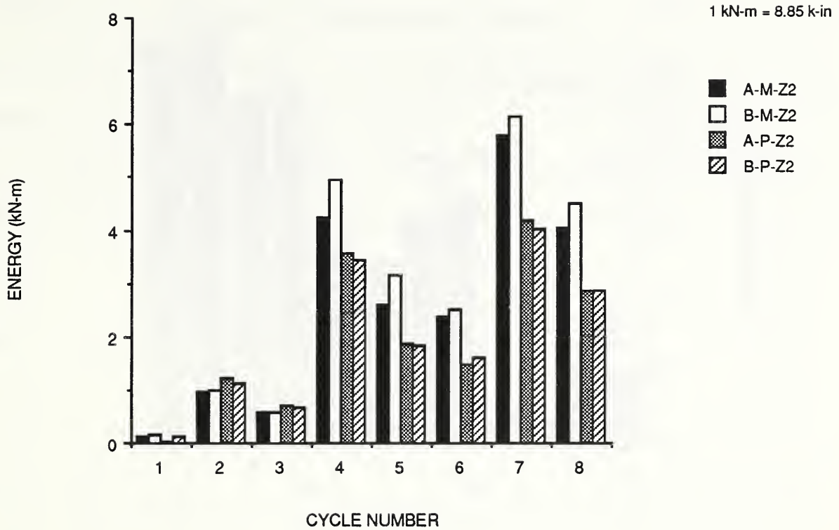
Fig. 4.3 Cyclic energy absorbed by Zone 2 specimens.
