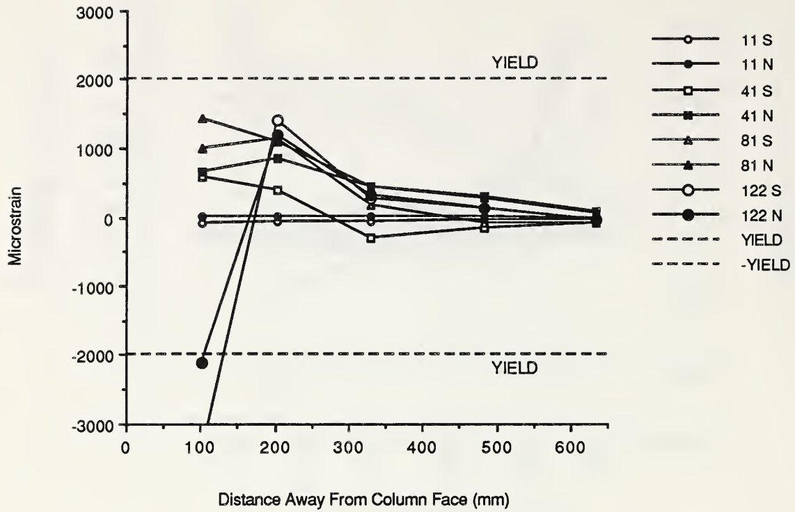
Fig. 3.53 Bottom northwest reinforcing bar strains - F-P-Z4.
