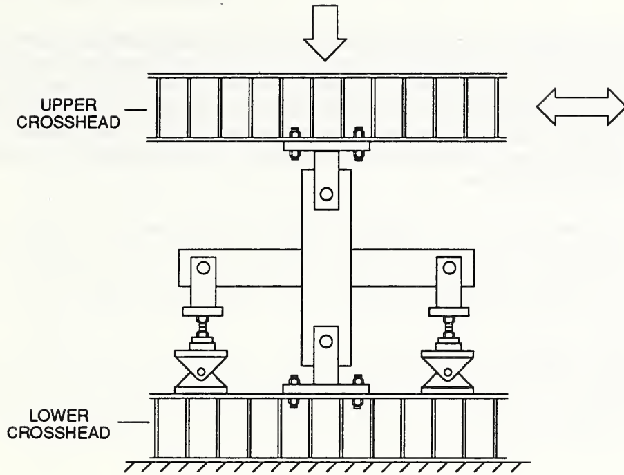
Fig. 2.7 Boundary conditions for the test specimens.
