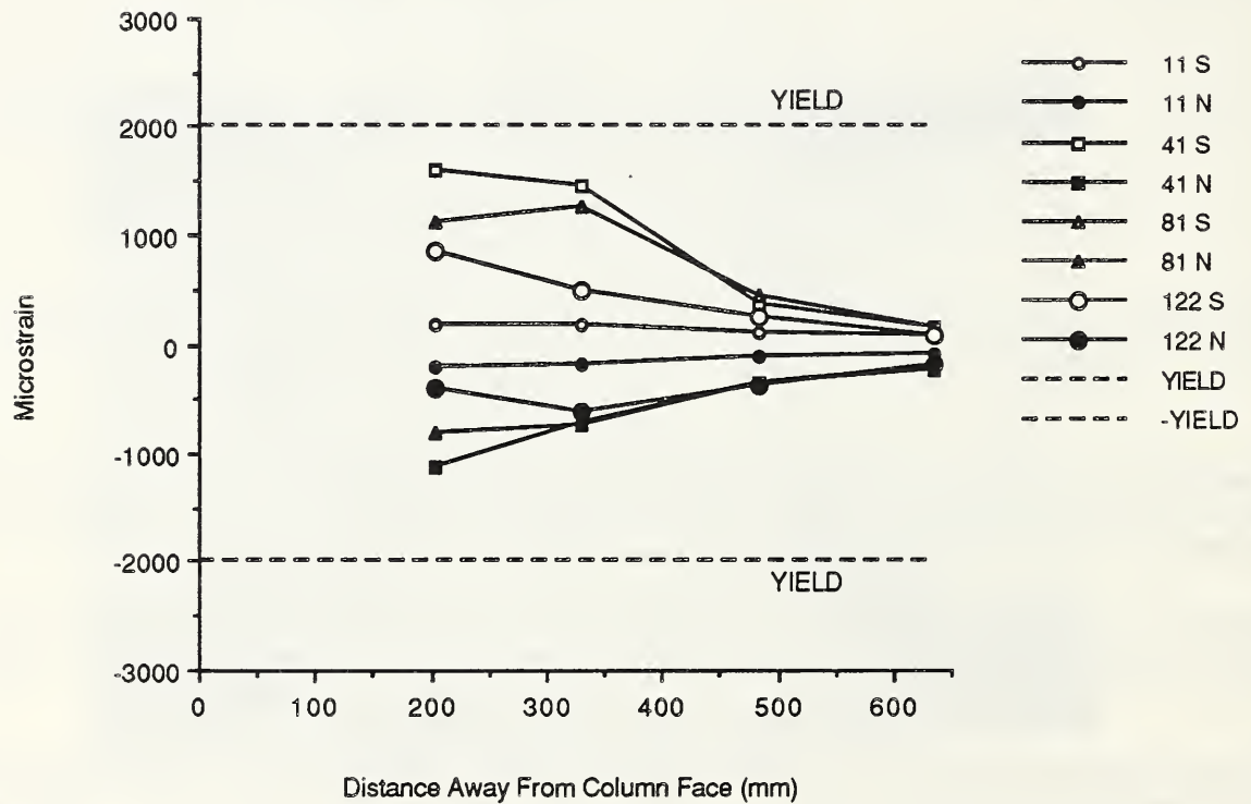
Fig. 3.42 Top northeast reinforcing bar strains - E-P-Z4.
