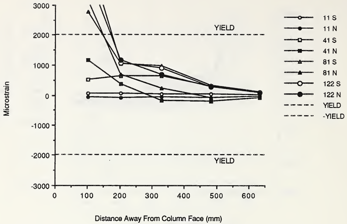
Fig. 3.57 Bottom southwest reinforcing bar strains - F-P-Z4.
