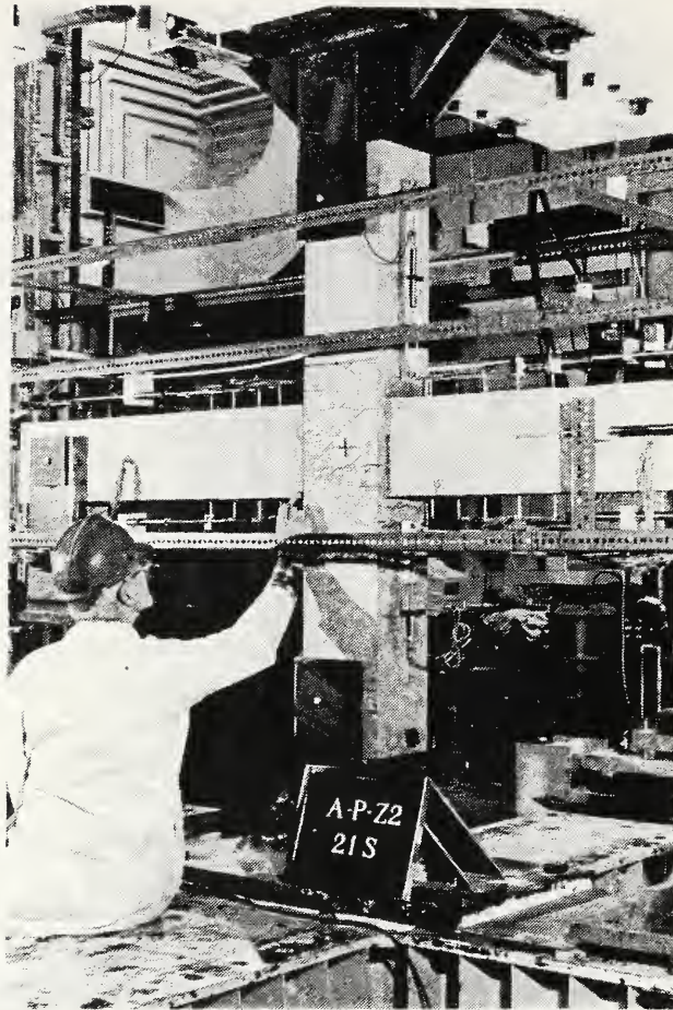
Fig. 3.59 Crack pattern at 2 \Delta_y - A-P-Z2.
