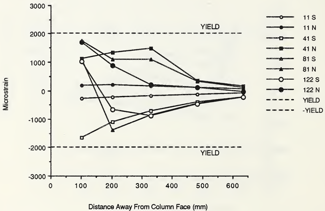
Fig. 3.46 Top southeast reinforcing bar strains - E-P-Z4.
