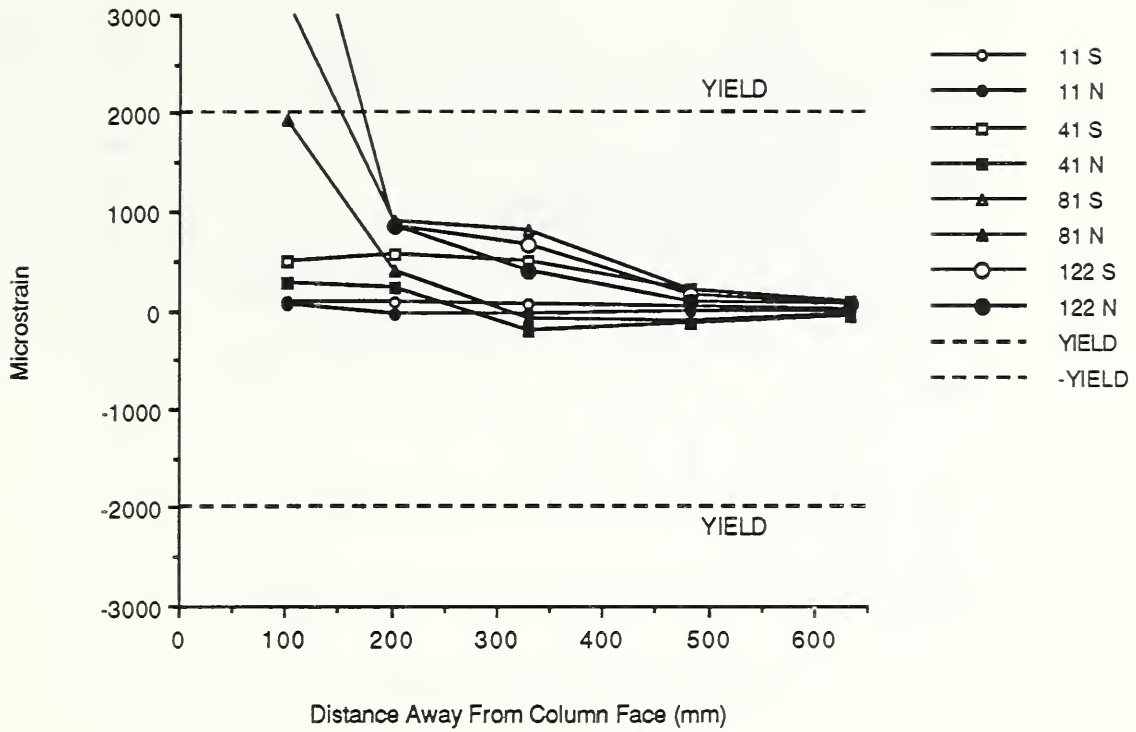
Fig. 3.55 Bottom southeast reinforcing bar strains - F-P-Z4.
