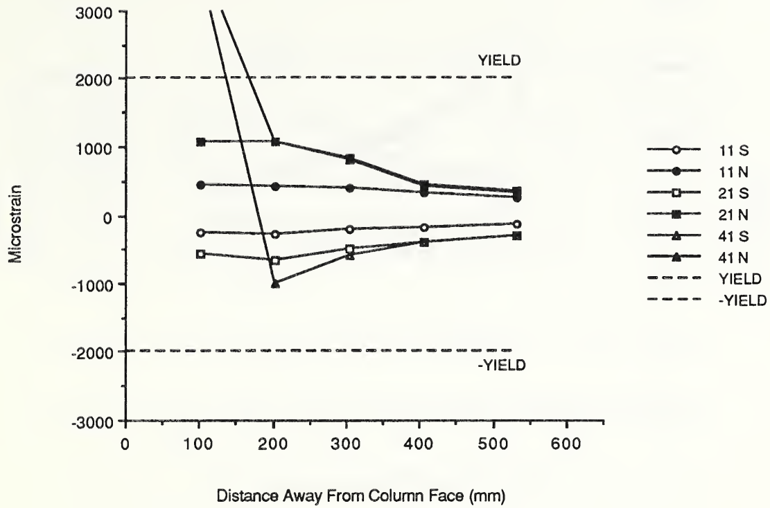
Fig. 3.71 Top southeast reinforcing bar strains - A-P-Z2.
