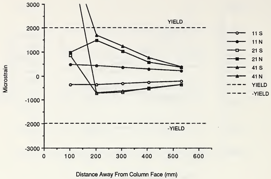
Fig. 3.81 Top southwest reinforcing bar strains - B-P-Z2.
