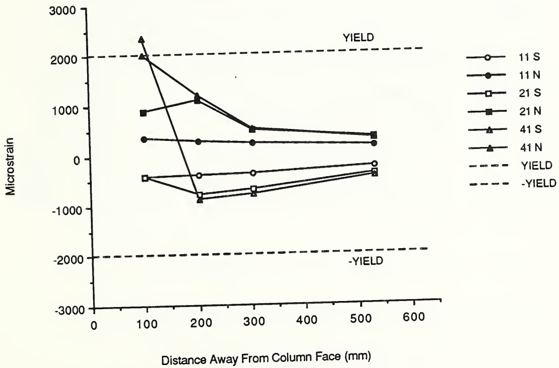
Fig. 3.76 Bottom northeast reinforcing bar strains - B-P-Z2.
