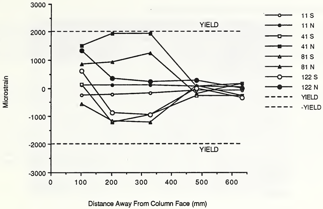
Fig. 3.29 Top southwest reinforcing bar strains - D-P-Z4.
