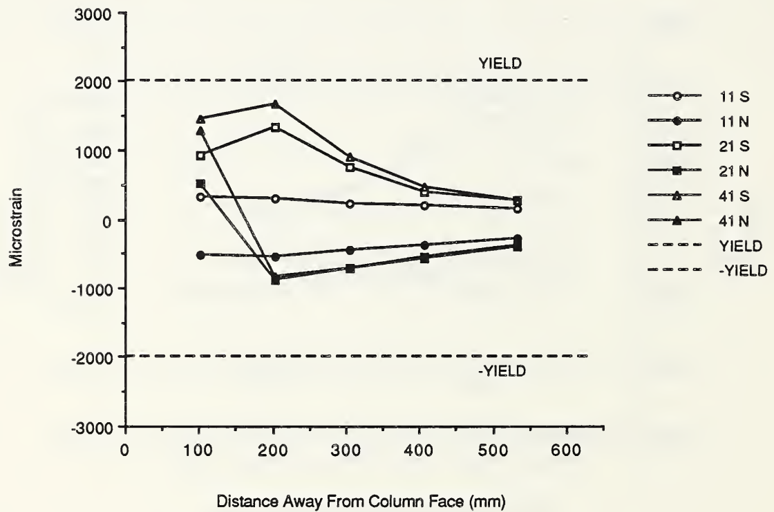
Fig. 3.82 Bottom southwest reinforcing bar strains - B-P-Z2.
