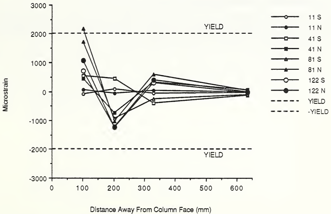
Fig. 3.56 Top southwest reinforcing bar strains - F-P-Z4.
