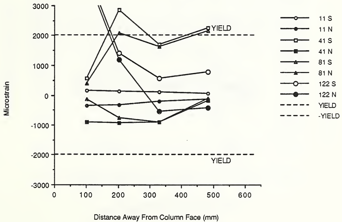
Fig. 3.22 Bottom southwest reinforcing bar strains - C-P-Z4.
