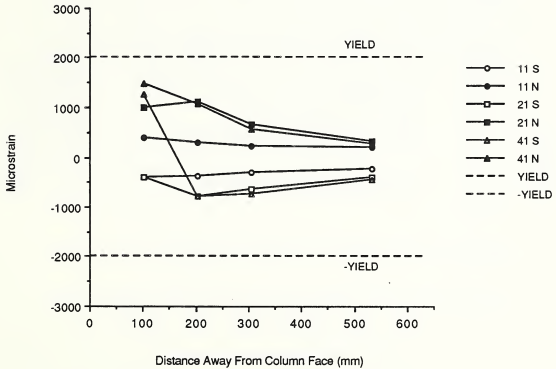
Fig. 3.68 Bottom northeast reinforcing bar strains - A-P-Z2.
