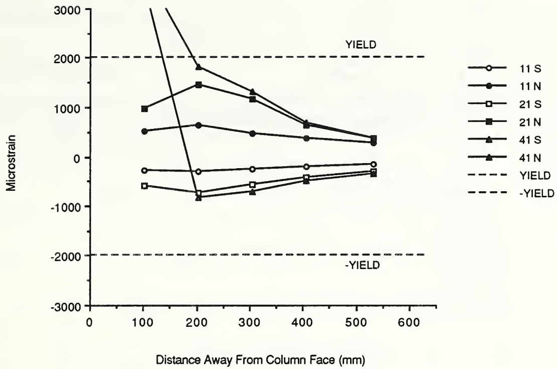
Fig. 3.79 Top southeast reinforcing bar strains - B-P-Z2.
