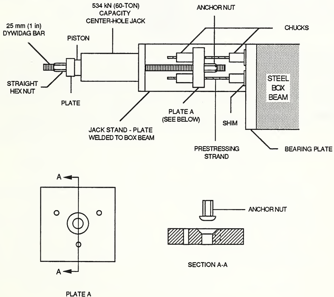
Fig. 2.5 Jacking assembly for precast concrete Zone 4 specimens.
