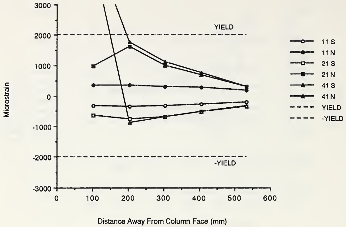
Fig. 3.73 Top southwest reinforcing bar strains - A-P-Z2.
