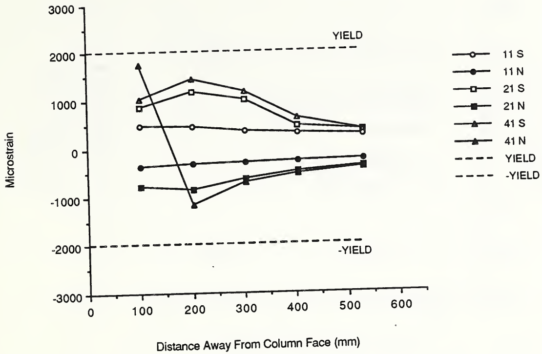
Fig. 3.75 Top northeast reinforcing bar strains - B-P-Z2.
