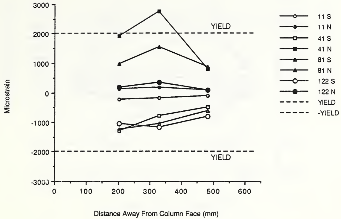
Fig. 3.21 Top southwest reinforcing bar strains - C-P-Z4.
