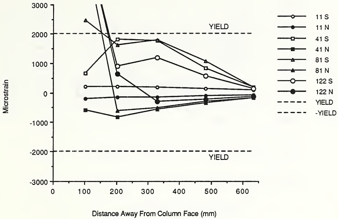
Fig. 3.47 Bottom southeast reinforcing bar strains - E-P-Z4.
