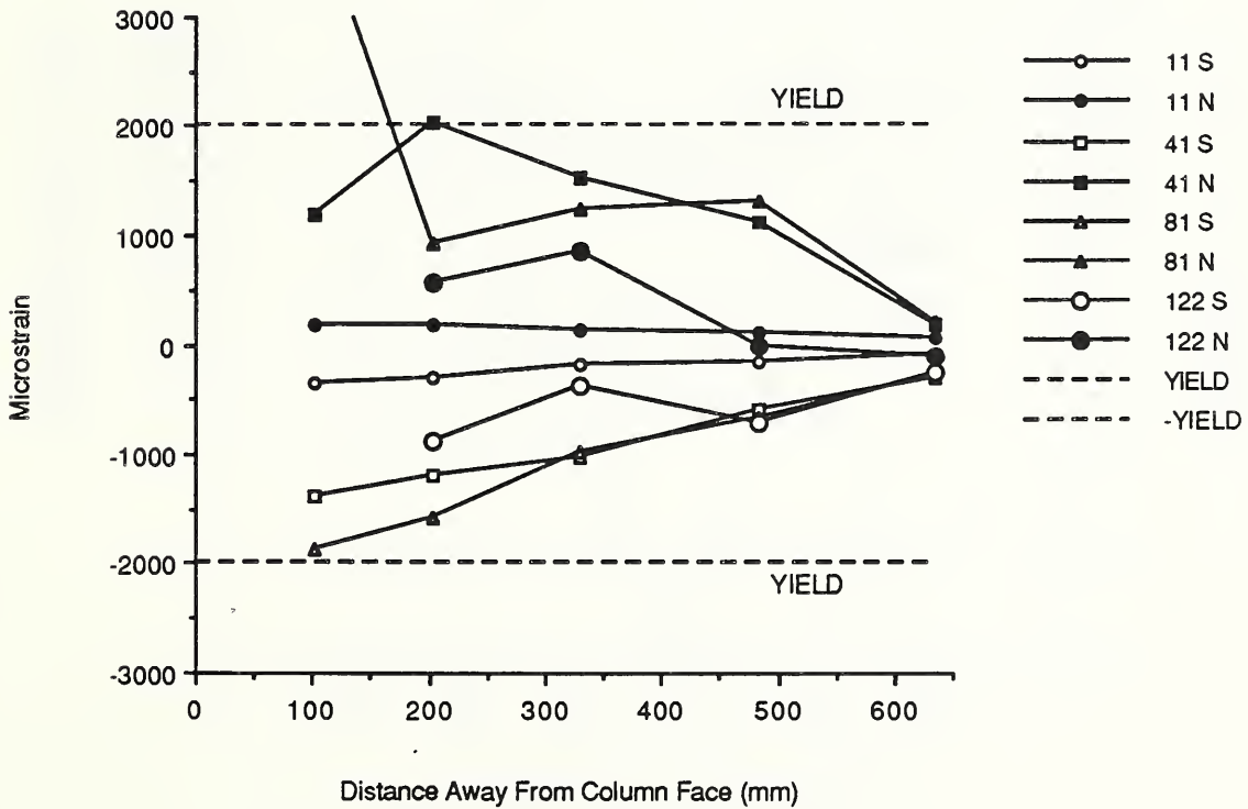
Fig. 3.18 Bottom northwest reinforcing bar strains - C-P-Z4.
