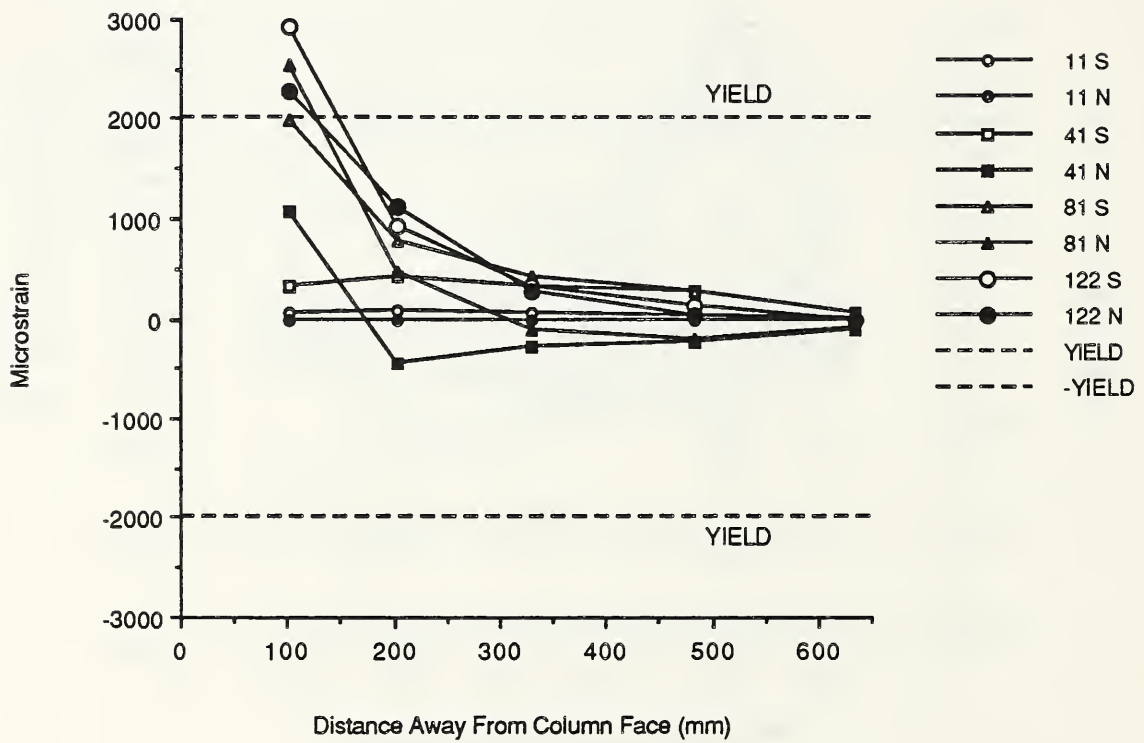
Fig. 3.50 Top northeast reinforcing bar strains - F-P-Z4.
