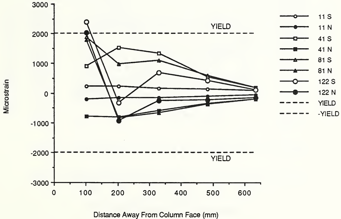
Fig. 3.44 Top northwest reinforcing bar strains - E-P-Z4.
