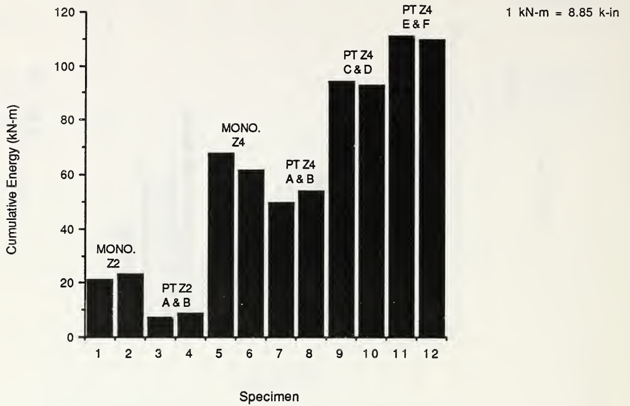
Fig. 4.4 Comparison of the cumulative energy absorbed.
