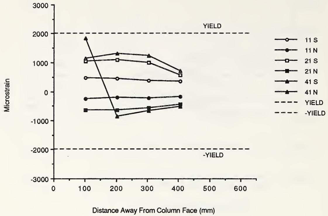
Fig. 3.77 Top northwest reinforcing bars strains - B-P-Z2.
