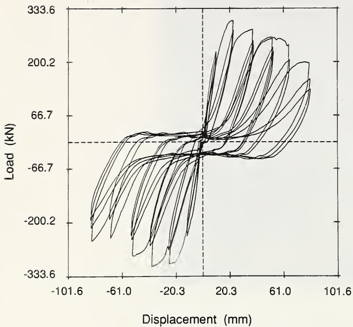
Fig. 3.12 Hysteresis curves for C-P-Z4.
