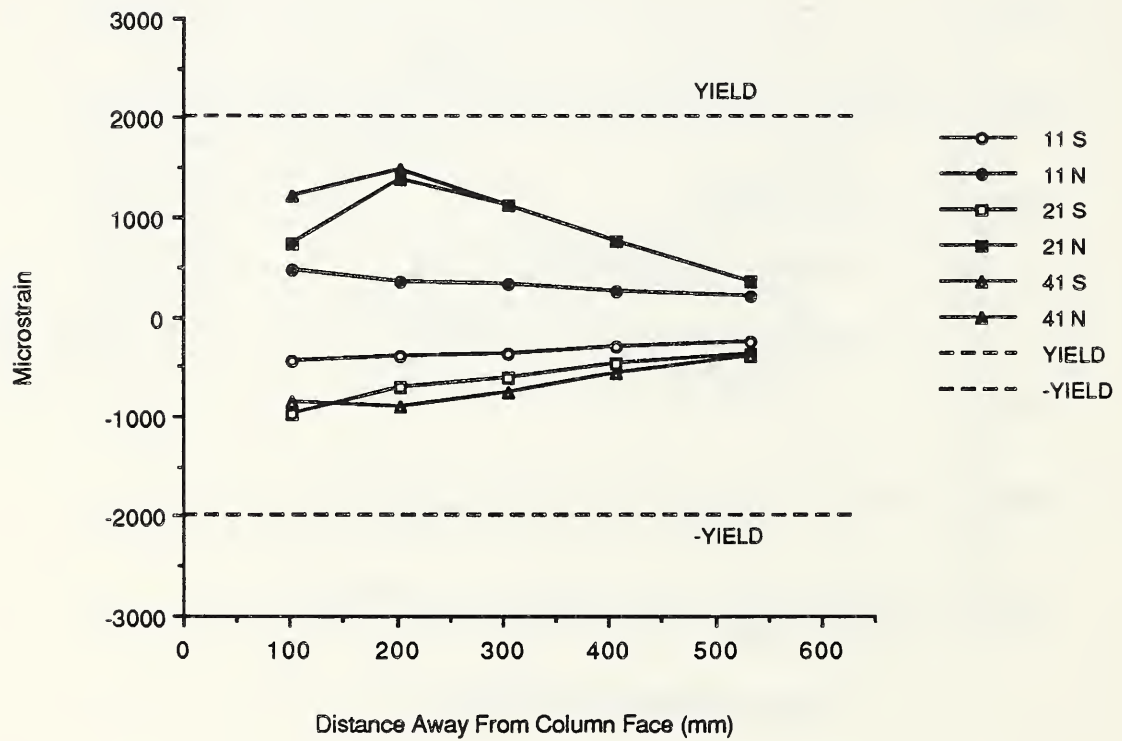
Fig. 3.78 Bottom northwest reinforcing bar strains - B-P-Z2.
