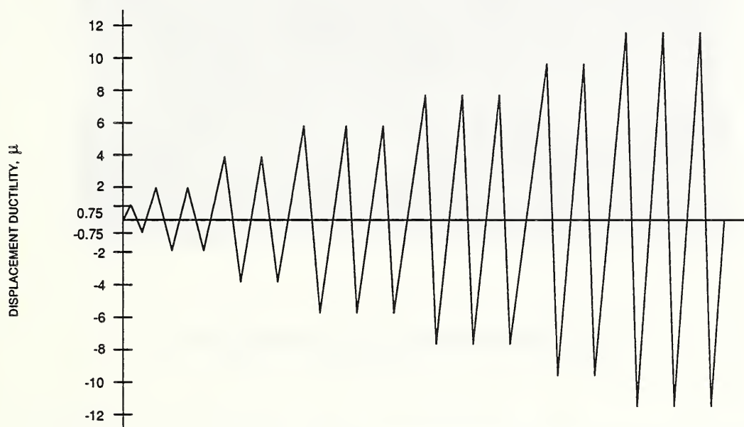
Fig. 3.1 Loading sequence for specimens C-P-Z4 through F-P-Z4.
