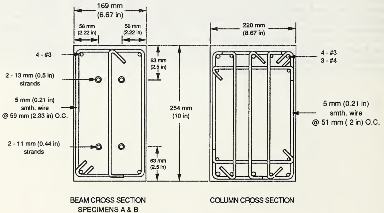
Fig. 2.2 Reinforcement details for precast concrete Zone 2 specimens.
