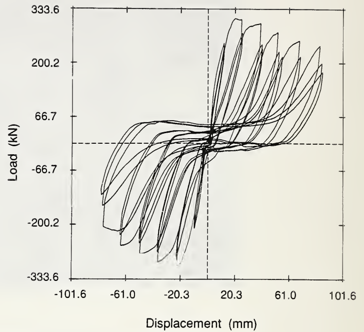
Fig. 3.13 Hysteresis curves for D-P-Z4.
