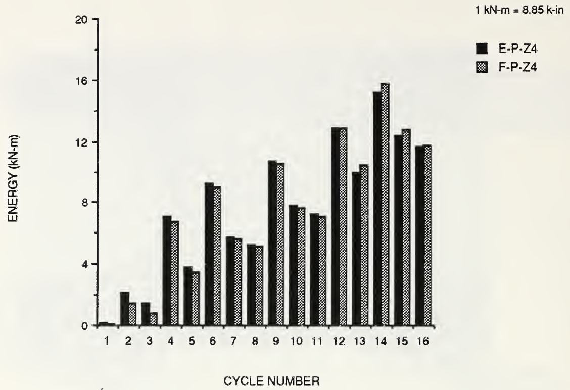
Fig. 3.41 Energy absorbed by specimens E-P-Z4 and F-P-Z4.
