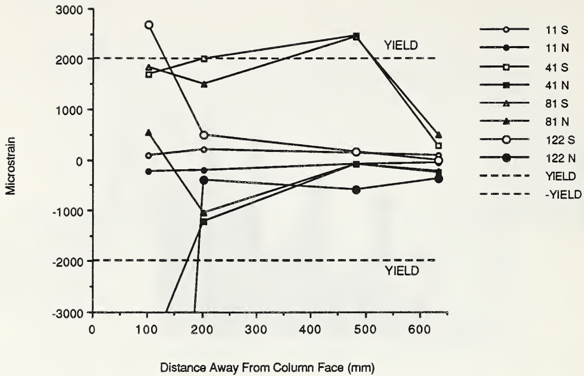
Fig. 3.15 Top northeast reinforcing bar strains - C-P-Z4.
