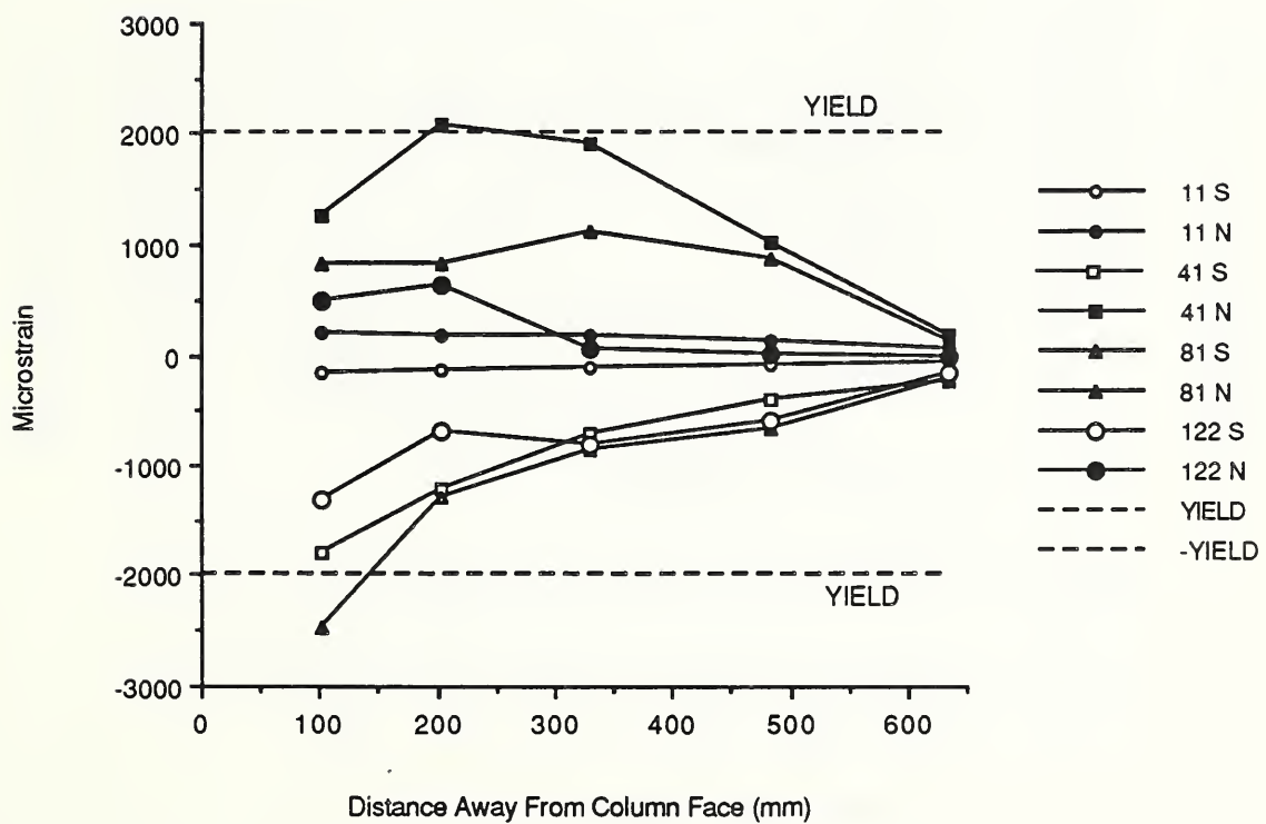
Fig. 3.26 Bottom northwest reinforcing bar strains - D-P-Z4.
