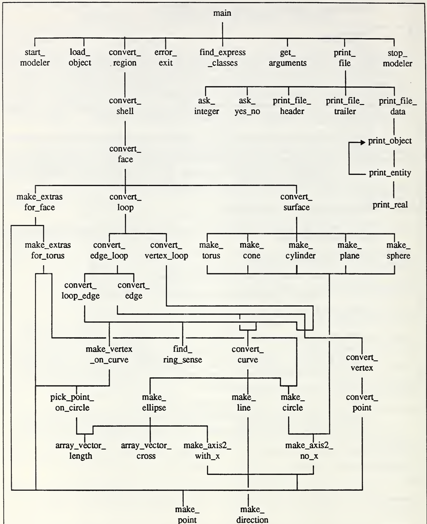
Figure 3. Hierarchy of Function Calls
