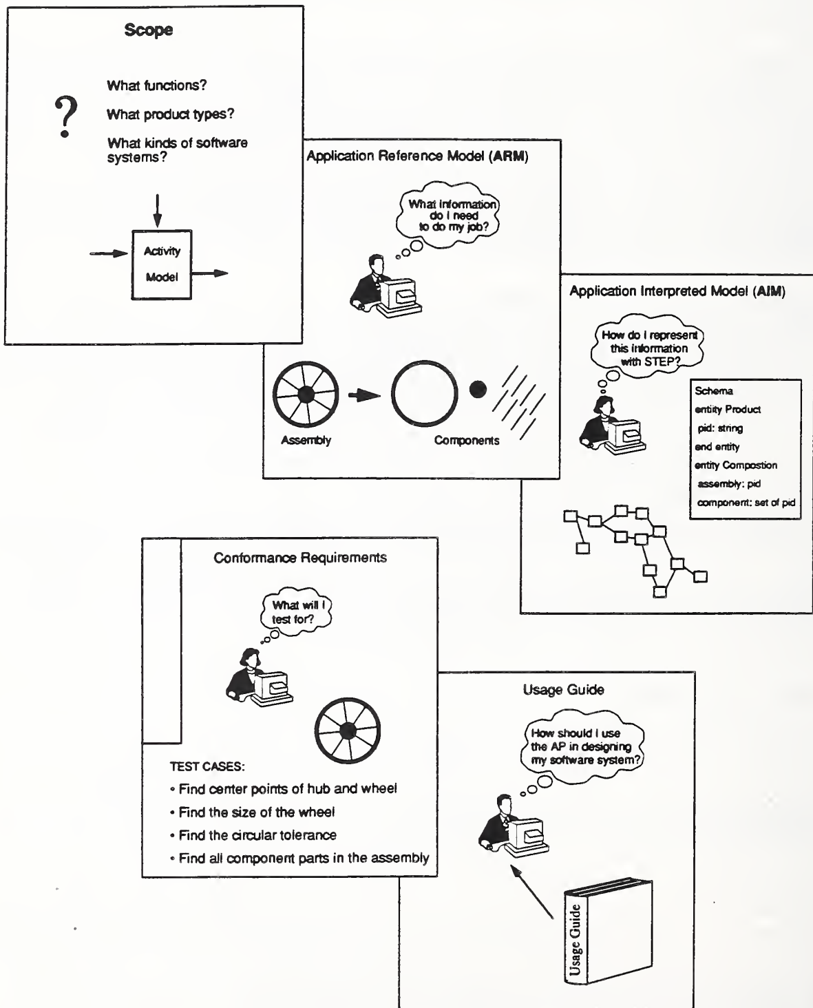
Fig. 8. The five components of an application protocol are the scope, the ARM, the AIM, the conformance requirements, and the usage guide.
