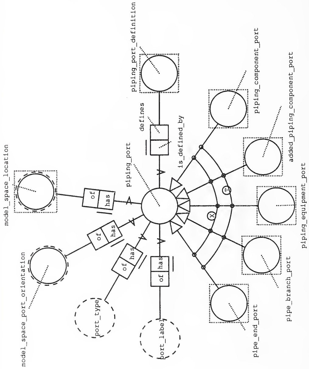
Figure 3-9. Piping port
