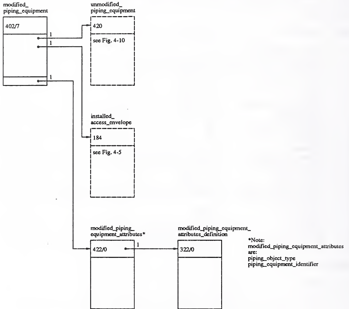
3D Piping AIM Figure 4-11. Modified piping equipment
