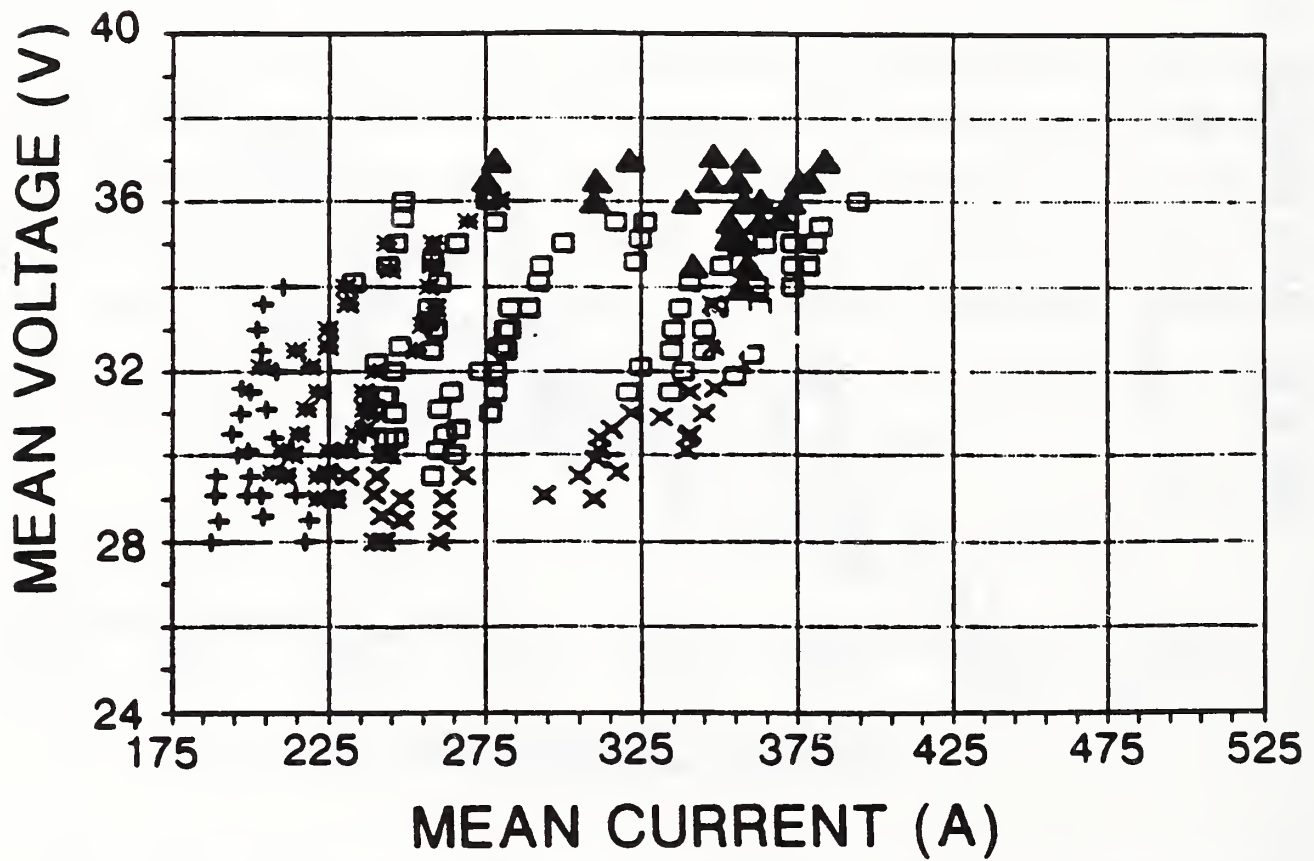
Figure 8. 25-mm contact-tube-to-work-distance: mean current versus voltage.
