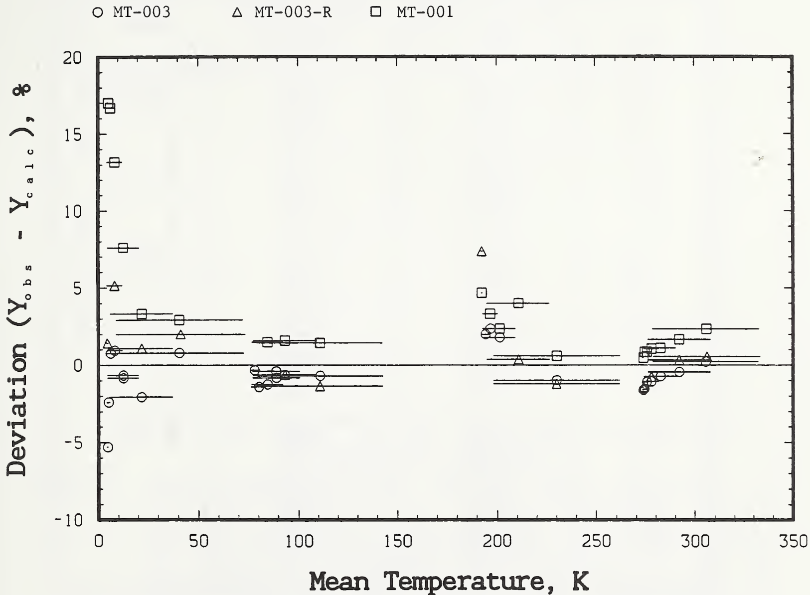
Figure 23. Comparison of relative deviation of experimental data (open squares) for PPMI film specimen MT-001 ( 25 \mu\text{m} ) with both calculated thermal conductivity (fitted curve) and experimental data (open circles and triangles) for film specimen MT-003 ( 76 \mu\text{m} ).
