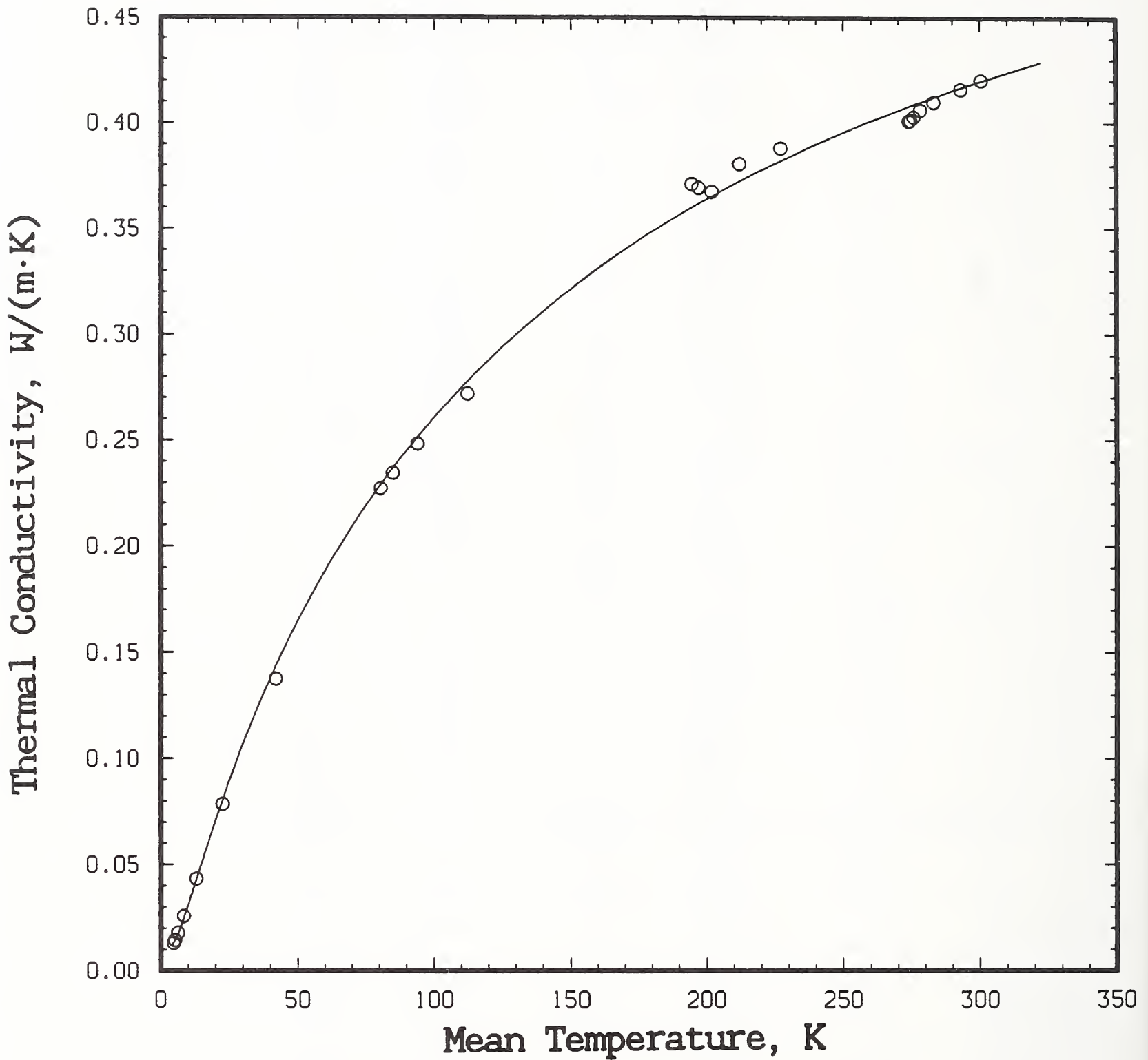
Figure 11. Thermal conductivity of PPMI film specimen MTL-003. Experimental data are presented as discrete points. Both scales are linear, which clarifies the behavior at high temperatures.
