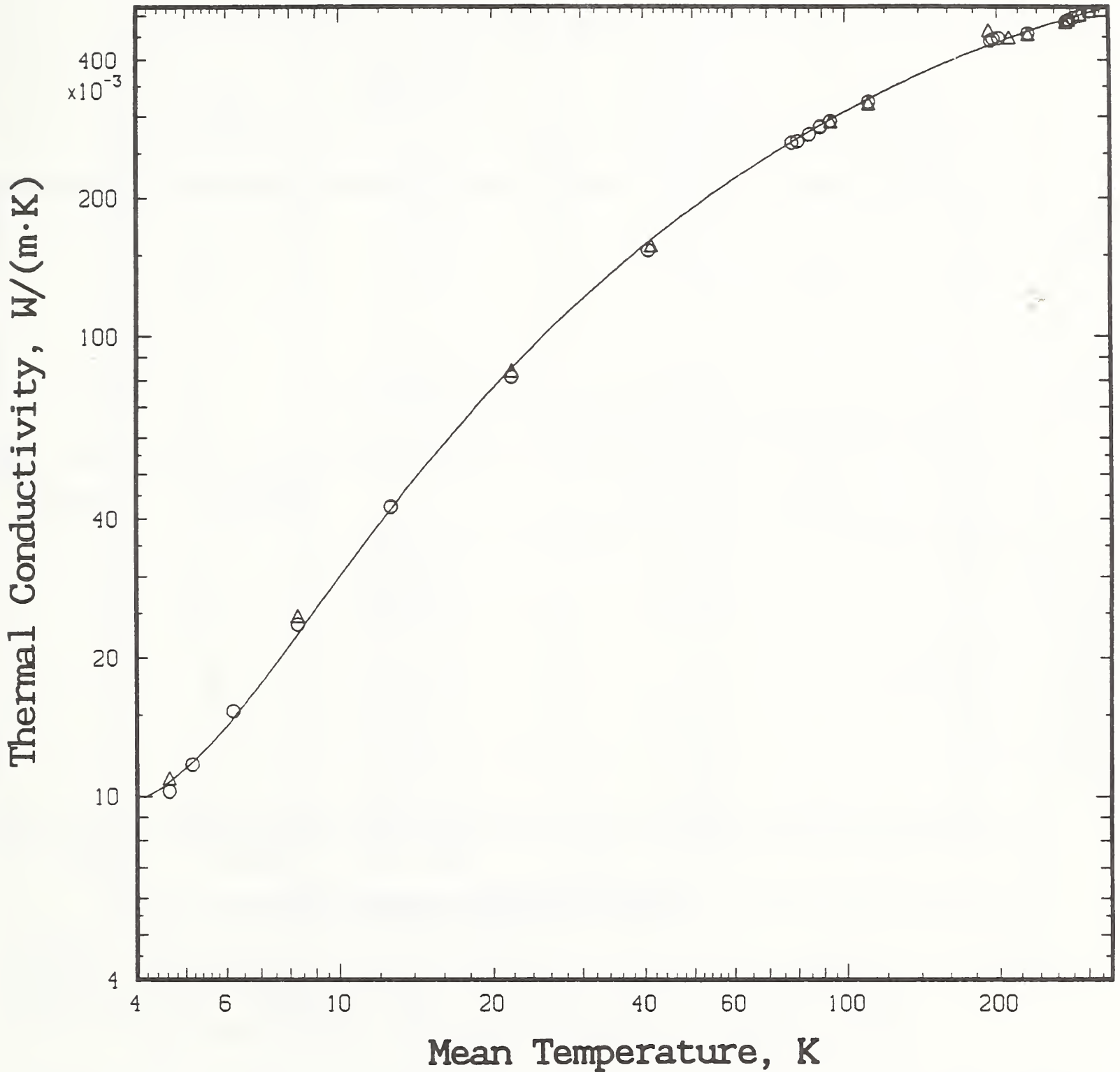
Figure 15. Thermal conductivity of PPMI film specimen MT-003 and MT-003-R (repeated measurements on same specimen). Experimental data are presented as discrete points. Two specimens were tested to determine reproducibility. Both scales are logarithmic, which clarifies the behavior at low temperatures.
