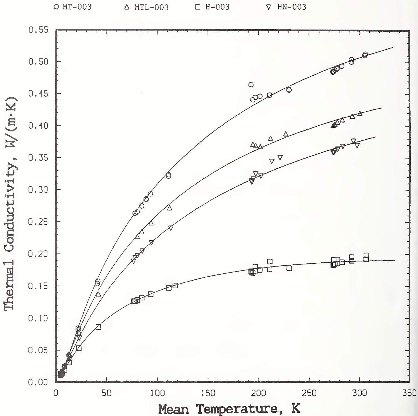
Figure 20. Thermal conductivity of four PPMI film specimens composed of layers of film 76 \mu\text{m} thick. Experimental data are presented as discrete points. [[Specimens MT-003 and H-003 were retested to determine reproducibility.]] Both scales are linear, which clarifies the behavior at high temperatures.
