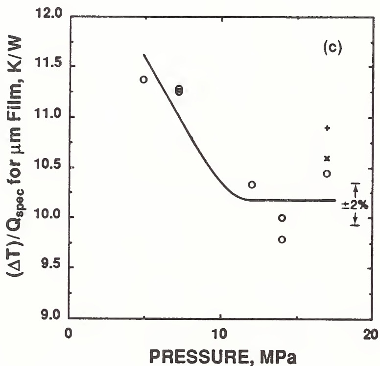
Figure 25. Thermal contact resistance, \Delta T/Q , per layer of 76\text{-}\mu\text{m} PPMI film (specimen MT-003-P), as a function of mechanical pressure, at mean specimen temperatures of (a) 277.8 K (ice), (b) 80.3 K (LN), and (c) 8.3 K (LHe). Data points "+" in each plot represent contact resistance for a different specimen (MT-003) of the same material under the same conditions, calculated from table 12. Points "X" represent contact resistance for specimen MT-003-R of the same material under the same conditions, calculated from data in table 13. Error bars for each curve provide scales with which to judge the amount of scatter in the data. At all measurement temperatures, experimental reproducibility (imprecision) is within about 2 percent. Within this imprecision, contact resistance appears to become independent of pressure, for pressures above about 12 MPa (1.7 kpsi), at all three mean temperatures.
