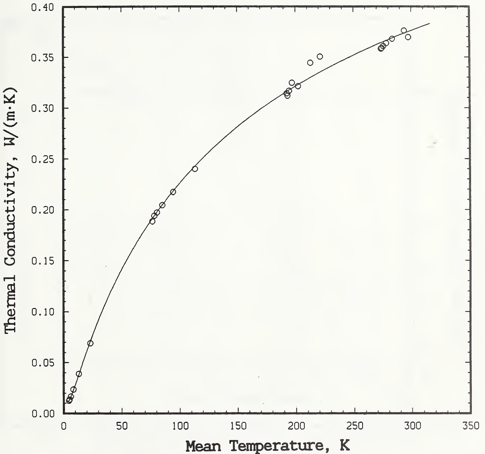
Figure 8. Thermal conductivity of PPMI film specimen HN-003. Experimental data are presented as discrete points. Both scales are linear, which clarifies the behavior at high temperatures.
