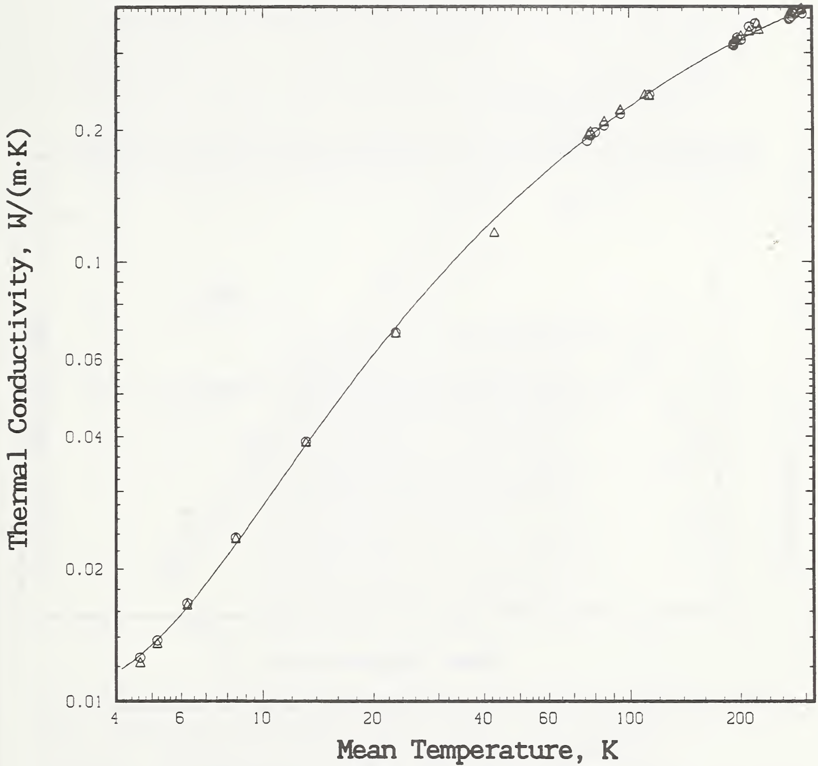
Figure 27. Intercomparison of the thermal conductivity of 76- \mu\text{m} PPMI film before (HN-003) and after (HN-Heat) a heat treatment at 150°C for ninety minutes.
