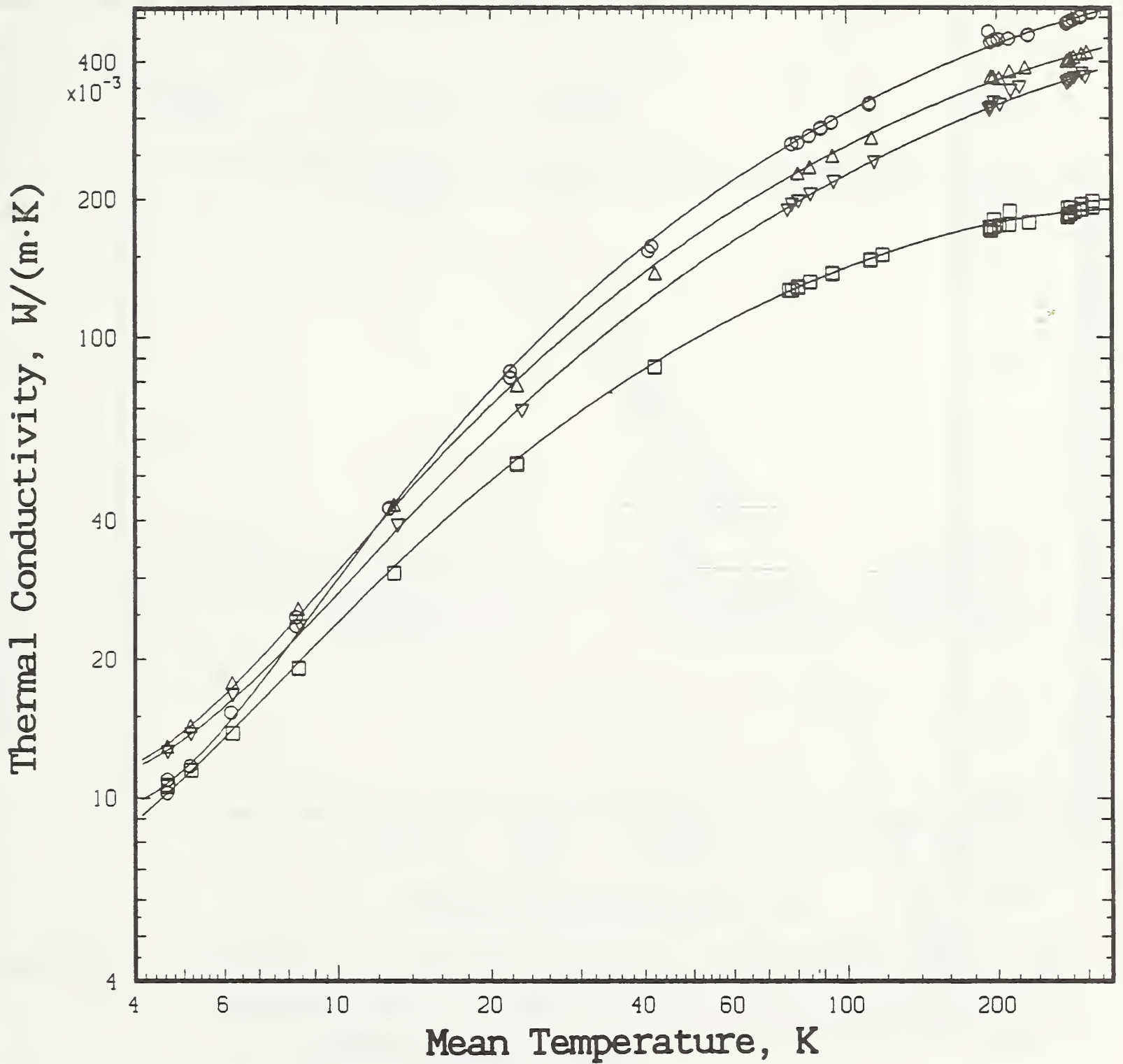
Figure 21. Thermal conductivity of four PPMI film specimens composed of layers of film 76 \mu\text{m} thick. Experimental data are presented as discrete points. Both scales are logarithmic, which clarifies the behavior at low temperatures.
