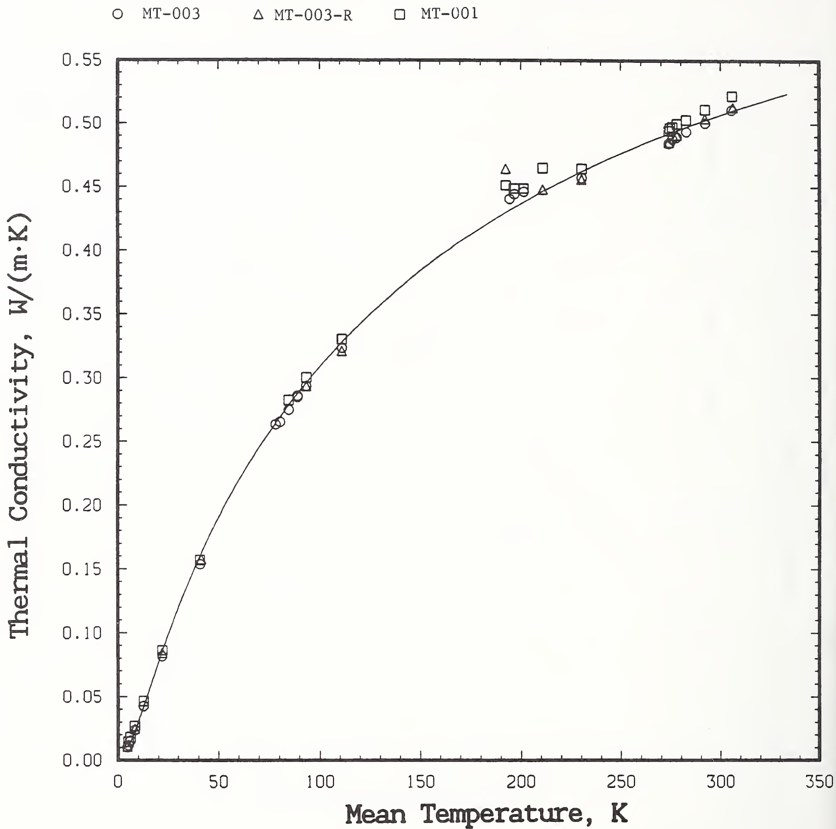
Figure 22. Intercomparison of thermal conductivity of PPMI film specimens MT-003 (thickness: 76 \mu\text{m} ) and MT-001 (thickness: 25 \mu\text{m} ).
