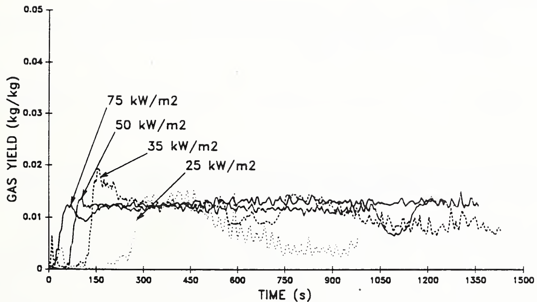
Figure 15. The Effect of Irradiance on the Production of CO from a FR Polyester/Fiber Glass Composite
