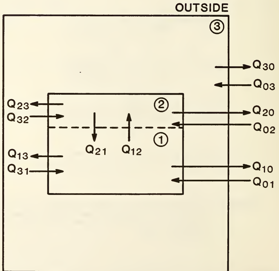
Figure 7 Schematic of a Three-Zone Model of Office Ventilation
