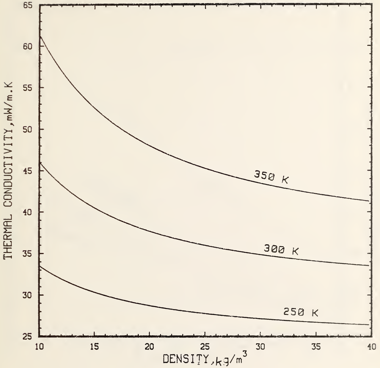
Figure 5.15 Thermal Conductivity versus Density for Several Temperatures as Calculated from the Model. Emittance = 0.95, Thickness = 2.54 cm, and Fiber Diameter = 5.0 \mu\text{m}
