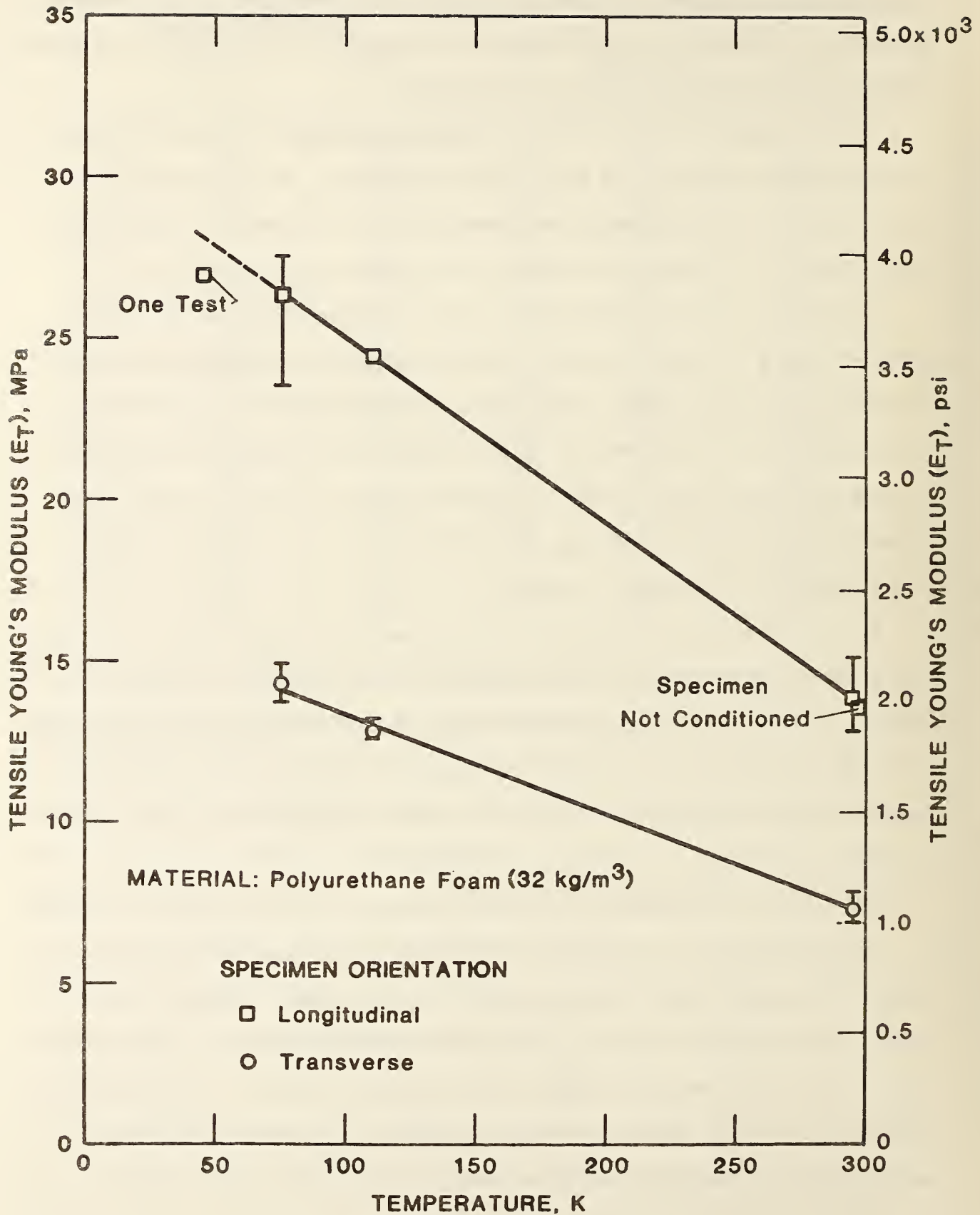
Figure 16. Tensile Young's modulus versus temperature for a 32\text{-kg/m}^3 polyurethane foam.
