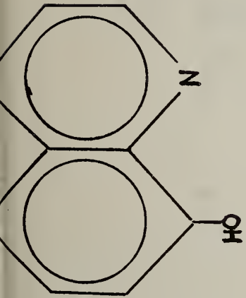
8-hydroxyquinoline (8-HQ)
