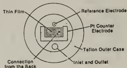
Fig. 4 The in situ EXAFS cell.
