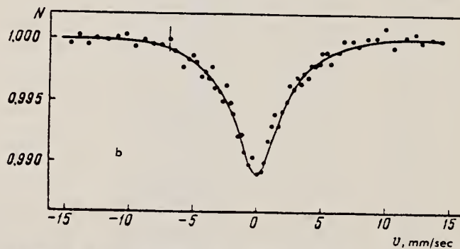
Resonance absorption spectra of \gamma quanta: a—86.5 keV, and b—60.0 keV, from Gd^{155} in gadolinium oxide, measured with a 190 mg/cm 2 absorber at 80°K. The ordinate gives the intensity of \gamma quanta in relative units; the abscissa is the velocity v of the source relative to the absorber.
