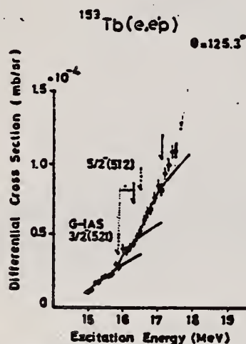
Fig. 2. Cross section of the 159 Tb(e, e'p) reactions. The solid curve and the dashed arrows are the cross sections and the IAR position obtained by the best fitting to the data with eq. (25). Solid arrows is the position of IAS estimated with eq. (20). G-IAS means the IAS of the ground state and the indicated figures are spin-parity and quantum numbers for the corresponding resonances.
