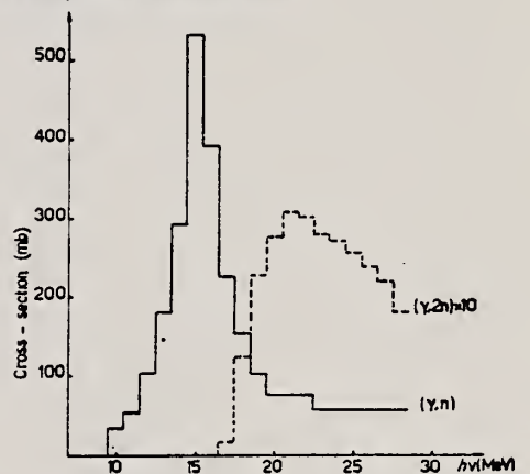
Fig. 1. The corrected ( \gamma, n ) and ( \gamma, 2n ) cross sections.
