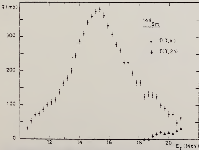
Fig. 2. Partial photoneutron cross sections [\sigma(\gamma, n) + \sigma(\gamma, np)] and \sigma(\gamma, 2n) of ^{144}\text{Sm} . ET 267
