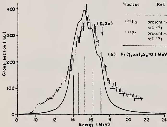
Fig. 1. (a) The ^{139}\text{La}(\gamma, xn) cross section, obtained by VBPL unfolding from yield data measured in 0.1 MeV steps. Also shown is the DCM dipole spectrum for ^{142}\text{Nd} , and a fit to it of Lorentz line shapes with widths 4.0 MeV (solid line). (b) The ^{141}\text{Pr}(\gamma, xn) cross section, obtained by VBPL unfolding from yield data measured in 0.1 MeV steps. Also shown is the DCM dipole spectrum for ^{146}\text{Nd} , and a fit to it of Lorentz line shapes with widths 1.0 MeV (solid line).
