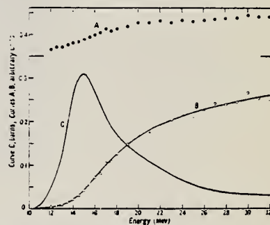
Figure 8. A, the ratio of activation curves 142 Nd(γ,n): 142 Ta(γ,n); B, activation curve for 142 Nd(γ,n); C, derived cross section: 142 Nd(γ,n).
