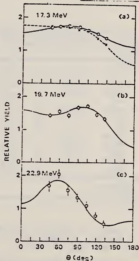
FIG. 9. Angular distributions for (a) 17.3-, (b) 19.7-, and (c) 22.9-MeV resonances. In (a) crosses and circles show the angular distribution for the \rho_0 + \rho_1 groups and those for total protons, respectively, observed in bombardment of E_p = 19.0 MeV. The solid curves show the Legendre polynomial fits.
