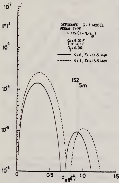
Fig. 8. The K=0 and K=1 form factors in 152 Sm calculated by assuming a deformed Fermi type charge distribution.
