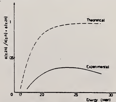
Fig. 2. Theoretical and experimental curves of the (\gamma, 2n)/(\gamma, n) + (\gamma, 2n) ratio.
