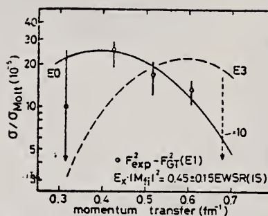
FIG. 3. The data points are identical to the difference between the cross section under the 15.3-MeV ( E1 ) resonance and a DWBA calculation based on the GT model and normalized to ( \gamma, \pi ) results (lowest curve in Fig. 2). Comparison with a monopole DWBA calculation shows that this difference is compatible with the presence of 45% of the E0 EWSR. Reasons against such an interpretation are given in the text.
