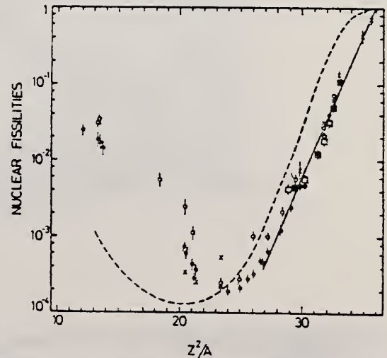
Fig. 2. Nuclear fissilities as a function of Z^2/A . Experimental points: solid circles represent our data; squares, the data from ref. 4 ); open circles, the data from ref. 7 ); and crosses, the data from (p.f) experiments 20 ). The straight line is the best fit calculated from our data for Z^2/A > 26 . The dashed curve is the curve VI calculated by Nix and Sassi 12 ).
