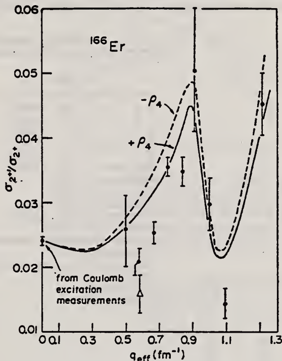
FIG. 9. Ratio of the cross sections observed for exciting the 0.786-MeV ( 2' ) \gamma -vibrational level to that for exciting the 0.081-MeV ( 2^+ ) state. The best fit curves differ only in the sign of the \rho_4 component of the charge distribution, since the sign is not determined by form factor fits to the ground state rotational band data.
