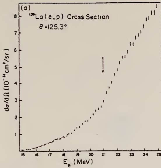
Fig. 2. The differential cross sections of the (e, p) reaction at \theta = 125.3^\circ lab. The arrows show the positions of inflection caused by T_c GDR. (a) ^{139}\text{La} . (b) ^{141}\text{Pr} .
