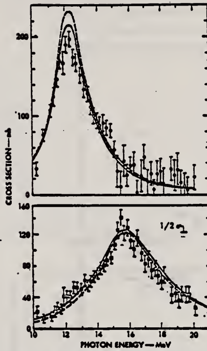
FIG. 16. The intrinsic cross sections for \text{Ho}^{163} . The cross section \sigma_{11} is associated with vibrations along the 'nuclear symmetry axis'; \sigma_{\perp} is that associated with vibrations perpendicular to this axis. The error bars represent statistical errors, and not those due to the uncertainty of f_3 . The solid curves are those derived from the elementary collective model; the dashed ones are calculated from the dynamic collective model.
