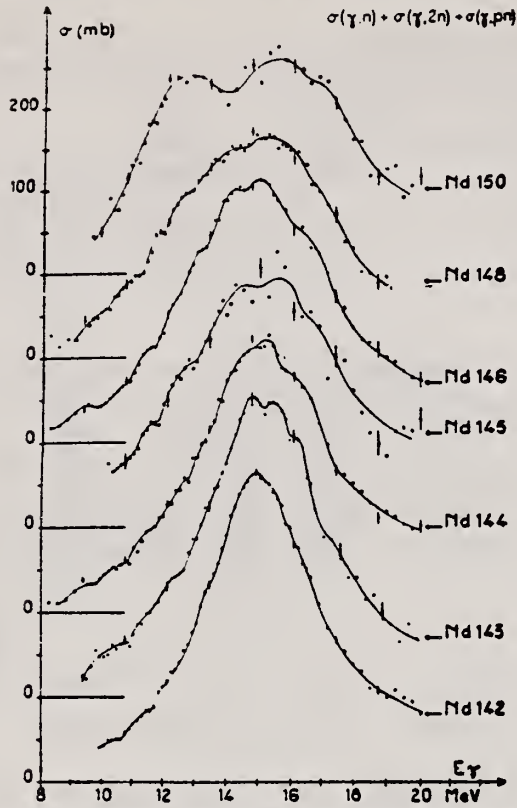
Fig. 9. Total photoneuclear cross-section \sigma_T of neodymium isotopes. The full line drawn through the experimental points is merely meant to facilitate the identification of structure.
