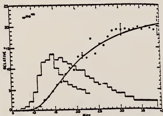
FIG. 5. Relative photon-neutron production cross sections for tin, iodine, samarium, holmium, erbium, and lead. The points and smooth curves represent the integral neutron-production cross section defined by \int_0^E \sigma_{\gamma n}(E) dE , where \sigma_{\gamma n}(E) = \sigma(\gamma, n) + 2\sigma(\gamma, 2n) + \sigma(\gamma, 3n) + 3\sigma(\gamma, 3n) + \dots . The scales are normalized to give approximately the same total neutron yield at 40 Mev. The errors indicated were obtained by propagating the statistical uncertainties, (\sqrt{n}) , in the original activation curve data through the integral cross section matrix. Solid histograms represent first differences of integral cross section curves. Dashed histograms show result of correcting for neutron multiplicity above the (\gamma, 2n) threshold.
