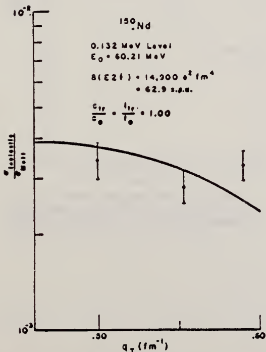
Fig. 17. Inelastic form factors for the 132 keV, 2^+ level in ^{150}\text{Nd} as a function of inelastic momentum transfer. The experimental points are the results of this experiment while the solid line traces out the best fit provided by parameters shown.
