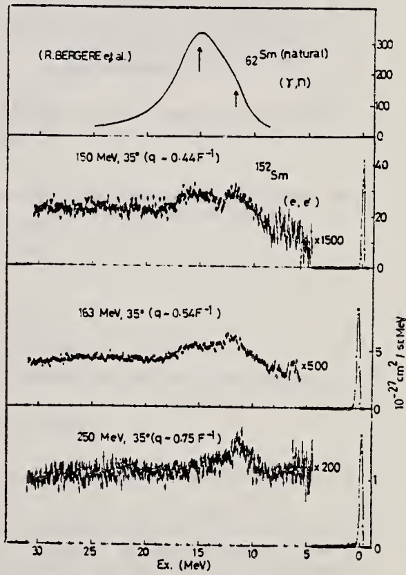
Fig. 7. The spectra of the deformed 152 Sm displayed as a function of the momentum transfer. The distinct peaks are seen at 11.5 and 15.5 MeV.
