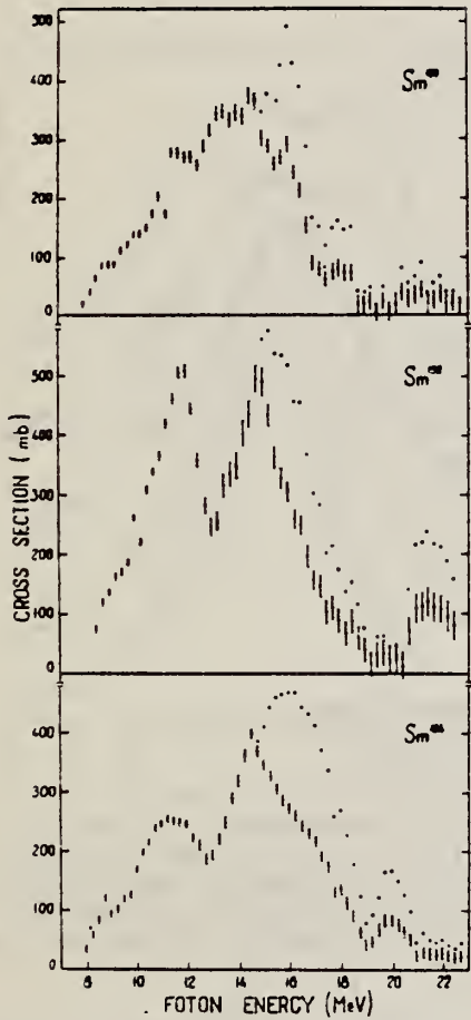
Fig. 3. The photoneutron and photoabsorption cross sections of ^{150}\text{Sm} , ^{152}\text{Sm} and ^{154}\text{Sm} . The symbols are the same as in fig. 2.
