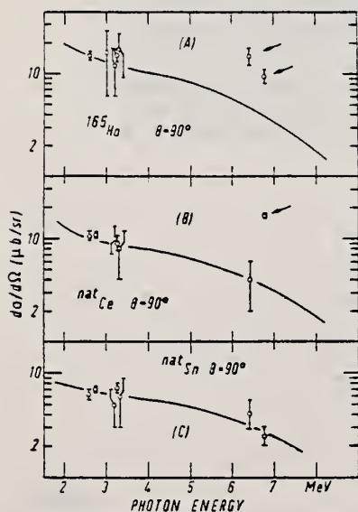
Fig. 11. Same as Fig. 9 but for (A) ^{165}\text{Ho} , (B) ^{nat}\text{Ce} and (C) ^{nat}\text{Sn}
