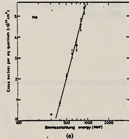
Fig. 1. Cross sections per equivalent quantum \sigma_q(E) as a function of \log E .
