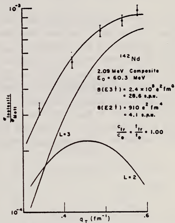
Fig. 15. Inelastic form factors for the excitation at approximately 2.09 MeV in 142 Nd. The experimental points are the findings of this experiment while the solid line through them represents the best fit obtained by an addition of the L = 2 and L = 3 curves shown. (L is the transition multipolarity.) The individual B(EL↑) values are given in the figure. See text.
