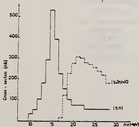
Fig. 1. The corrected ( \gamma, n ) and ( \gamma, 2n ) cross sections. Fig. 2. Theoretical and experimental curves of the ( \gamma, 2n )/( \gamma, n ) + ( \gamma, 2n ) ratio.
