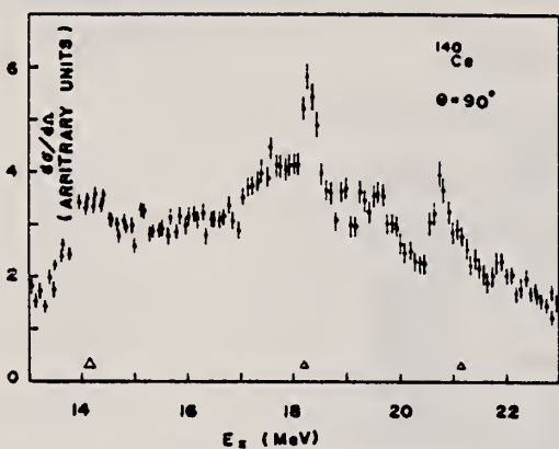
Fig. 2. Photoproton cross section for ^{140}\text{Ce} calculated from the energy distribution of the E_0 = 30.0 MeV bombardment.
