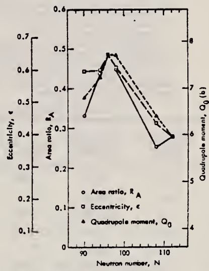
FIG. 9. The area ratio R_A , nuclear eccentricity \epsilon , and intrinsic quadrupole moment Q_0 plotted versus neutron number N . The data were scaled between the value for \text{Gd}^{150} and that for \text{W}^{182} . The absolute scale for Q_0 is based on a mean radius parameter R_0 = 1.26 F . The lines merely connect the three sets of data points. The experimental uncertainties have been omitted for clarity but are given in Tables VII and VIII; their average values are 0.065 (17%) for R_A , 0.010 (1.9%) for \epsilon , and 0.26b (3.7%) for Q_0 .
