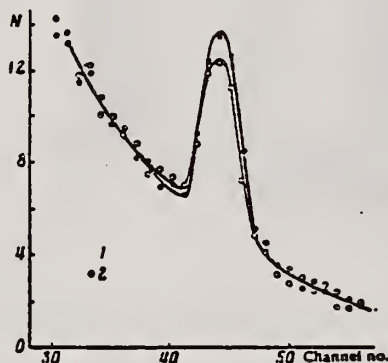
Fig. 3. The spectrum of the scattered radiation in the case ^{159}\text{Gd} ^{159}\text{Tb} at a source temperature of 1000^\circ \text{C} . 1) Terbium scatter; 2) samarium scatter. N = hundreds of pulses in 20 min. In nonresonance conditions ( T = 20^\circ \text{C} ) the scattering from both scatterers was the same N_{\text{Tb}}/N_{\text{Sm}} = 1.012 \pm 0.003 .
