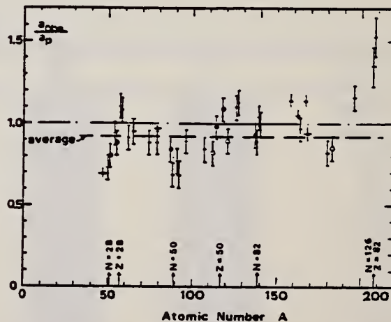
Fig. 15. Ratio a_{nnn}/a_p versus atomic number A . Here a_{nnn} is the level density parameter taken from the neutron resonance work of refs. 1,2), and a_p is the level density parameter derived from the present (\gamma, n) work. Filled circles represent points where nuclei in the neutron resonance and in the (\gamma, n) experiment were the same. Open circles represent points where the respective nuclei were approximately matched. Triangles represent points which are based on measurement of neutron mean energies at two bremsstrahlung energies only.
