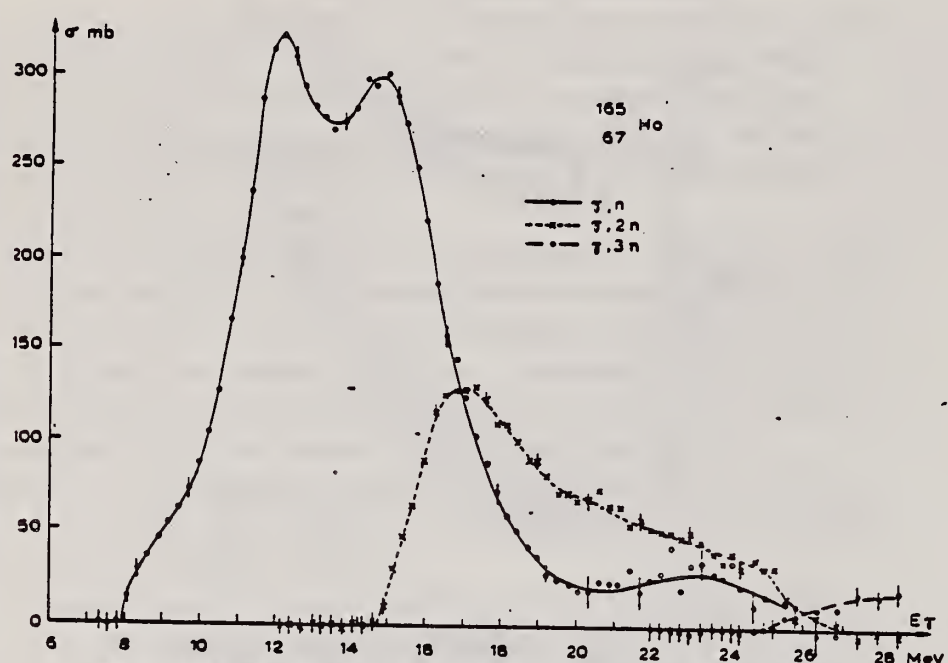
Fig. 4. Partial photoneuclear cross sections \sigma(\gamma, n) , \sigma(\gamma, 2n) and \sigma(\gamma, 3n) of ^{165}\text{Ho} .
