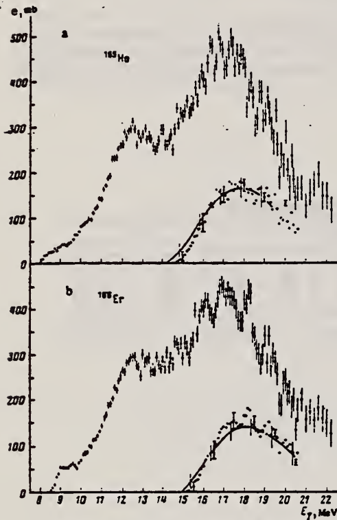
FIG. 1. Photon neutron production cross section \sigma_n , obtained for ^{165}\text{Ho} (a) and for ^{166}\text{Er} (b). The hollow and solid circles correspond to two independent series of data. The solid curves show the (\gamma, 2n) cross sections calculated from the data of a statistical experiment by the regularization method. [12] The circles near the curves give the same cross sections calculated from the formula \sigma_n(1-f(E, a)) .
