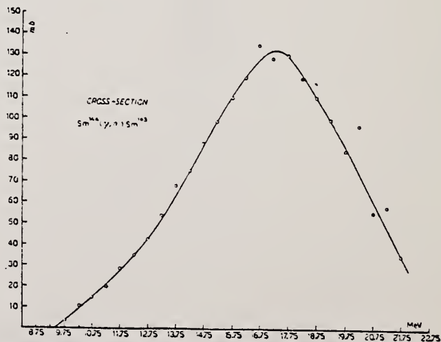
Fig. 3. - Cross section for the reaction 144 Sm(γ, n) 143 Sm.
