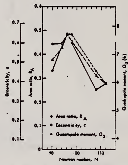
FIG. 9. The area ratio R_A , nuclear eccentricity e , and intrinsic quadrupole moment Q_0 plotted versus neutron number N . The data were scaled between the value for Gd^{160} and that for W^{182} . The absolute scale for Q_0 is based on a mean radius parameter R_0 = 1.26 F . The lines merely connect the three sets of data points. The experimental uncertainties have been omitted for clarity but are given in Tables VII and VIII; their average values are 0.065 (17%) for R_A , 0.010 (1.9%) for e , and 0.26b (3.7%) for Q_0 .
