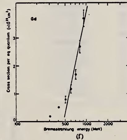
Fig. 1. Cross sections per equivalent quantum \sigma_q(E) as a function of \log E .
