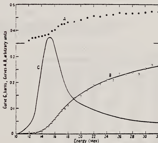
Figure 9. A, the ratio of activation curves 144 Sm( \gamma, n )/ 181 Ta( \gamma, n ); B, activation curve for 144 Sm( \gamma, n ); C, derived cross section: 144 Sm( \gamma, n ).
