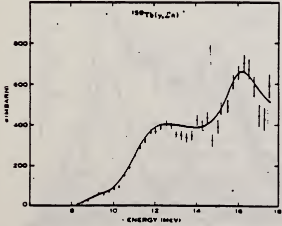
Fig. 6.—Total neutron production cross section for 159 Tb.
