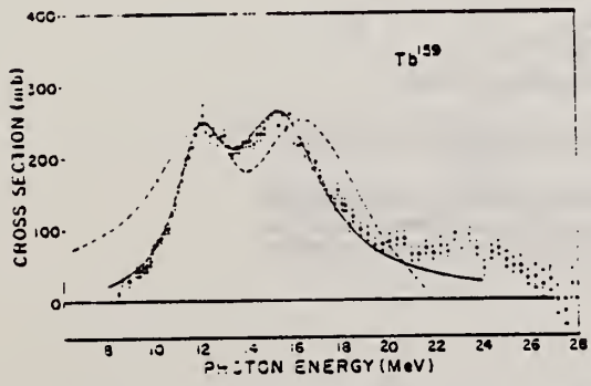
Fig. 5. The photon absorption cross section of Tb^{159} obtained by adding the (\gamma, n) and (\gamma, 2n) cross sections of Fig. 4. The electric dipole giant resonance is double peaked due to the quadrupole moment of Tb^{159} . The solid curve is the sum of two Lorentz curves with parameters given in Table III. The dashed curve is from Wilkinson (Ref. 9).
