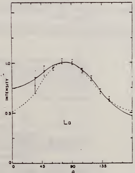
Fig. 10. Angular distribution of fast neutrons from lanthanum. See fig 3
