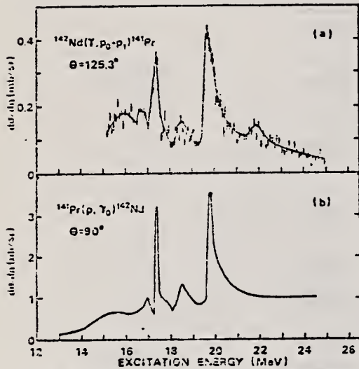
FIG. 2. (a) Differential cross section for the ^{142}\text{Nd}(\gamma, p_1 + p_0)^{141}\text{Pr} reaction at \theta_p = 125.3^\circ . The line drawn is merely to guide the eye. (b) Differential cross section for the ^{141}\text{Pr}(p, \gamma)^{142}\text{Nd} reaction at \theta_p = 90^\circ from Ref. 7.
