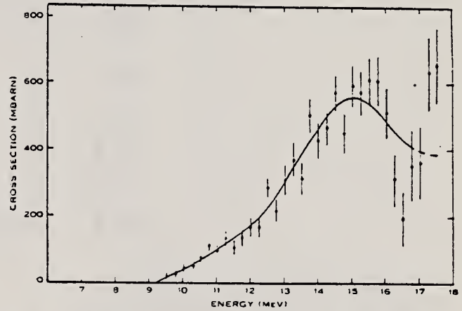
Fig. 5.—Total neutron production cross section for 141 Pr. The points are obtained by analysis using the experimental points. The smooth curve is obtained by analysis of a smooth yield curve drawn through the experimental points.
