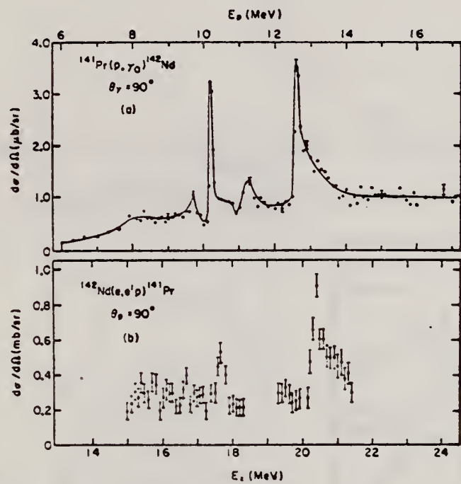
Fig. 3. (a) Differential yield curve of ^{141}\text{Pr}(p, \gamma)^{142}\text{Nd} at \theta_\gamma = 90^\circ . The line drawn is merely to guide the eye. (b) The ^{142}\text{Nd}(e, e'p)^{141}\text{Pr} data of ref. 15).
