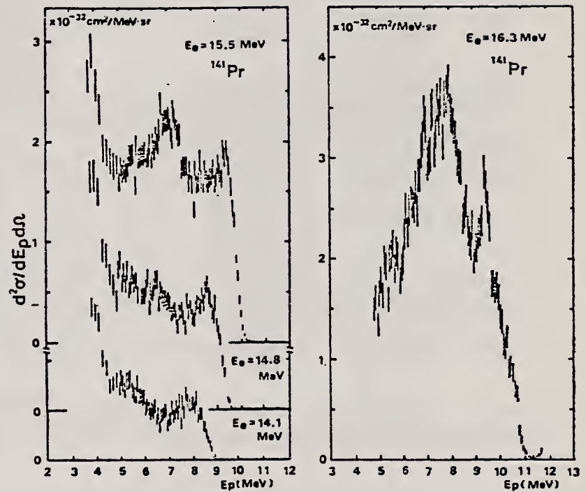
Fig. 4. The proton spectra of the ^{141}\text{Pr}(e, e'p) reactions for \theta = 125.3^\circ .
