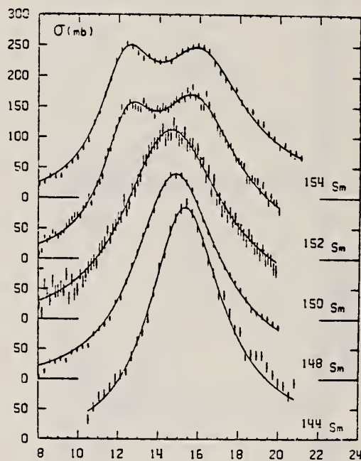
Fig. 19 Total photoneutron cross section \sigma(\gamma,n) + \sigma(\gamma,2n) of Sm isotopes. The solid lines show the best 1 Lorentz line fit ( ^{144}\text{Sm} ^{148}\text{Sm} ^{150}\text{Sm} ) or 2 Lorentz lines fit ( ^{152}\text{Sm} and ^{154}\text{Sm} ).
