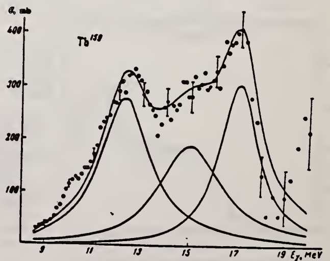
FIG. 11. Approximation of σ γ of Tb 159 by three Lorentz lines.
