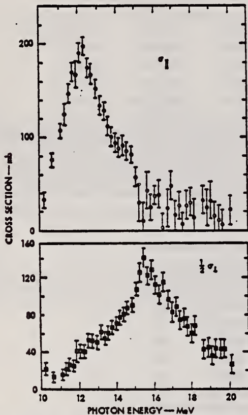
FIG. 14. The intrinsic cross sections for Ho 165 . The cross section \sigma_{\parallel} is associated with vibrations along the nuclear symmetry axis. One-half \sigma_{\perp} is half the cross section associated with vibrations perpendicular to the symmetry axis. The error bars represent statistical errors, and not those due to the uncertainty of f_2 .
