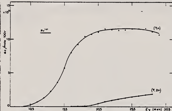
Fig. 1. Excitation functions for Pr^{141}(\gamma, n)Pr^{140} and Pr^{141}(\gamma, 2n)Pr^{139} reactions.
