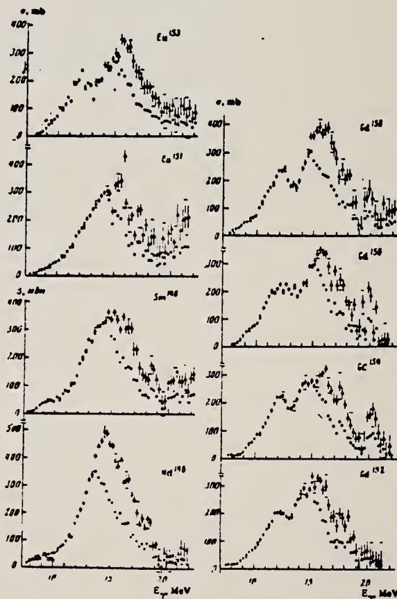
FIG. 1. Photonuclear cross sections and photoabsorption cross sections of Nd 146 , Sm 148 , Eu 151 , Eu 153 , Gd 154 , Gd 156 and Gd 158 . Statistical and rms experimental errors are shown (the latter horizontal bars at 9.42 MeV, 10.42 MeV etc.) At photon energies above the ( \gamma , 2n) threshold the photoabsorption cross section errors are not shown.
