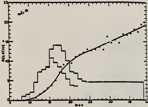
FIG. 5. Relative photon-neutron production cross sections for tin, iodine, samarium, holmium, erbium, and lead. The points and smooth curves represent the integral neutron-production cross section defined by \int_0^E \sigma_{T_n}(E) dE , where \sigma_{T_n}(E) = \sigma(\gamma, n) + 2\sigma(\gamma, 2n) + \sigma(\gamma, 3n) + 3\sigma(\gamma, 3n) + \dots . The scales are normalized to give approximately the same total neutron yield at 40 Mev. The errors indicated were obtained by propagating the statistical uncertainties, (\sqrt{n}) , in the original activation curve data through the integral cross section matrix. Solid histograms represent first differences of integral cross section curves. Dashed histograms show result of correcting for neutron multiplicity above the (\gamma, 2n) threshold.
