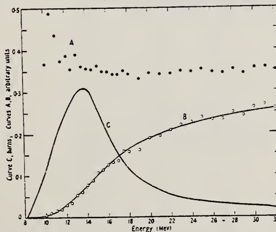
Figure 5. A, the ratio of activation curves ^{154}Sm(\gamma, n)/^{181}Ta(\gamma, n) ; B, activation curve for ^{154}Sm(\gamma, n) ; C, derived cross section: ^{154}Sm(\gamma, n) .
