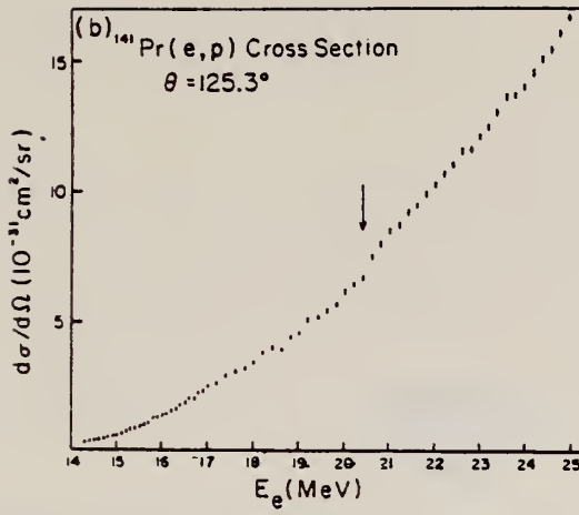
Fig. 2. The differential cross sections of the (e, p) reaction at \theta = 125.3^\circ lab. The arrows show the positions of inflection caused by T_c GDR. (a) ^{139}\text{La} . (b) ^{141}\text{Pr} .
