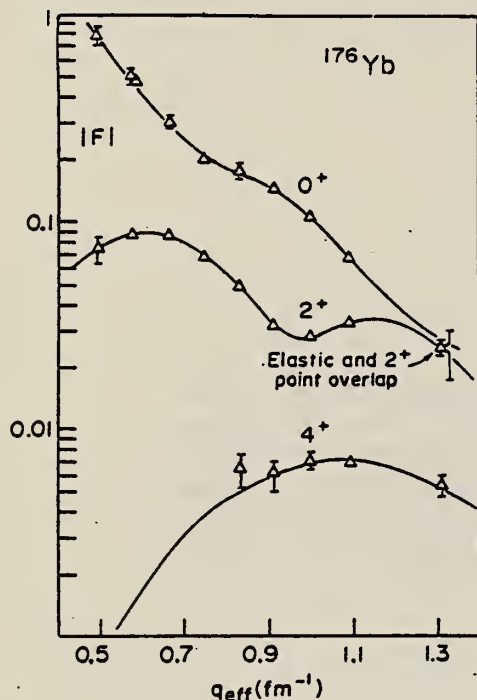
FIG. 6. Measured form factors for the elastic ( 0^+ ) and the inelastic 0.081-MeV ( 2^+ ) and 0.267-MeV ( 4^+ ) states in ^{176}\text{Yb} . The fitted curves are based on a best fit deformed Fermi charge distribution.
