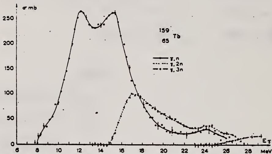
Fig. 7. Partial photoneuclear cross sections \sigma(\gamma, n) , \sigma(\gamma, 2n) and \sigma(\gamma, 3n) of ^{159}_{65}\text{Tb} .
