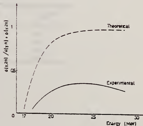
Fig. 1. The corrected ( \gamma, n ) and ( \gamma, 2n ) cross sections. Fig. 2. Theoretical and experimental curves of the ( \gamma, 2n )/( \gamma, n ) + ( \gamma, 2n ) ratio.
