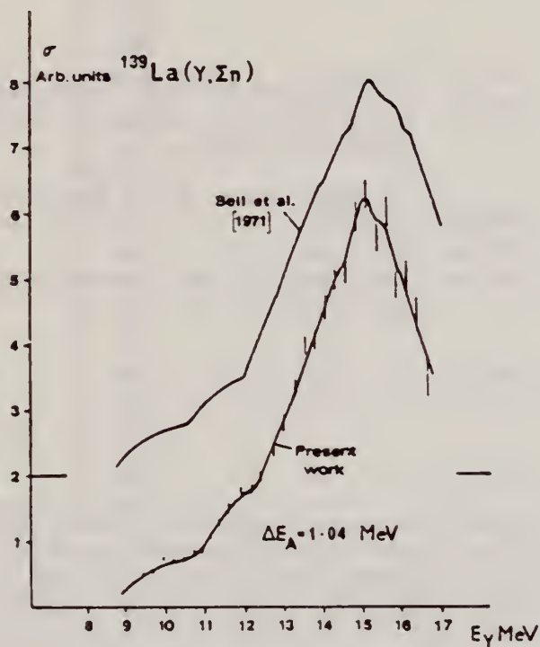
Fig. 7. Cross section for ^{139}\text{La}(\gamma, \Sigma n) .
