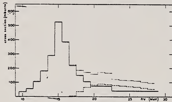
Fig. 2. Cross sections versus energy: — Pr^{141}(\gamma, n)Pr^{140} ; - - - Pr^{141}(\gamma, 2n)Pr^{139} ; ... sum of the two above processes.
