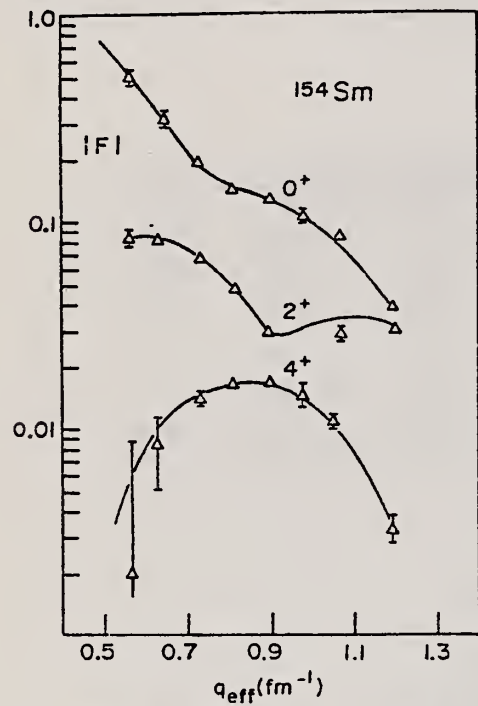
FIG. 1. Measured form factors for the elastic (0 + ) and the inelastic 0.082-MeV (2 + ) and 0.267-MeV (4 + ) states in 154 Sm. The fitted curves are based on a best fit deformed Fermi charge distribution.
