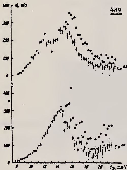
Fig. 2. Photoneutron cross sections and photoabsorption cross sections for \text{Eu}^{151} and \text{Eu}^{153} . The graphic symbols are the same as in Fig. 1.
