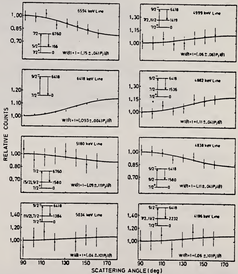
FIG. 5. Angular distributions of some intense \gamma lines scattered by 139 La using a \gamma source obtained from the Ti( n, \gamma ) reaction. See caption to Fig. 4.
