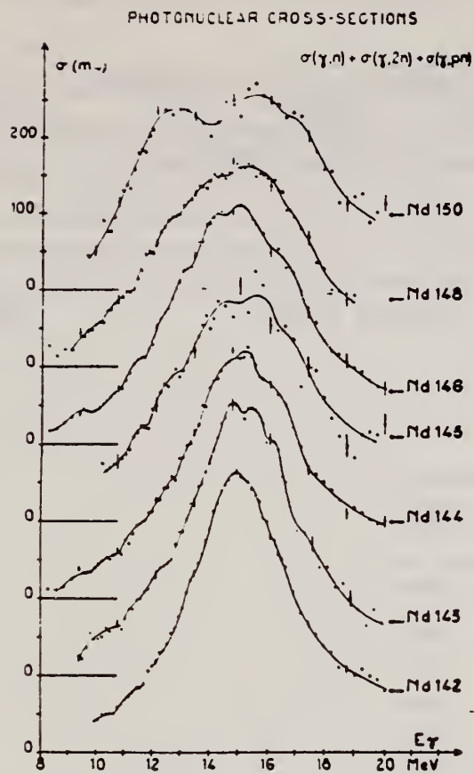
Fig. 9. Total photoneuclear cross-section \sigma_T of neodymium isotopes. The full line drawn through the experimental points is merely meant to facilitate the identification of structure.
