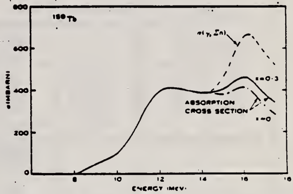
Fig. 8.—Cross section for photon absorption in 159 Tb, using statistical theory of nuclear reactions to correct for neutron multiplicity. The factor z is a measure of the probability that a direct photoeffect will occur.
