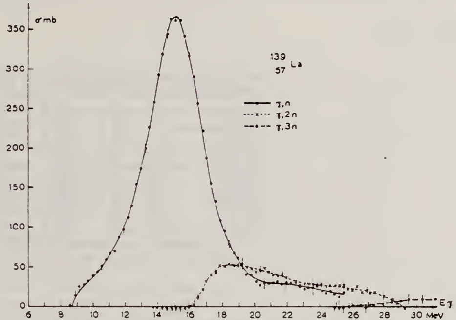
Fig. 9. Partial photoneuclear cross sections \sigma(\gamma, n) , \sigma(\gamma, 2n) and \sigma(\gamma, 3n) of ^{139}_{57}\text{La} .
