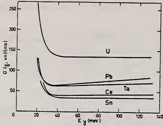
Fig. 11. The general behaviour of the "smoothed" average neutron yield cross sections \sigma(\gamma, xn) = \sum_i \sigma(\gamma, in; E_\gamma) for the Sn, Ce, Ta, Pb and U nuclei studied in the present paper (see text).
