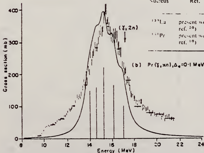
Fig. 1. (a) The ^{139}\text{La}(\gamma, xn) cross section, obtained by MBPL unfolding from yield data measured in 0.1 MeV steps. Also shown is the DCM dipole spectrum for ^{142}\text{Nd} , and a fit to it of Lorentz line shapes with widths 4.0 MeV (solid line). (b) The ^{141}\text{Pr}(\gamma, xn) cross section, obtained by MBPL unfolding from yield data measured in 0.1 MeV steps. Also shown is the DCM dipole spectrum for ^{146}\text{Nd} , and a fit to it of Lorentz line shapes with widths 1.0 MeV (solid line).
