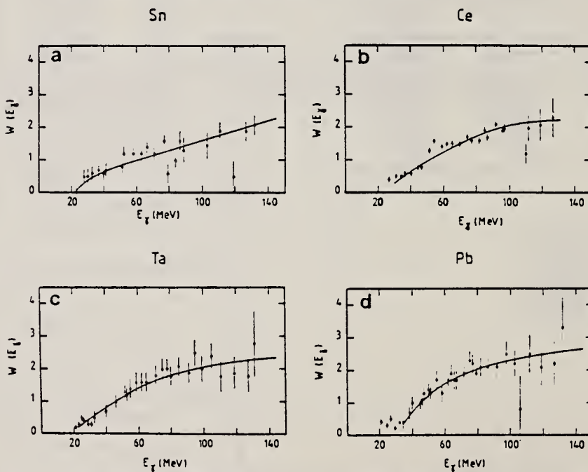
Fig. 3. Widths, W(E_\gamma) of the experimental photoneutron multiplicity distributions as a function of the photon energy E_\gamma for 25 \text{ MeV} \leq E_\gamma \leq 140 \text{ MeV} . Data points were evaluated using results from ref. 1) . The full line represents a smoothed average behaviour. Fig. 3a: Sn; fig. 3b: Ce; fig. 3c: Ta; fig. 3d: Pb.
