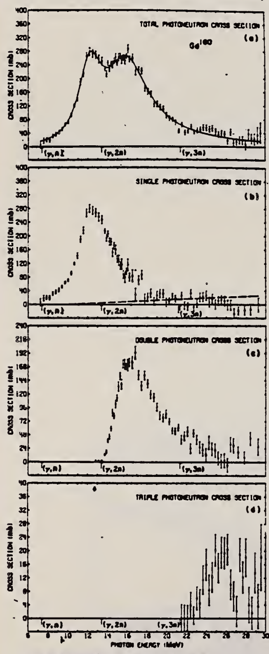
FIG. 6. Photonuclear cross sections for Gd 160 : (a) \sigma[(\gamma, n) + (\gamma, pn) + (\gamma, 2n) + (\gamma, p2n) + (\gamma, 3n)] , (b) \sigma[(\gamma, n) + (\gamma, pn)] , (c) \sigma[(\gamma, 2n) + (\gamma, p2n)] (d) \sigma(\gamma, 3n) .
