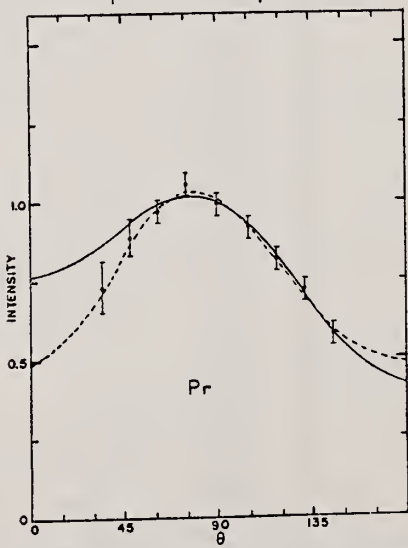
Fig. 9. Angular distribution of fast neutrons from praseodymium. See fig. 5.
