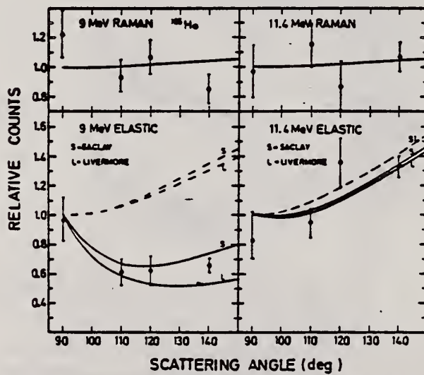
Fig. 8. Angular distributions of elastic and inelastic Raman scattered lines from ^{165}\text{Ho} . Here, S and L indicate calculated values where the nuclear resonance amplitudes were extracted from the (\gamma, n) data of Saclay and Livermore. See caption to fig. 7.
