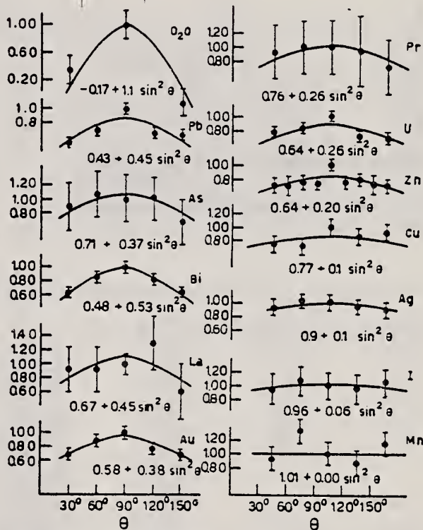
Fig. 4. Angular distributions of fast photonucleons as observed with the Si 28 (n, p)Al 28 detector. Data normalized at 90° in each case.
