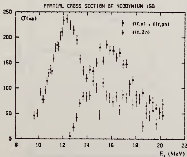
Fig. 8. Partial photonuclear cross sections \sigma(\gamma, n) and \sigma(\gamma, 2n) of 150 Nd.
