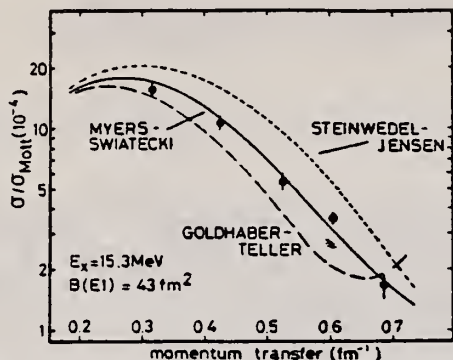
FIG. 2. Comparison between the experimental cross section divided by the Mott cross section [called form factor (squared) in the text] and DWBA calculations [S. T. Tuan et al. , Nucl. Instrum. Methods 60 , 70 (1968)] as a function of momentum transfer. Since the data were taken at four different energies (150 MeV, 93°; 65 MeV, 93°; 80 MeV, 90°; 92 MeV, 90° and 105°), form factors were constructed from separate calculations at the correct momentum transfer for each energy and connected by a smooth curve. Other methods presenting ( e, e' ) data in this case are possible, but ours has the advantage of not manipulating the experimental points.
