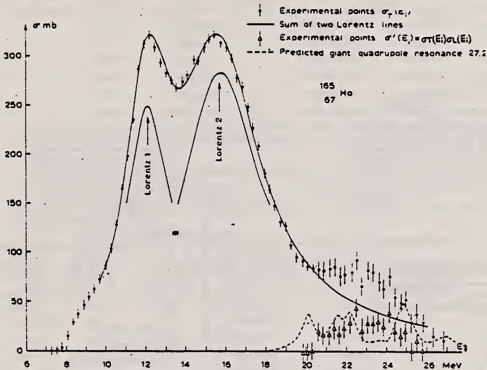
Fig. 5. Total cross section data showing a two Lorentz line fit for a ^{165}\text{Ho} target.
