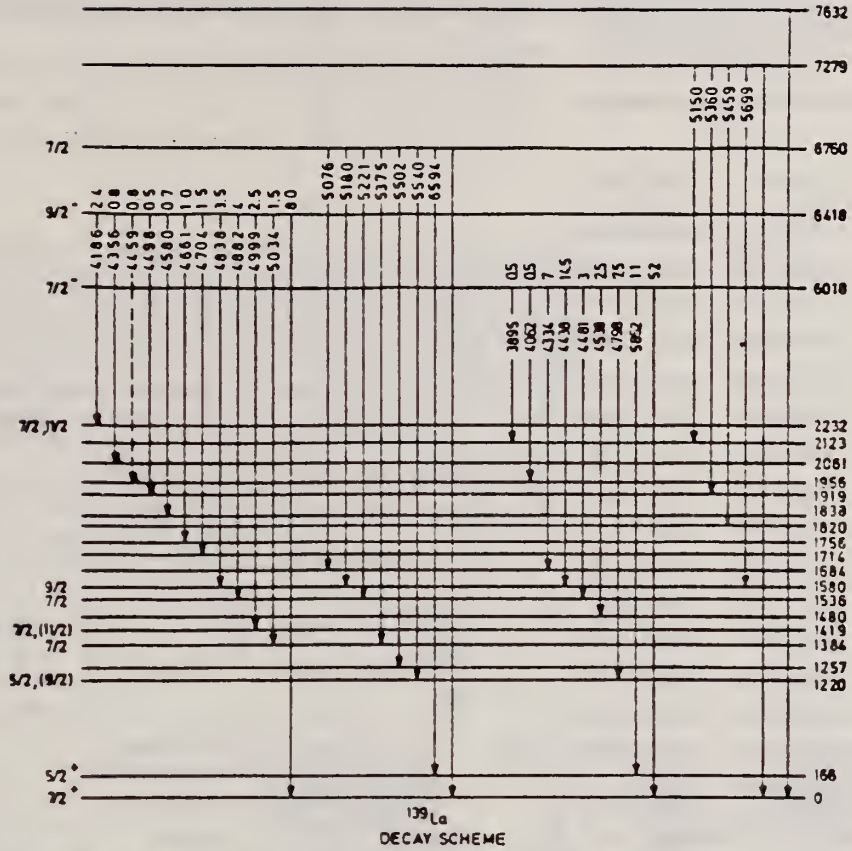
FIG. 3. Decay scheme of five resonance levels of 139 La showing branching ratios for only two strongly excited resonances where most of the inelastically scattered lines are believed to have been detected. Spin and parities for some levels assigned in the present work, are given. Parentheses and broken lines indicate uncertainties.
