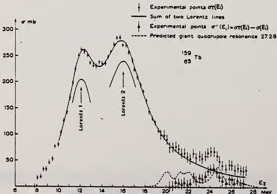
Fig. 8. Total cross section data showing a two Lorentz line fit for a ^{159}_{65}\text{Tb} target. 414
