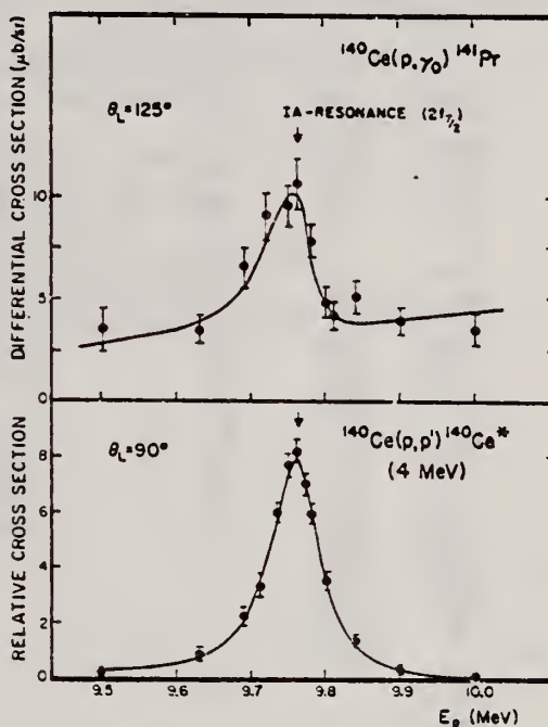
Fig. 4. Excitation function of the ^{140}\text{Ce}(p, \gamma)^{141}\text{Pr} reaction through the 2f_{7/2} IA resonance for the two-quanta escape peak of the ground state transition (upper part) and that of the ^{140}\text{Ce}(p, p')^{140}\text{Ce}^* reaction leaving the 4^- particle-hole state at 4 MeV (lower part). Solid lines are calculated ones. For the fit to the (p, p') excitation function, a slight interference effect \sqrt{T_p} \cdot (E - \bar{E}) is also used.
