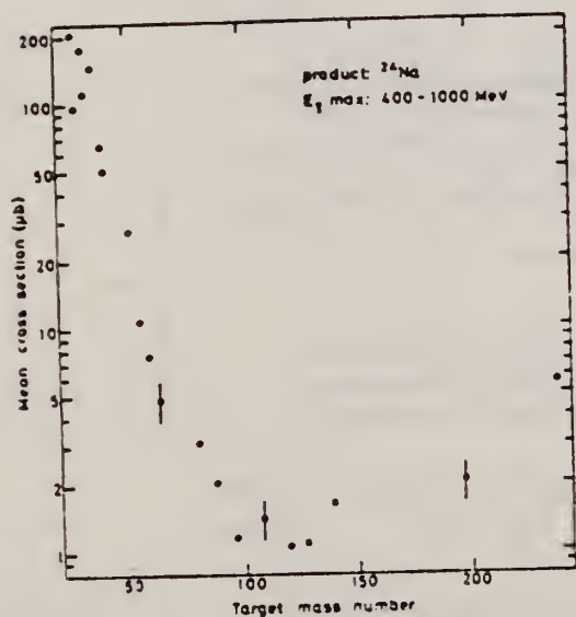
Fig. 2. The mean cross section in the energy range 400 to 1000 MeV calculated from the yields of Figure 1 in this work and of Figures 1 to 3. The error bars given by bars in some points.
