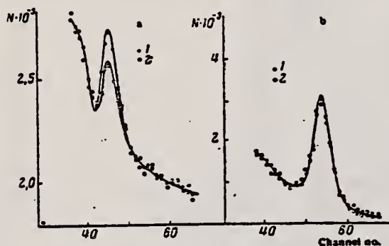
Fig. 2. Scattered radiation spectra: b) with ^{155}\text{Eu} source ( E_\gamma = 105 keV). 1) Ho scatterer; 2) (Ta + Cd) scatterer. N is the number of pulses in an interval of 10 min. a) ^{165}\text{Dy} source. 1) Ho scatterer; 2) (Ta + Cd) scatterer. N is the number of pulses in an interval of 20 min.
