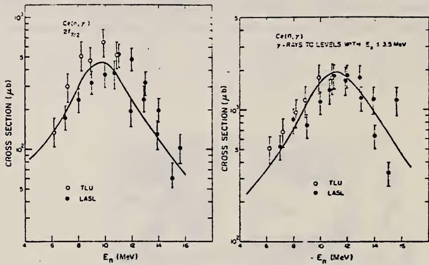
Fig. 4. Experimental (n, \gamma) cross sections for \gamma -ray transitions to the 2f_{7/2} states in ^{141}\text{Ce} ( E_B = 5.44 MeV) and ^{143}\text{Ce} ( E_B = 5.15 MeV), and the integrated cross section for \gamma -ray transitions to levels in the regions corresponding to excitation energies below 3.5 MeV in ^{141}\text{Ce} . (For further notation, see caption to fig. 3.)
