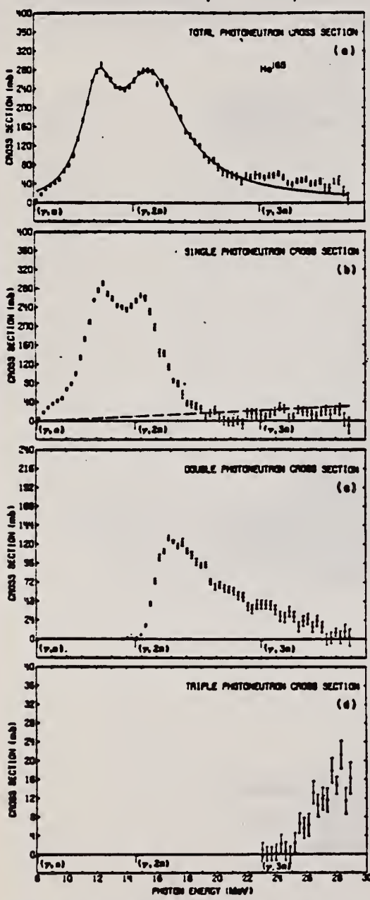
FIG. 7. Photoneutron cross sections for Ho^{165} : (a) \sigma[(\gamma, n) + (\gamma, pn) + (\gamma, 2n) + (\gamma, p2n) + (\gamma, 3n)] , (b) \sigma[(\gamma, n) + (\gamma, pn)] , (c) \sigma[(\gamma, 2n) + (\gamma, p2n)] , (d) \sigma(\gamma, 3n) .
