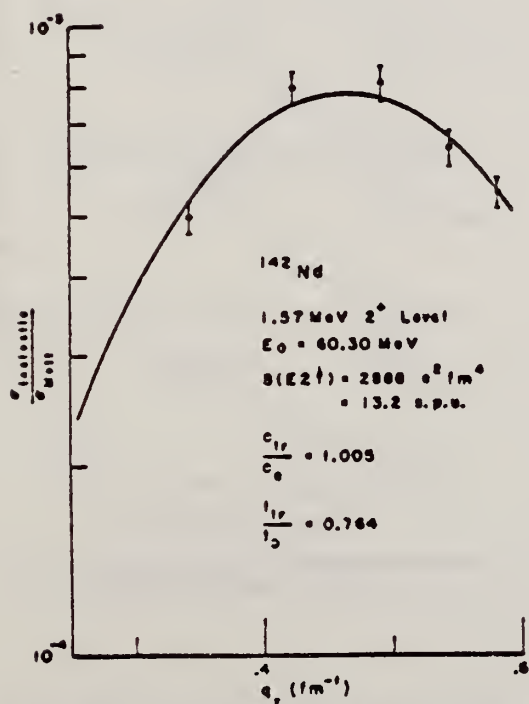
Fig. 14. Inelastic form factors for the 2 + level at 1.57 MeV in 142 Nd as a function of inelastic momentum transfer. The experimental points are the findings of this experiment and the solid line is the best fit obtained with the parameters shown.
