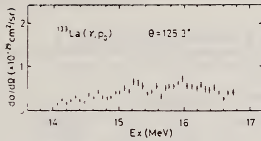
Fig 7 The ^{133}\text{La}(\gamma, p) cross section
