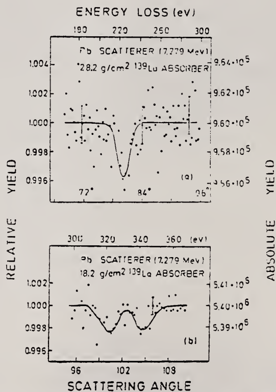
Fig. 3. (a) Portion of the normalized absorption spectrum obtained using a 28.2 \text{ g/cm}^2 thick La absorber. (b) Another portion of the spectrum obtained with a 18.2 \text{ g/cm}^2 thick absorber using higher statistics of \approx 5 \times 10^6 counts/channel.
