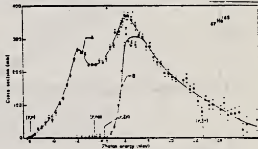
Fig. 4. Cross sections for Ho from neutron yield data. Curve A consists of \sigma(\gamma, n) + 2\sigma(\gamma, 2n) + \sigma(\gamma, np) + 3\sigma(\gamma, 3n) and was obtained from single-neutron counting data. Curve B consists of 2\sigma(\gamma, 2n) + \sigma(\gamma, 3n) , and was obtained from double-neutron counting data.
