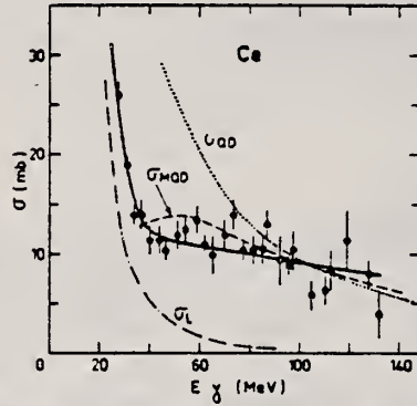
Fig. 15. Total photonuclear absorption cross sections \sigma(\text{tot}; E_\gamma) = \sigma^{(2)}(E_\gamma) from the present paper, represented by the experimental points and the corresponding full lines, are shown for Pb, Sn, Ce, Ta and U. These experimental results for photon energies E_\gamma between 20 and 140 MeV are compared with: (a) Lorentz line fits to the GDR data of the appropriate nucleus represented by the dot-dash \sigma_L(E_\gamma) plots. (b) Quasideuteron cross sections, \sigma_{OD}(E_\gamma) = (4.6NZ/A)\sigma_D(E_\gamma) for the appropriate nuclei, represented by the dotted \sigma_{OD}(E_\gamma) plots. Here \sigma_D(E_\gamma) is the photodisintegration cross section of deuterium. (c) Modified quasideuteron cross sections, \sigma_{ODM}(E_\gamma) = (8NZ/A)\sigma_D(E_\gamma) \exp(-D/E_\gamma) with D = 60 MeV, represented by the dashed \sigma_{ODM}(E_\gamma) plots. Pertinent GDR data for Pb, Sn, Ce, Ta and U were taken from refs. 5, 26-28 .
