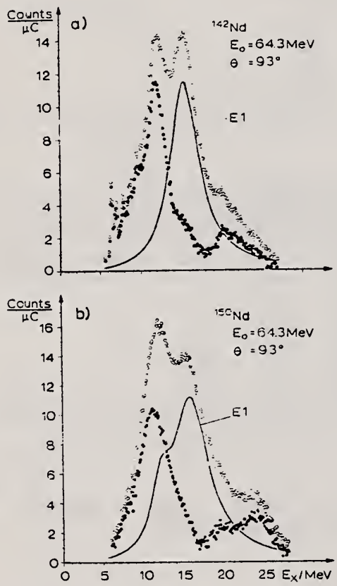
Fig. 1. Spectrum of inelastically scattered electrons after subtraction of radiation tail and background, a) 142 Nd, b) 150 Nd (open circles). Solid line: E1 cross section. Full circles: E1 cross section subtracted. The total number of counts/μC in the region of the giant resonances is about 100.
