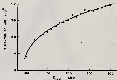
FIG. 2. Yield data from the production of ^{140}\text{Nd} in \text{Pr}_6\text{O}_{11} targets.
