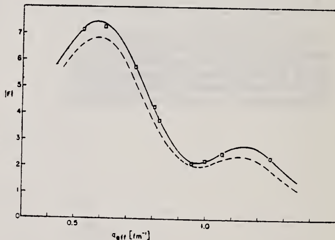
Fig. 3. Form factor for the 0-2^+ transition, F = \sqrt{\sigma/\sigma_{mott}} . The solid curve assumes \rho(r, \theta) = \bar{\rho} [1 + \exp \frac{r-R(\theta)}{t}]^{-1} and the skin thickness is constant. The dashed curve assumes \rho(r, \theta) = \bar{\rho} [1 + \exp \frac{\alpha-c}{t}]^{-1} with \alpha = r[1/(1 + \Sigma B_L Y_{L0}(\theta))] . In this last choice the skin thickness actually varies as the radius.
