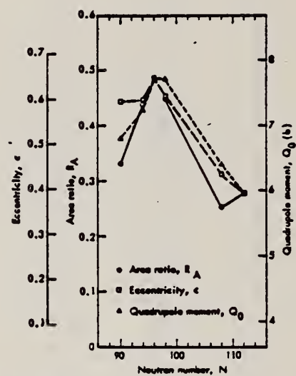
FIG. 9. The area ratio R_A , nuclear eccentricity e , and intrinsic quadrupole moment Q_0 plotted versus neutron number N . The data were scaled between the value for Gd 160 and that for W 184 . The absolute scale for Q_0 is based on a mean radius parameter R_0 = 1.26 F . The lines merely connect the three sets of data points. The experimental uncertainties have been omitted for clarity but are given in Tables VII and VIII; their average values are 0.065 (17%) for R_A , 0.010 (1.9%) for e , and 0.26b (3.7%) for Q_0 .
