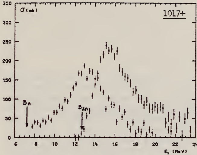
Fig. 6. Partial photoneutron cross sections [\sigma(\gamma, n) + \sigma(\gamma, pn)] and \sigma(\gamma, 2n) for ^{142}\text{Ce} . Arrows B_n and B_{2n} indicate theoretical threshold values for (\gamma, n) and (\gamma, 2n) reactions respectively. Data are not corrected for impurities.
