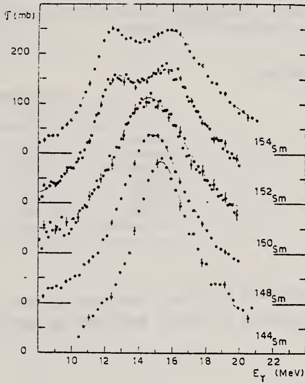
Fig. 7. Total photoneutron cross sections \sigma_T(E) of the doubly even samarium isotopes. Best single Lorentz line fits are shown for ^{144}\text{Sm} , ^{148}\text{Sm} and ^{150}\text{Sm} . For ^{152}\text{Sm} and ^{154}\text{Sm} the best two Lorentz line fits are presented. Corresponding Lorentz line parameters are given in table 2.
