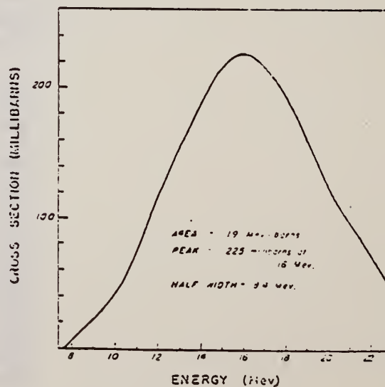
FIG. 3. ^{175}\text{Lu} cross section.
