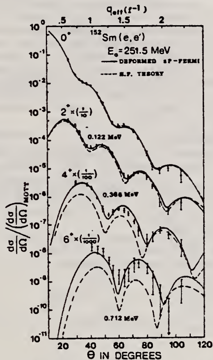
FIG. 1. Experimental values of \sigma/\sigma_{\text{Mott}} for the ground-state rotational band of ^{152}\text{Sm} , as a function of angle and q_{\text{eff}} = q(1 + \frac{1}{2}Z\alpha(r^2)^{-1/2}E^{-1}) . The solid lines are phenomenological fits (see text) and the dashed lines are the results of the use of HF wave functions.
