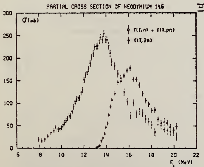
Fig. 6. Partial photonuclear cross sections \sigma(\gamma, n) and \sigma(\gamma, 2n) of 146 Nd.
