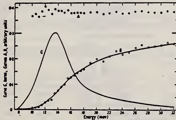
Figure 6. A, the ratio of activation curves ^{160}Gd(\gamma, n)/^{181}Ta(\gamma, n) ; B, activation curve for ^{160}Gd(\gamma, n) ; C, derived cross section: ^{160}Gd(\gamma, n) .
