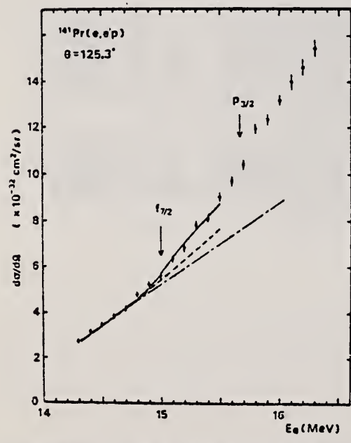
Fig. 3. The differential cross section of the ^{141}\text{Pr}(e, e'p) reaction for \theta = 125.3^\circ (see caption to fig. 2).
