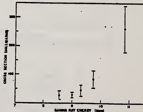
FIG. 5. Cross section vs energy, Ho 165 ( \gamma, n )Ho 164 (34 min).
